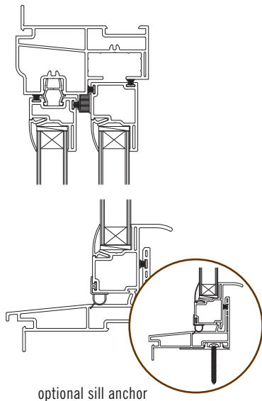
StyleView Single-Hung with Flange
