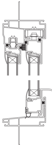
StyleView NT Single-Hung
