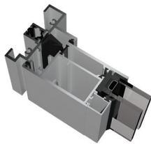
Window Wall Frame for YWW 45 TU
