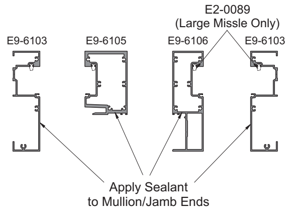
Detail 15 OXO Frame
