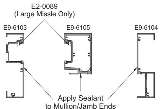
Detail 14 OX Frame
