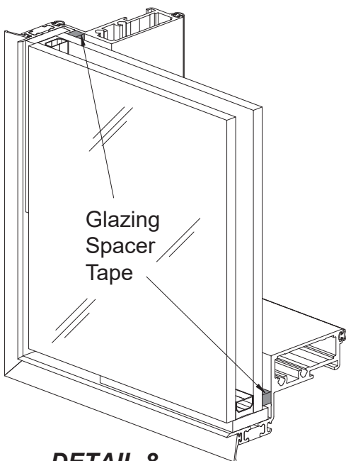
DETAIL 8
