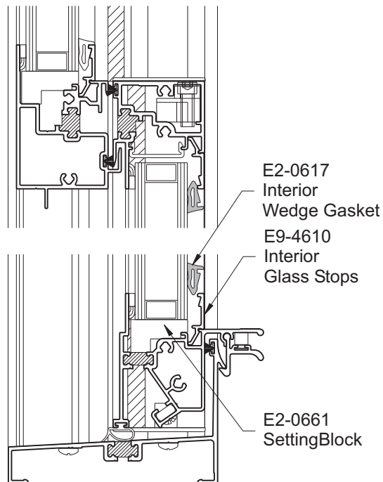
DETAIL 13
