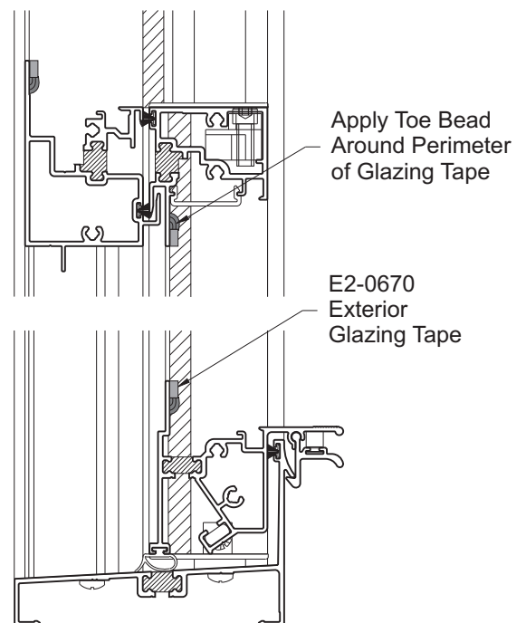
DETAIL 12
