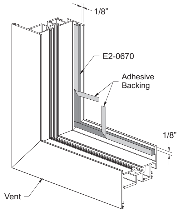
DETAIL 9
