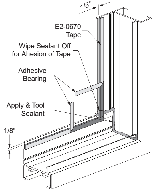
DETAIL 7
