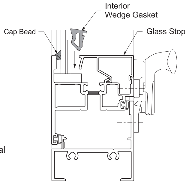
DETAIL 13
