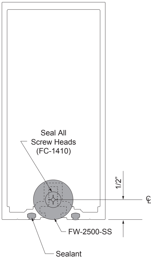
Detail 14 5-1/4" Back Depth Mullion Shown, Others Similar
