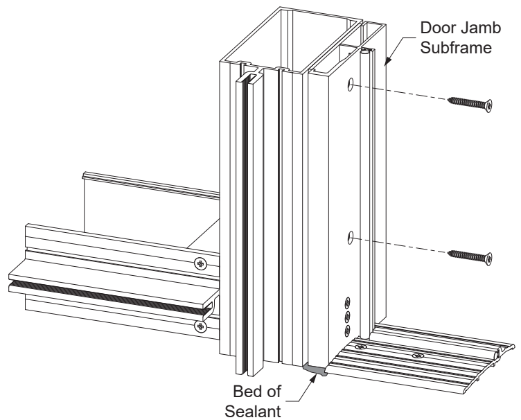
Detail 34 Air-resistant Threshold Shown
