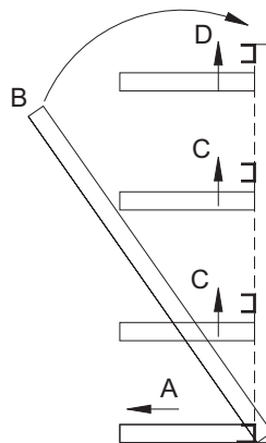
DETAIL 28 Insulating Glazing Shown Single Glazing Similar
