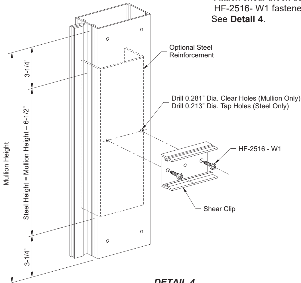
DETAIL 4 Insulating Glazing Shown Single Glazing Similar
