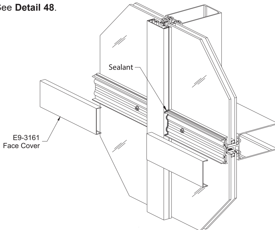
DETAIL 48 Insulating Glazing Shown Single Glazing Similar
