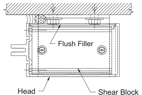
DETAIL 29 Single Glazing Shown Insulating Glazing Similar
