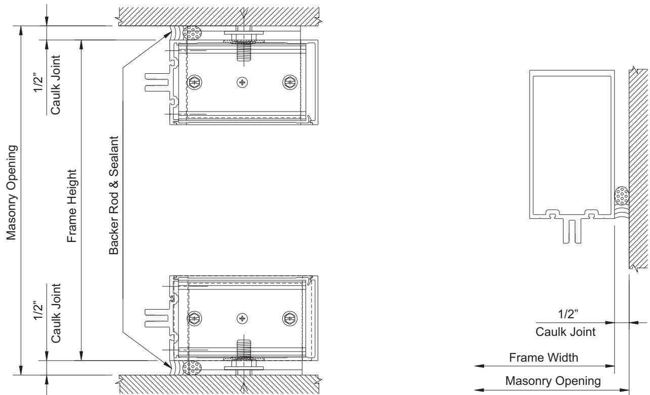
DETAIL 35 Single Glazing Shown Insulating Glazing Similar
