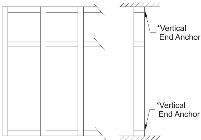
SINGLE SPAN
