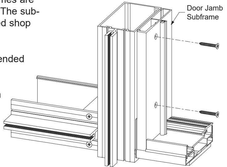
Detail 32 Water-resistant Threshold Shown
