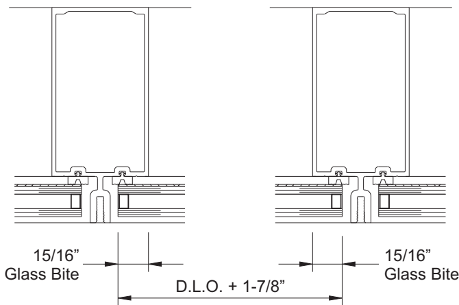
DETAIL 45 Insulating Glazing Shown Single Glazing Similar
