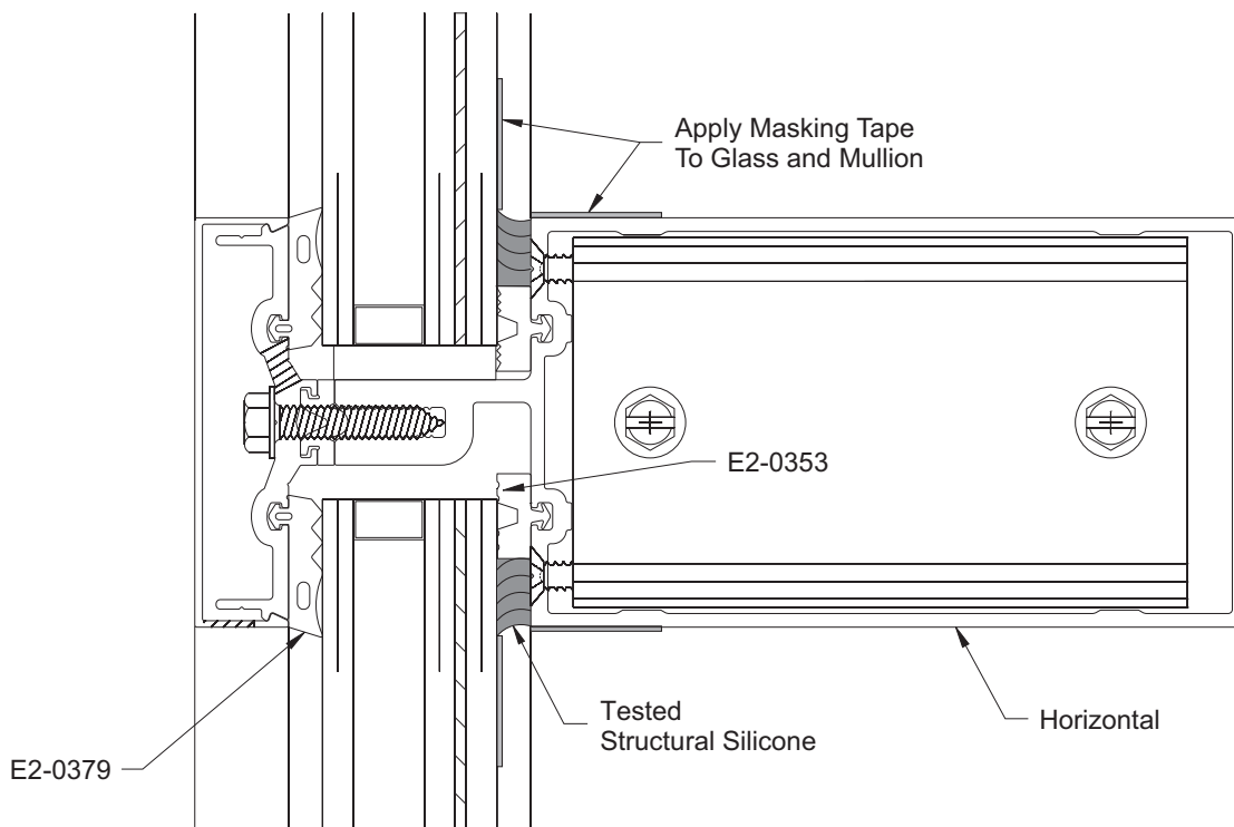
DETAIL 49 Insulating Glazing Shown Single Glazing Similar
