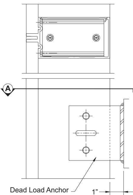
DETAIL 24 Single Glazing Shown Insulating Glazing Similar
