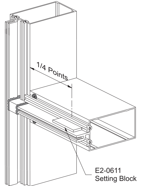
DETAIL 44 Insulating Glazing Shown Single Glazing Similar
