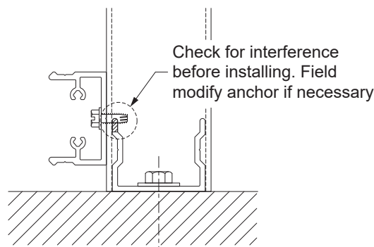
Detail 30 For Exposed Fasteners Shear Block Used as Anchor
