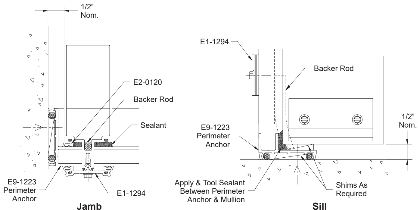
Detail 25 E9-1223 Shown Others Similar
