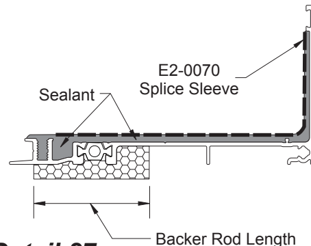
Detail 27
