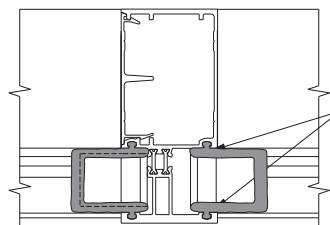
Seal Ramp of Deflector to the Pocket Wall
