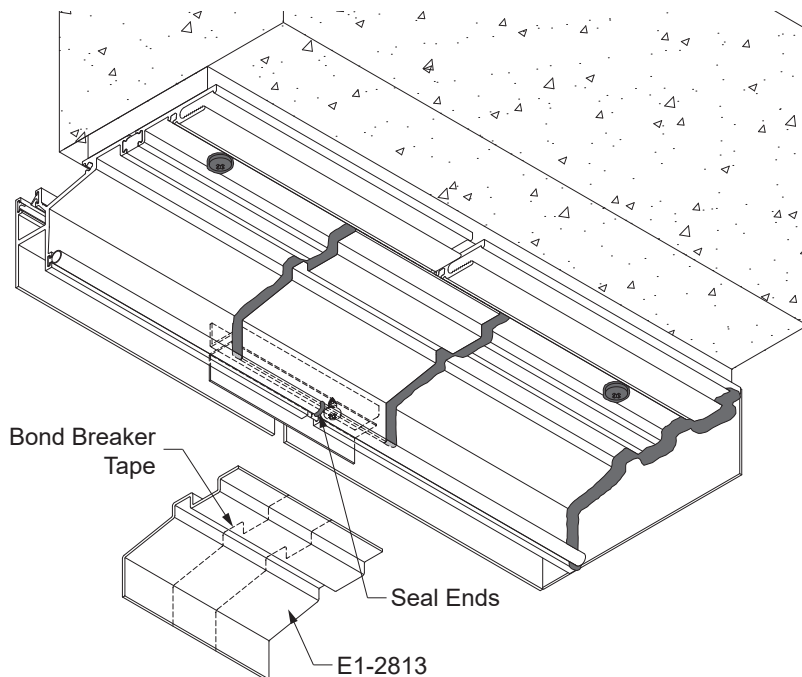
Detail 35
