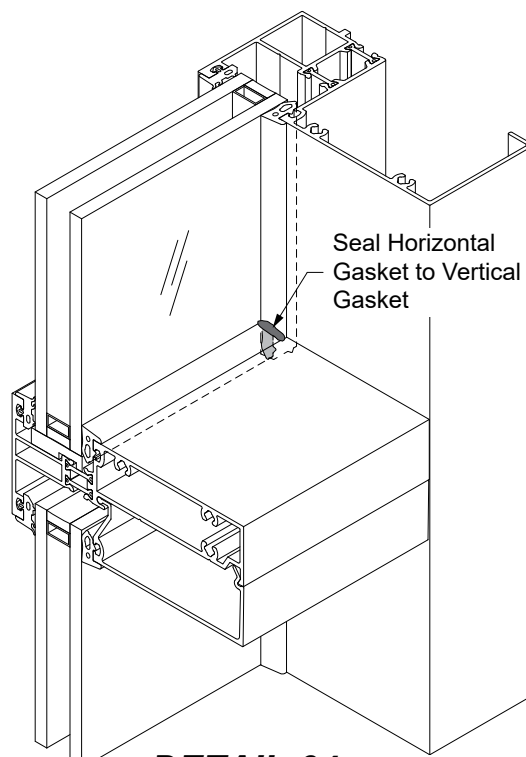
DETAIL 64 Inside Glazing
