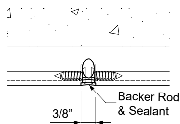
DETAIL 52A (WITH SLAB EDGE COVER)
