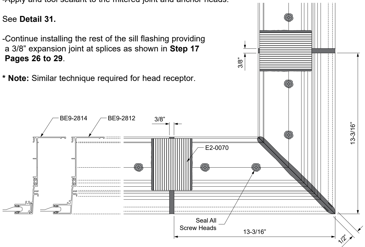
Detail 31 90° Outside Corner Shown Others Similar
