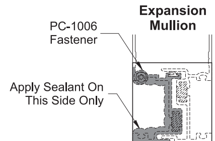
DETAIL 18
