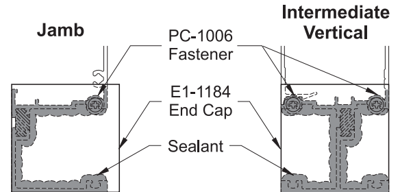
DETAIL 18
