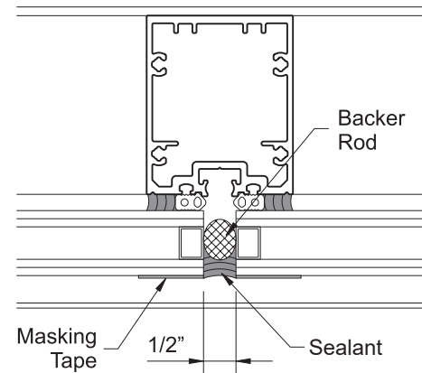
DETAIL 62
