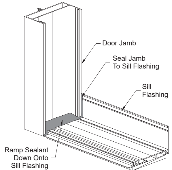
DETAIL 66
