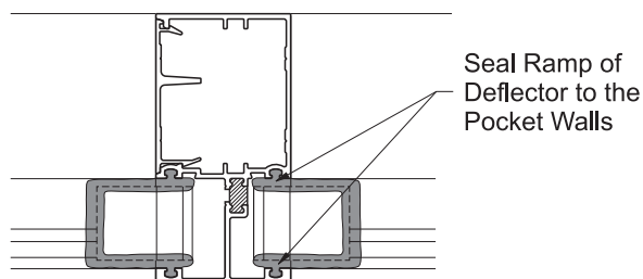
DETAIL 46a
