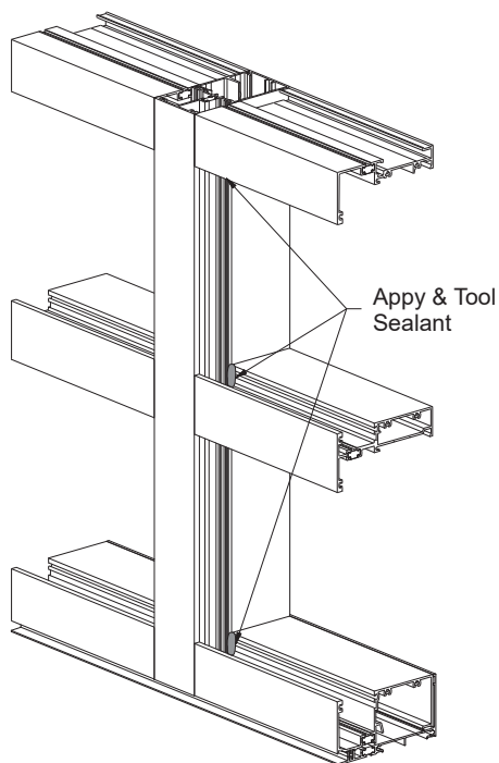
VERTICAL THROUGH
