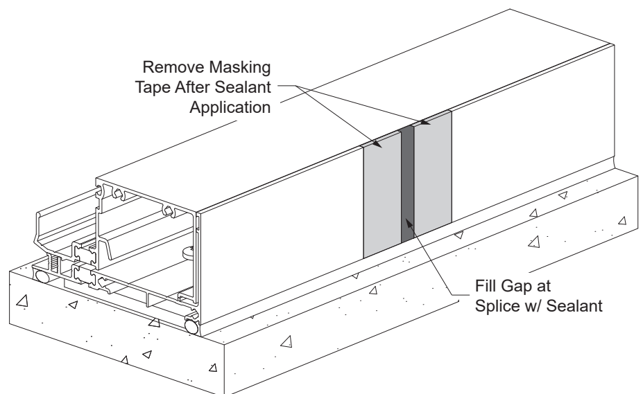
DETAIL 45
