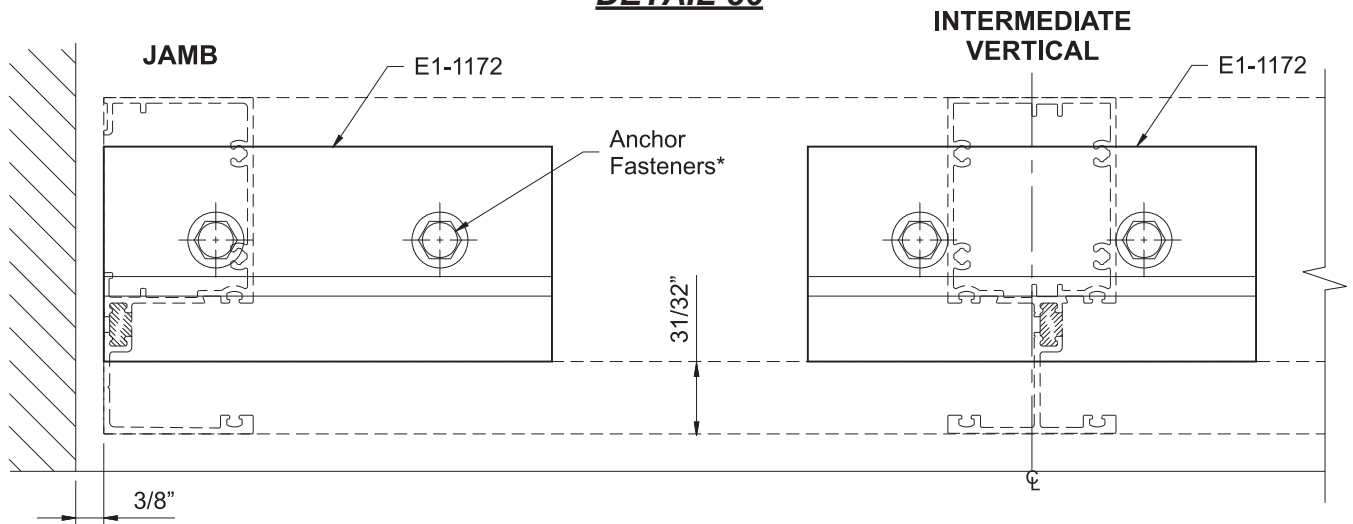
DETAIL 36
