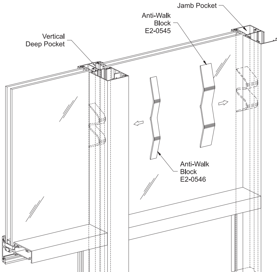
DETAIL 53
