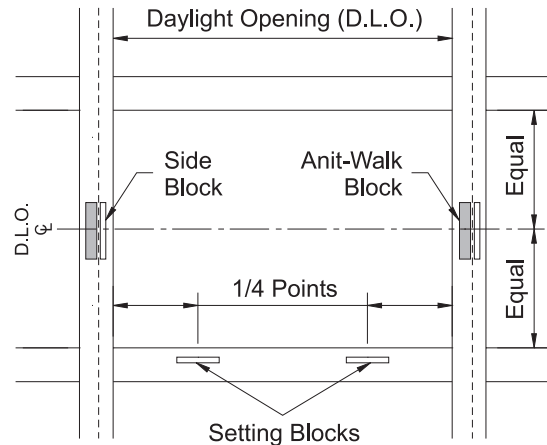
DETAIL 53
