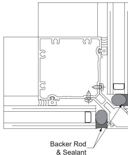
Detail 65
