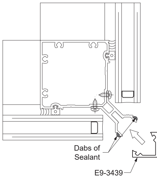
Detail 64
