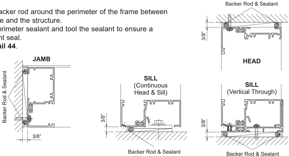
DETAIL 44
