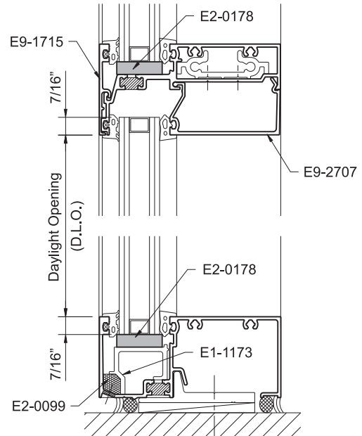
DETAIL 57
