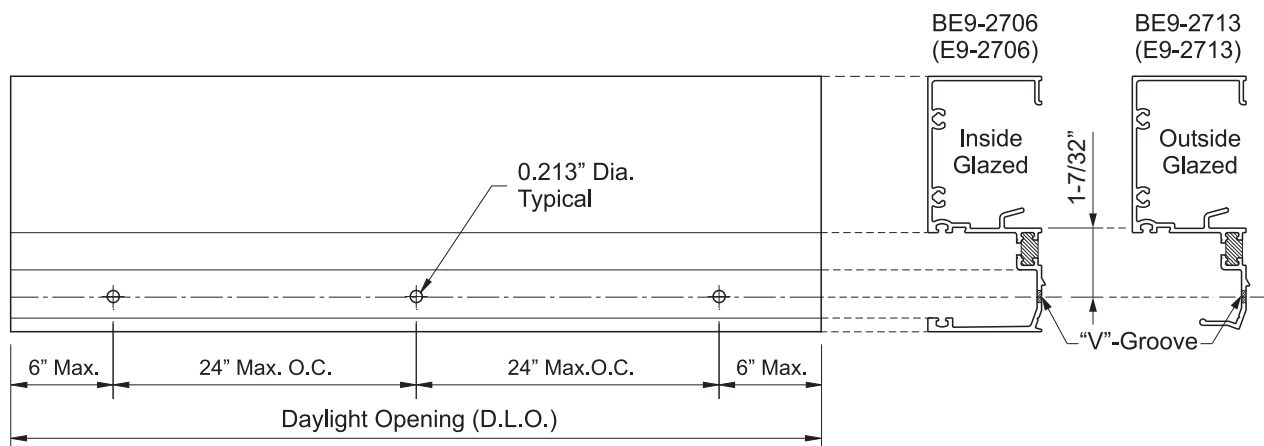
DETAIL 4
