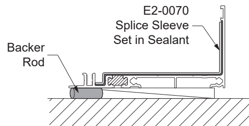
Detail 27
