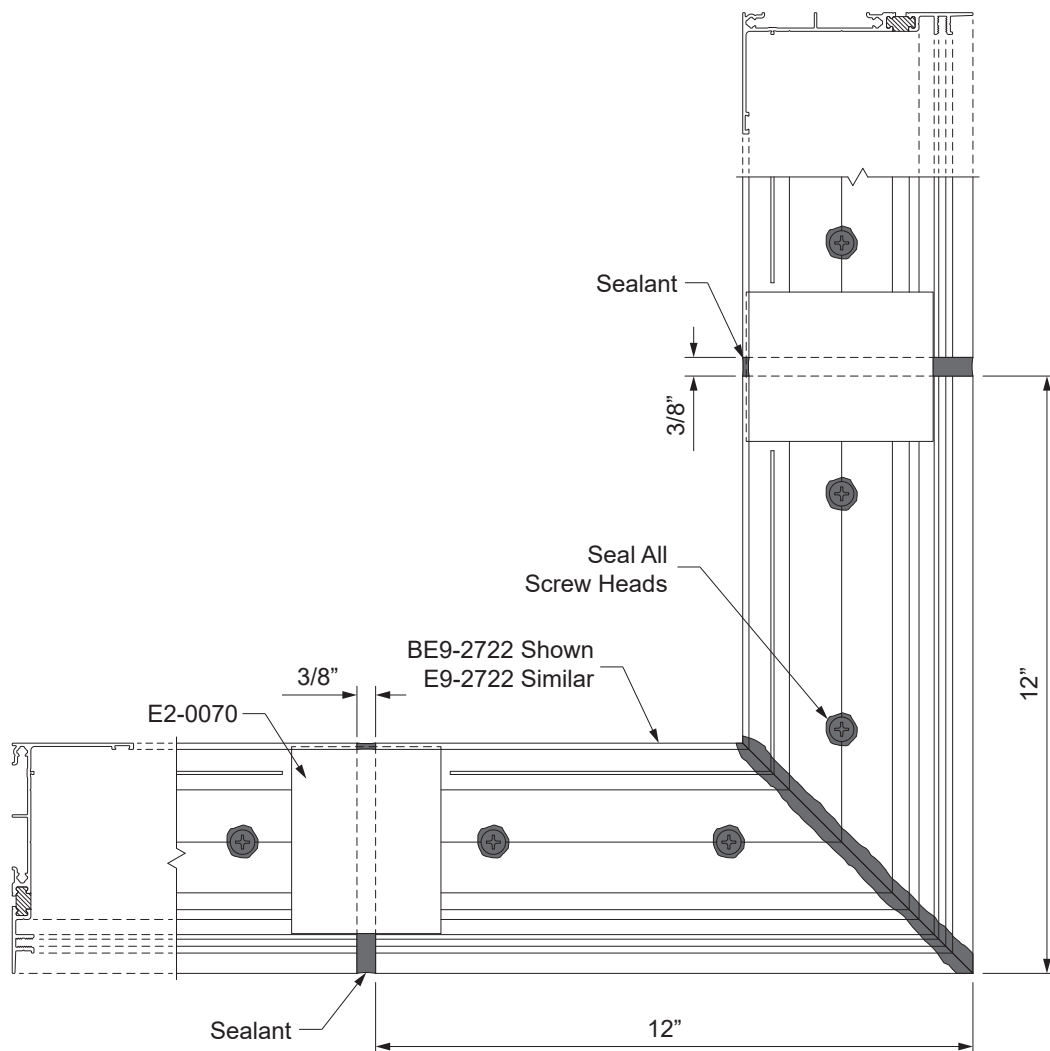
Detail 30
