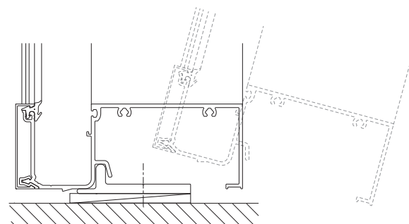
DETAIL 31
