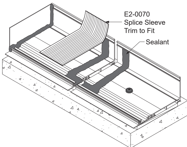
DETAIL 22
