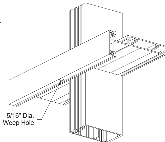
DETAIL 36 Intermediate Horizontal Shown Head Similar
