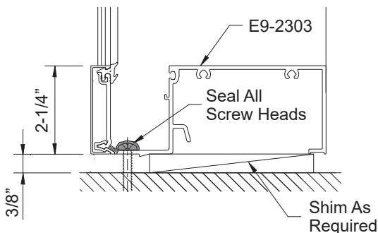
DETAIL 27
