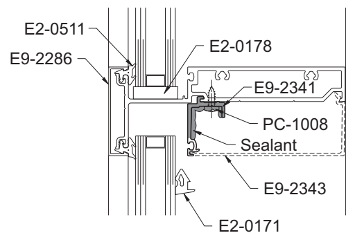
DETAIL 45
