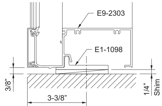
DETAIL 28
