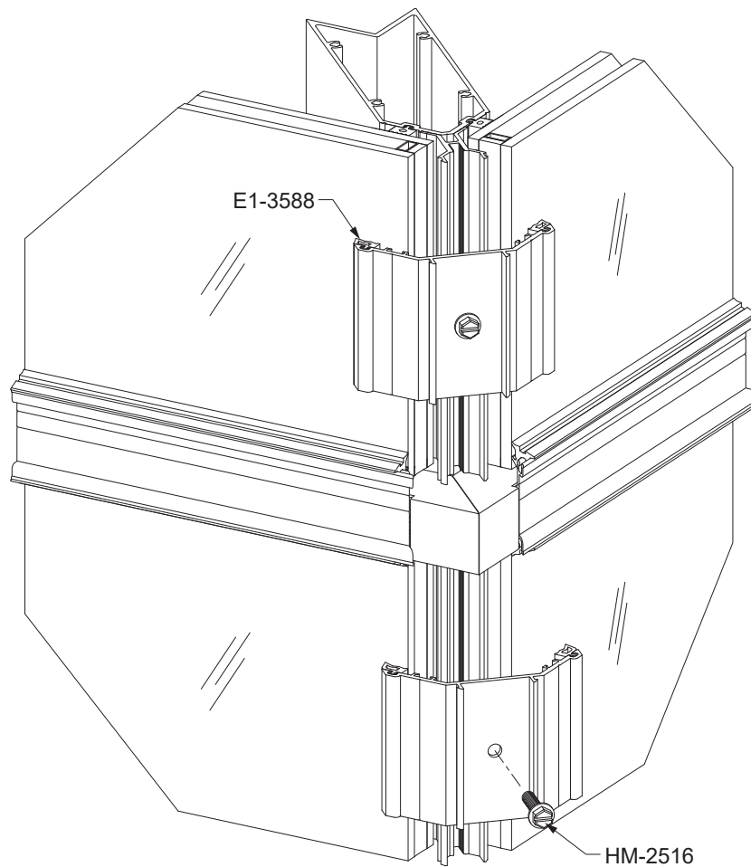
DETAIL 10C
