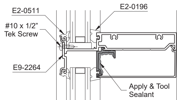
Detail 50
