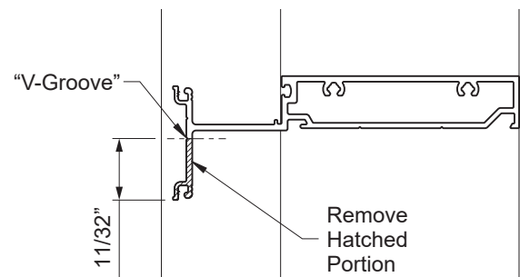
Detail 49
