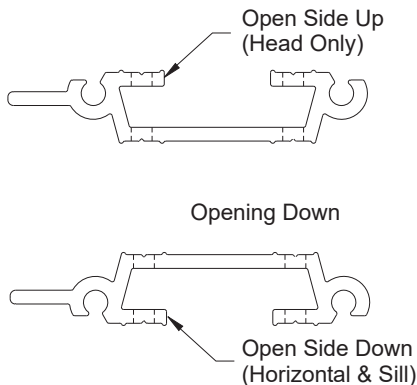
DETAIL 2D
