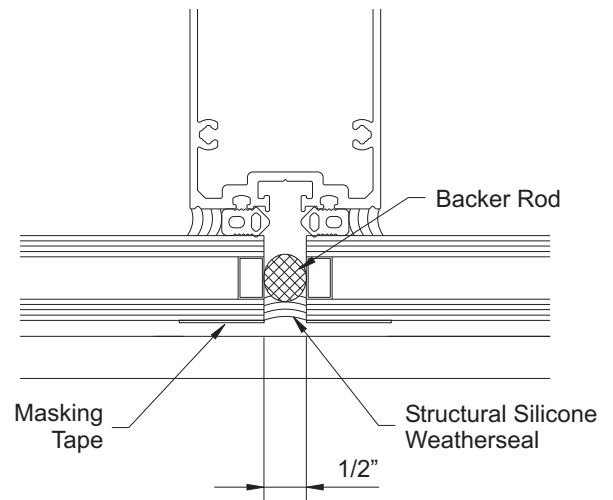
DETAIL 48
