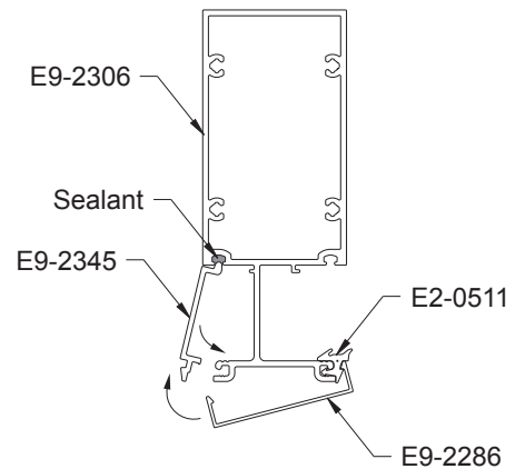
DETAIL 9D
