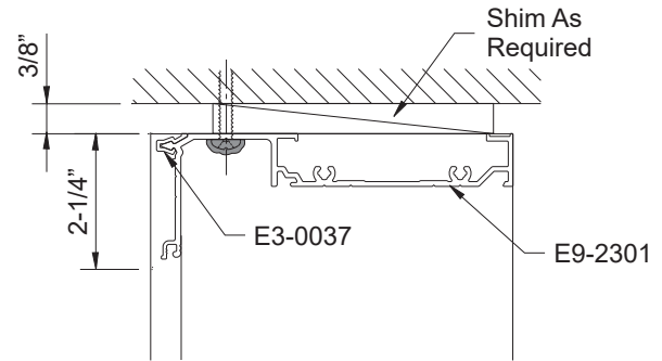
DETAIL 26
