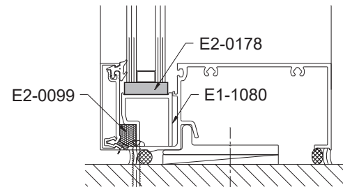
DETAIL 41
