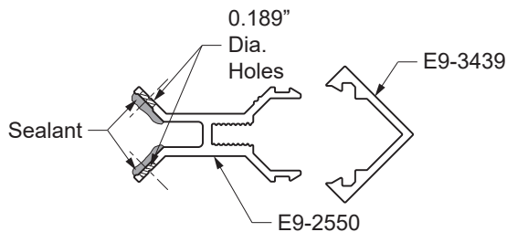
DETAIL 8C
