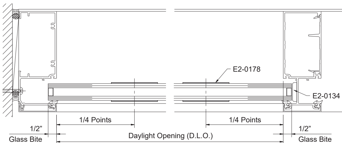
DETAIL 41
