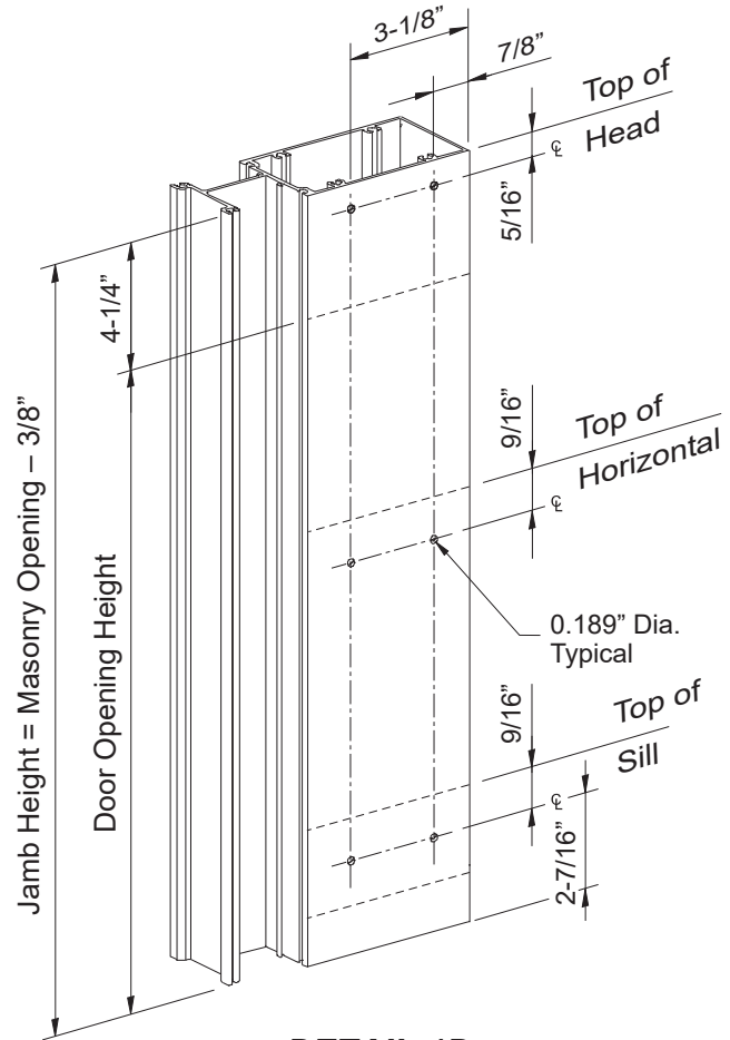
DETAIL 1D
