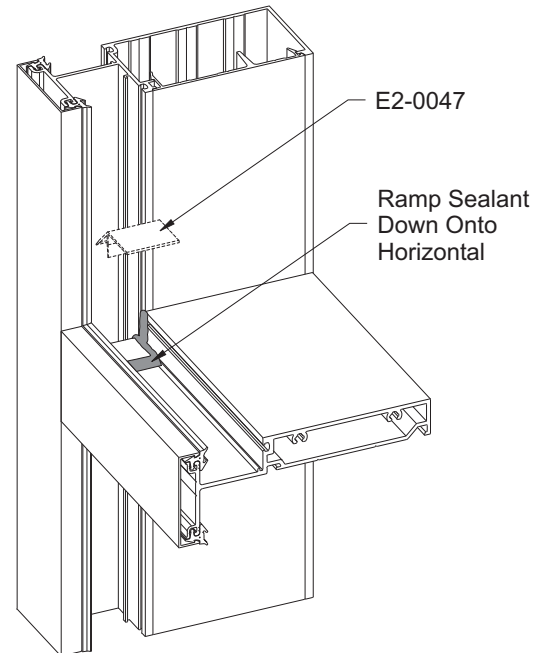
DETAIL 33
