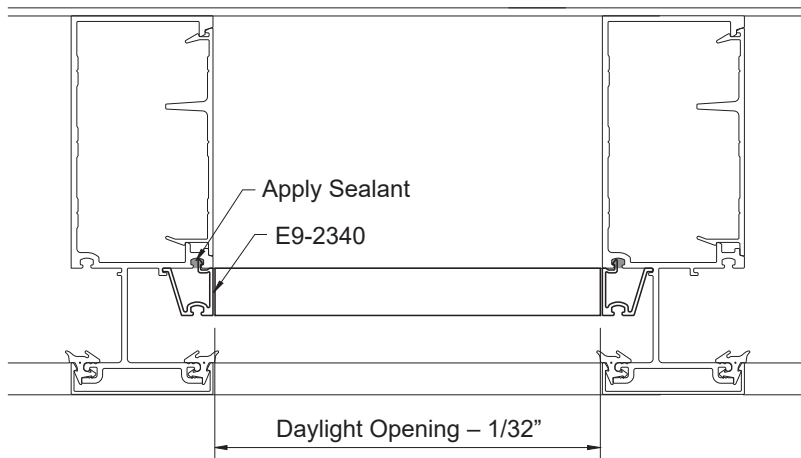
DETAIL 38
