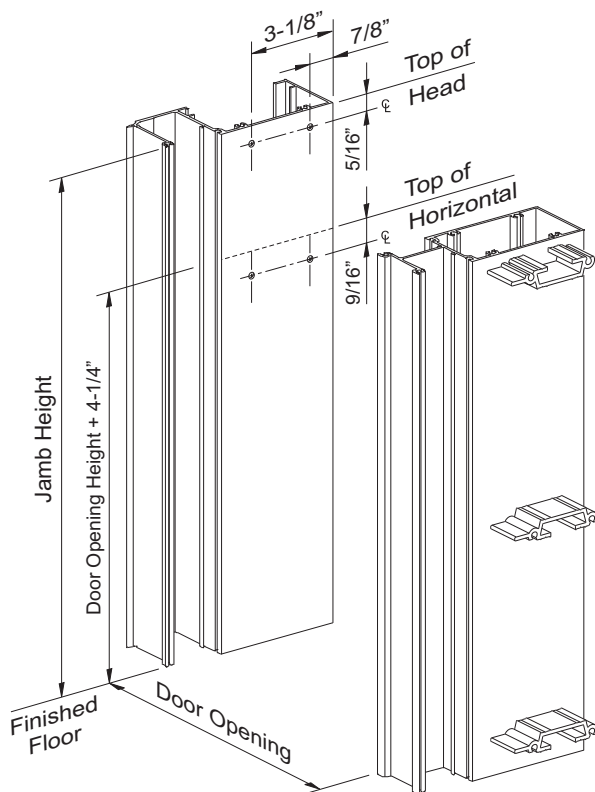
DETAIL 4D
