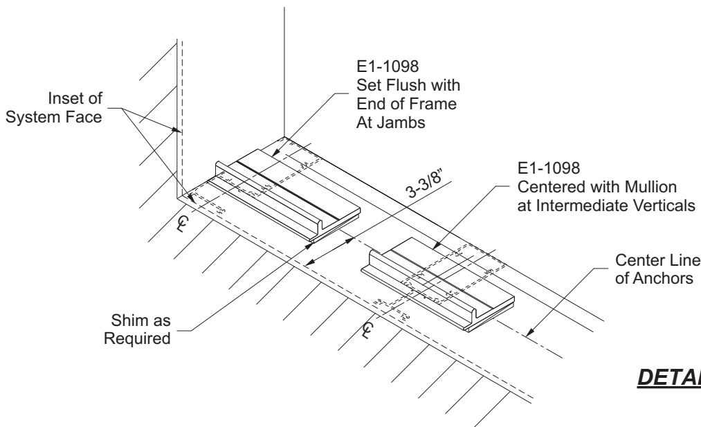
DETAIL 28
