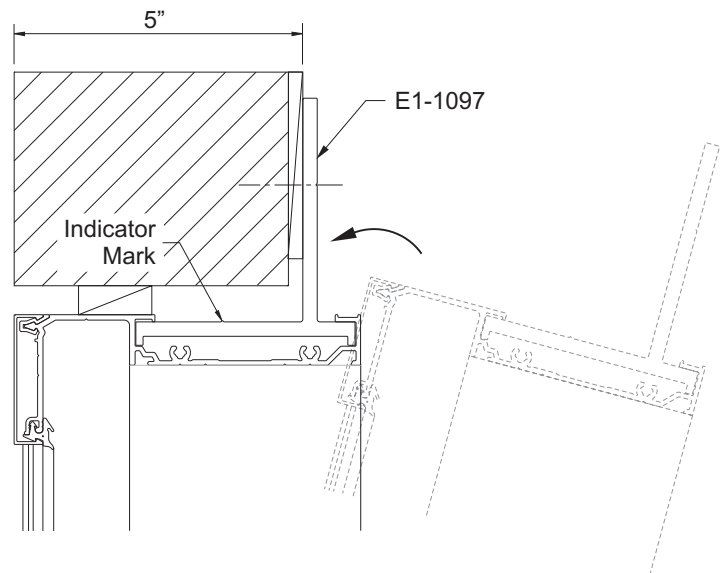
DETAIL 31
