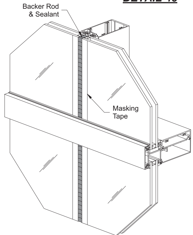
DETAIL 48
