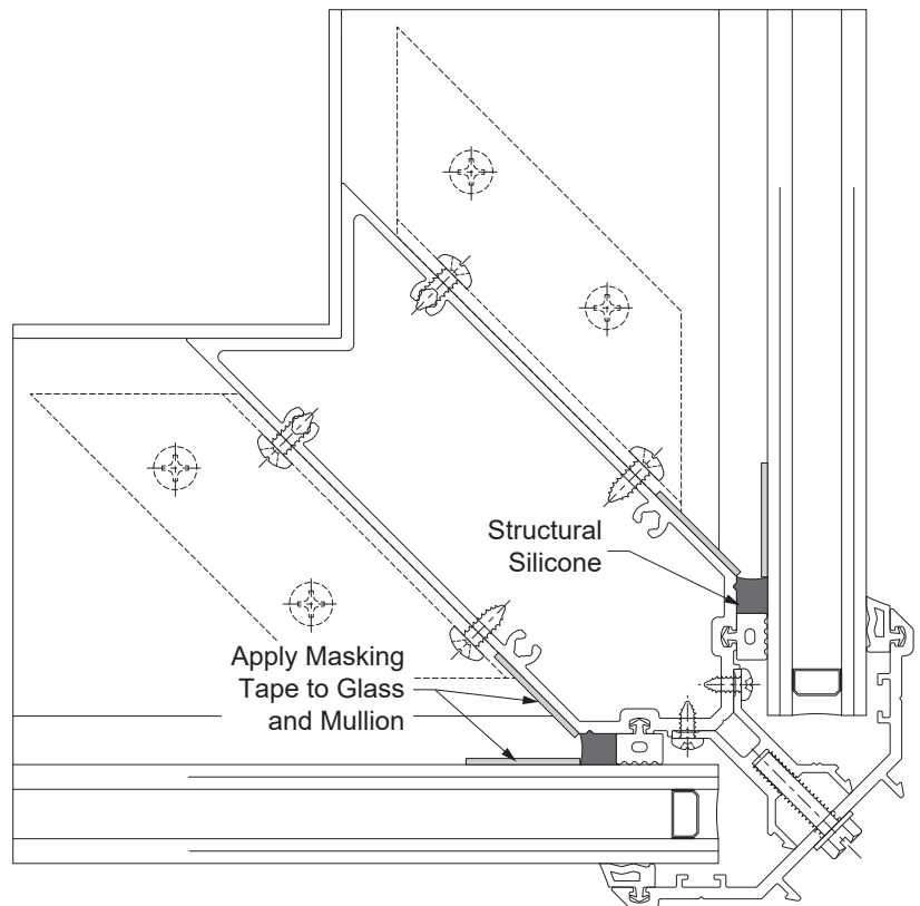
DETAIL 11C
