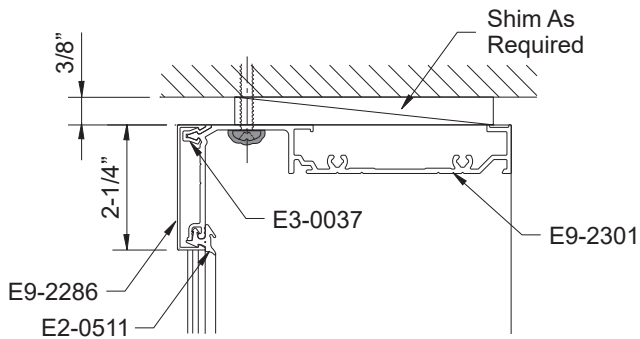
DETAIL 27
