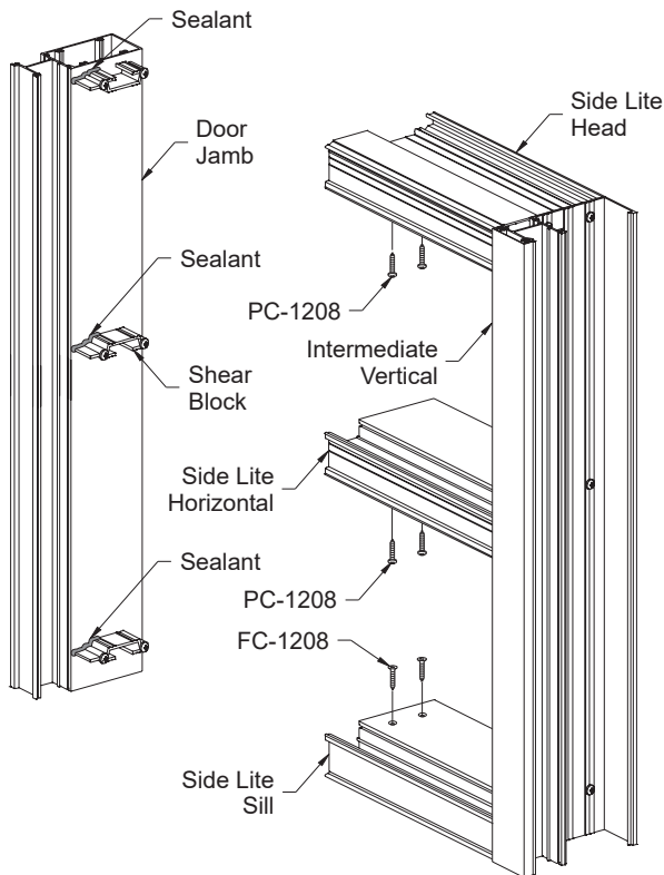
DETAIL 8D
