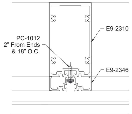
DETAIL 40
