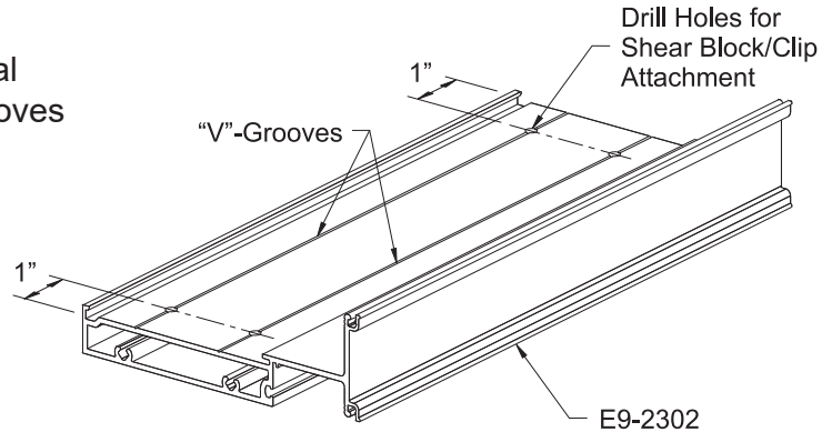
DETAIL 7
