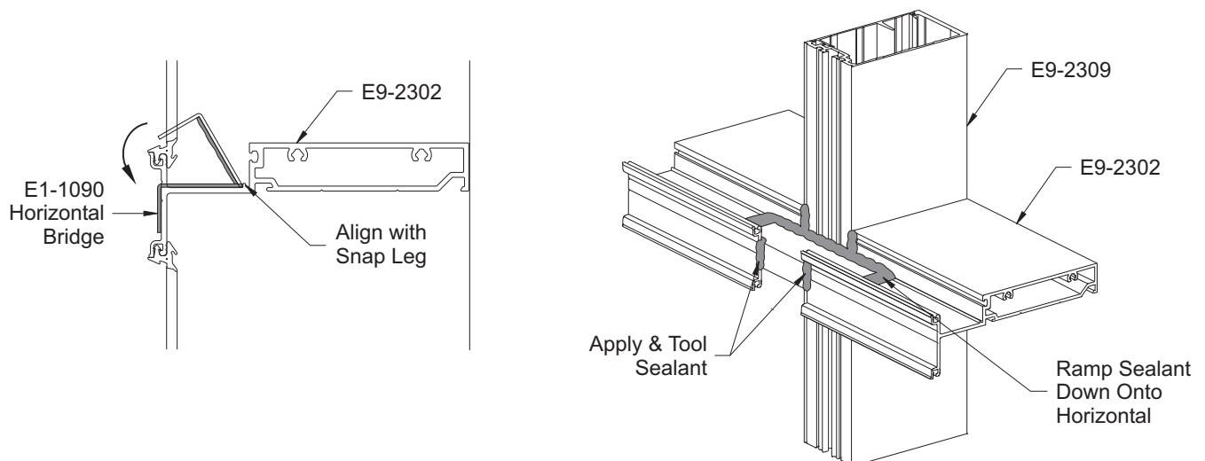
DETAIL 34
