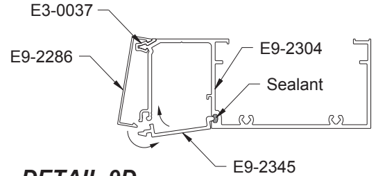
DETAIL 9D
