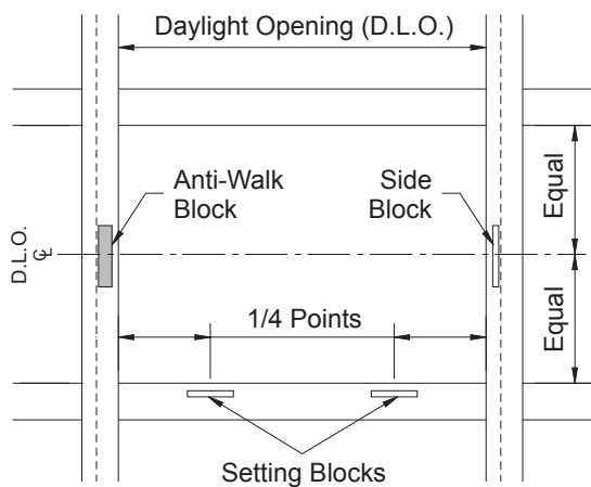
DETAIL 42
