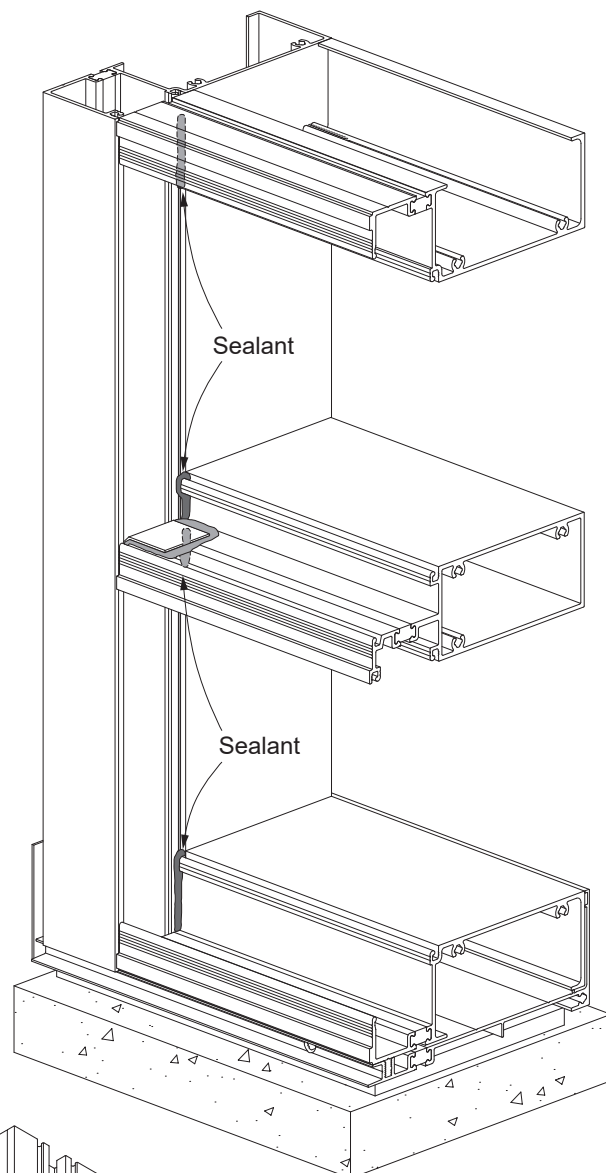
Detail 51 Jamb Mullion Shown, Captured Corner Mullion Similar
