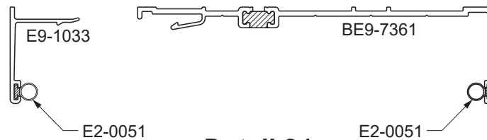
Detail 21
