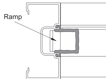
Detail 17 1" Glazing Shown 1/4" Glazing Similar
