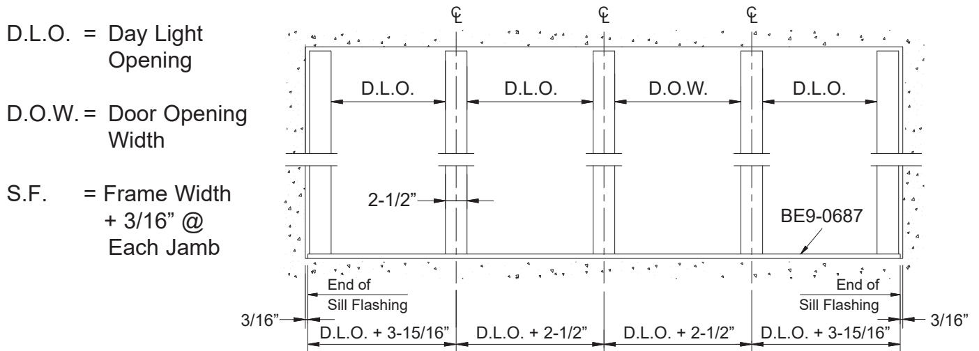
Entrance Door with Water Resistant Threshold, E9-0502
