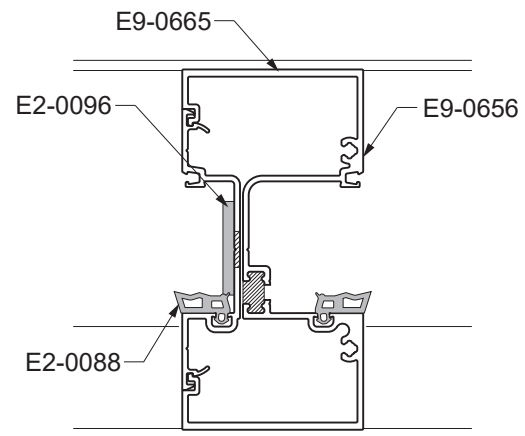
Detail 34A Inside Glazing
