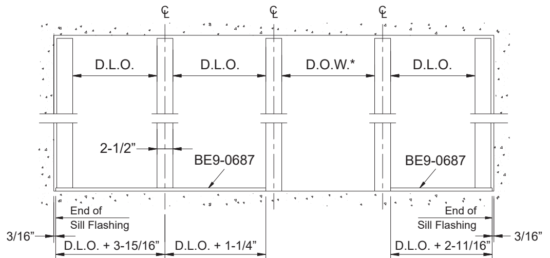
Entrance Door with Air Tight Threshold, E9-0487
