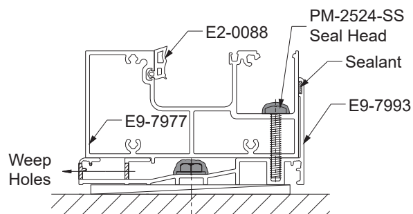
Detail 26B Inside Glazing
