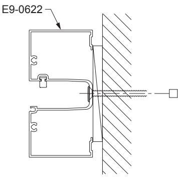
Jamb ± 50 PSF
