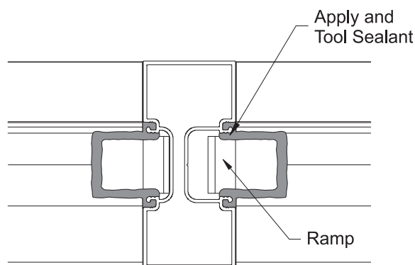
Detail 26 1" Glazing Shown 1/4" Glazing Similar
