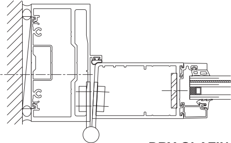
DRY GLAZING
