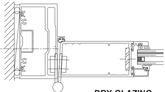
DRY GLAZING
