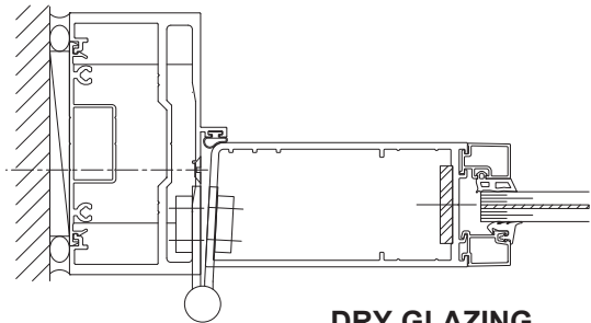
DRY GLAZING
