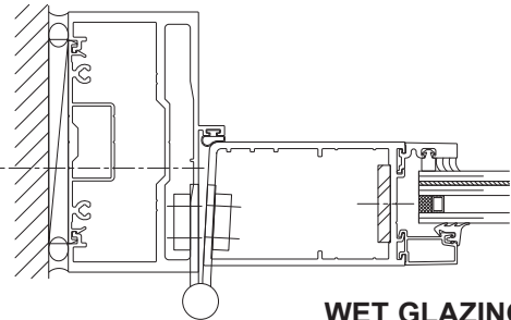
WET GLAZING
