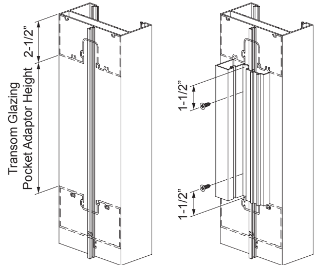
DETAIL 1
