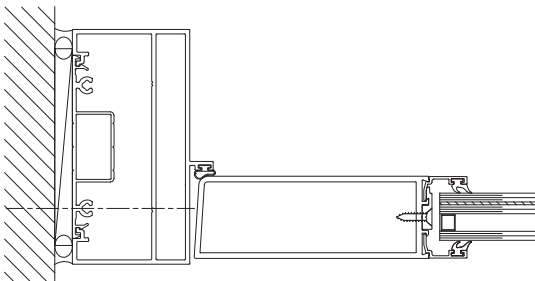
1" Glazing
