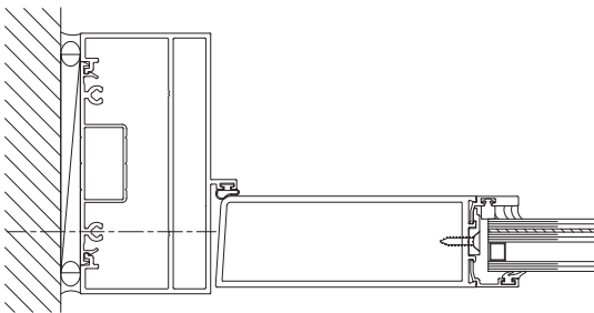
1" Glazing
