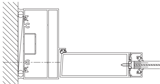
9/16" Glazing
