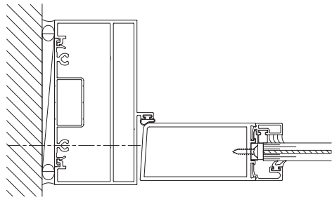
9/16" Glazing
