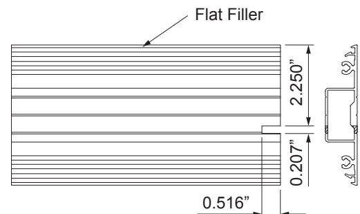
DETAIL 3
