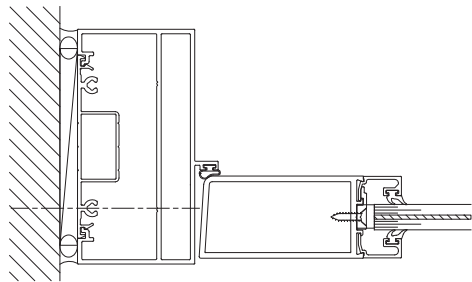
9/16" Glazing
