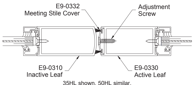
DETAIL 14
