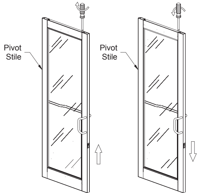
DETAIL 12
