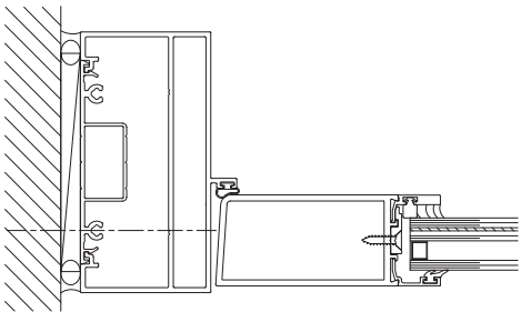
1" Glazing
