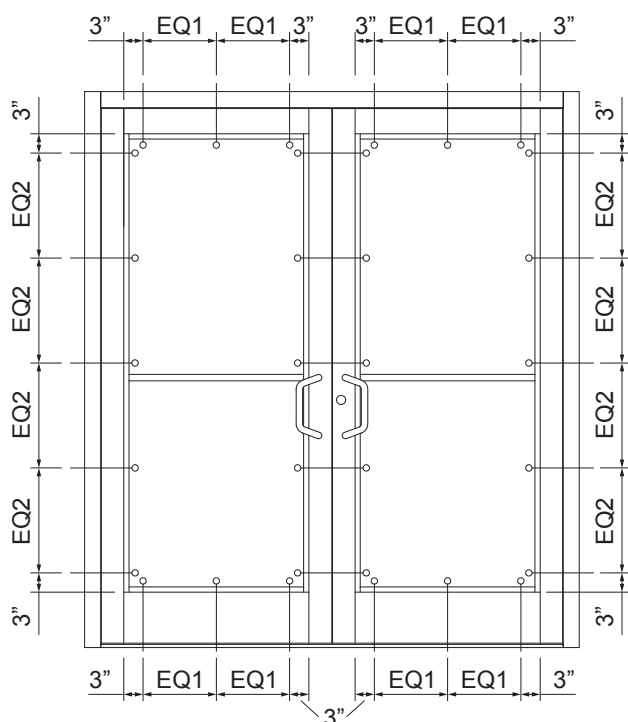
DETAIL 10
