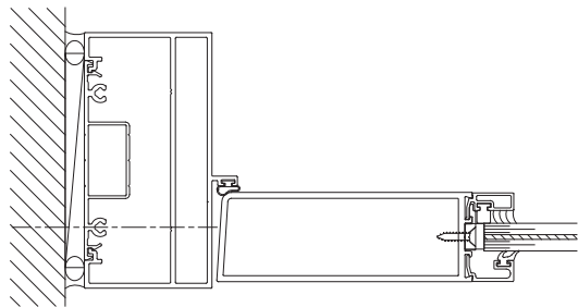
9/16" Glazing
