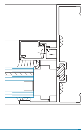
SECTION 3 Opp.
