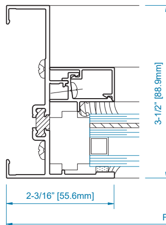
SECTION 3
