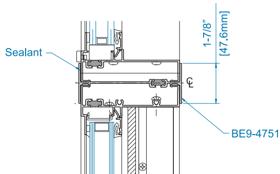
SECTION 38 HORIZONTAL STACKING MULLION
