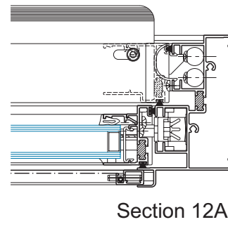
Spiral Balance Shown 4 Pieces/Vent Location
