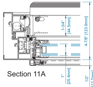
Spiral Balance Shown 2 Pieces/Vent Location
