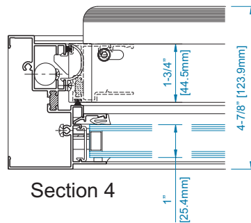
Spiral Balance Shown 2 Pieces/Vent Location
