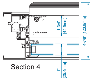
Spiral Balance Shown 2 Pieces/Vent Location
