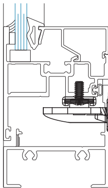
SECTION 2 w/ Butt Hinge
