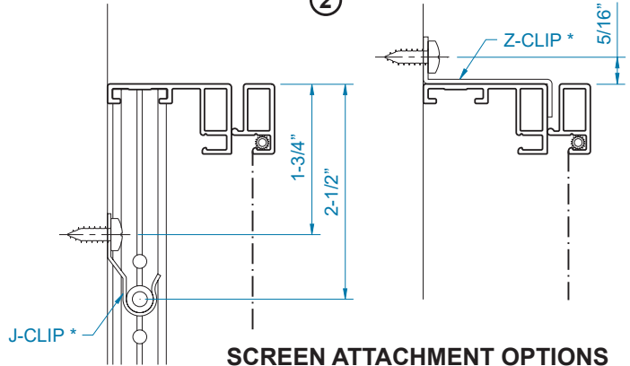
SCREEN ATTACHMENT OPTIONS
