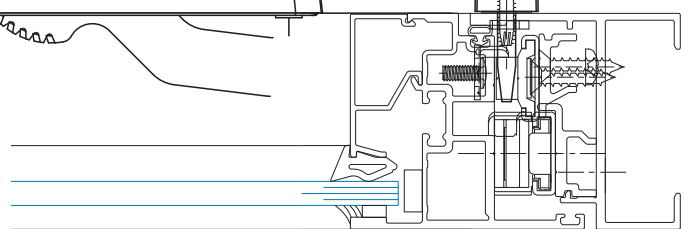
SECTION 4 w/ 4-Bar Hinge
