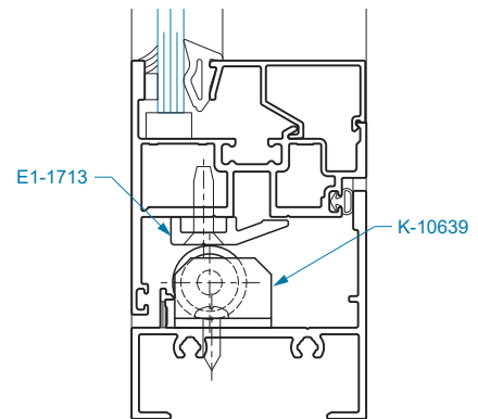
SECTION 2A At Roller Guide
