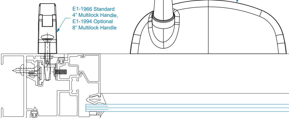
SECTION 3 w/ 4-Bar Hinge
