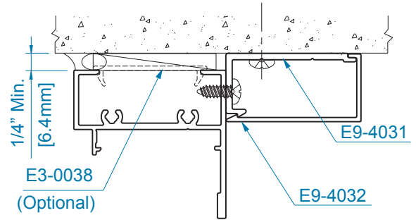
Head With 1" x 2" Trim & Clip (Jamb Similar)
