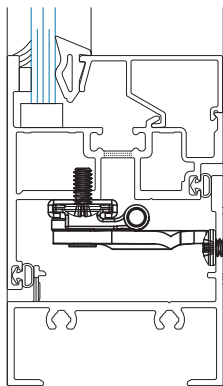
SECTION 2 w/ 4-Bar Hinge
