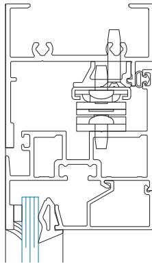
SECTION 1A Head w/ Butt Hinge
