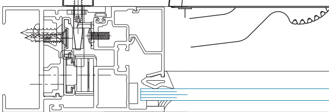
SECTION 3 w/ 4-Bar Hinge
