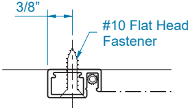
ANCHOR SCREW
