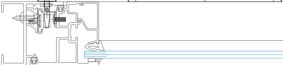
SECTION 3 w/ Butt Hinge
