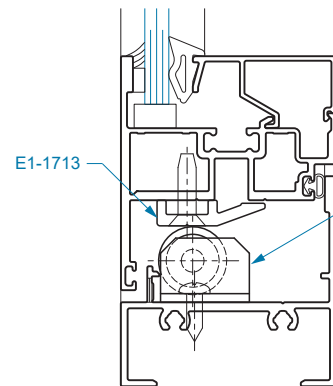
SECTION 2A At Roller Guide
