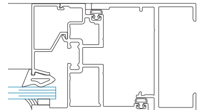
SECTION 4 w/ 4-Bar Hinge
