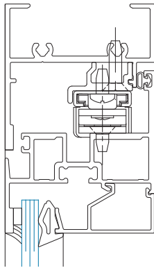
SECTION 1 Head w/ 4-Bar Hinge
