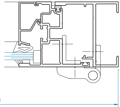
SECTION 9 w/ Optional Butt Hinge
