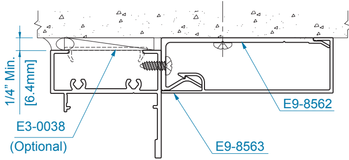
Head With 1-1/8" x 3-1/2" Trim & Clip (Jamb Similar)
