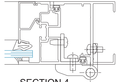
SECTION 4 w/ Butt Hinge
