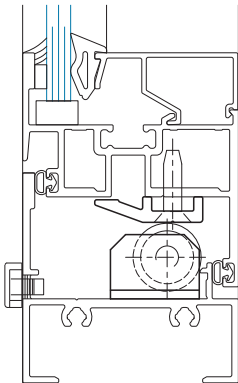
SECTION 2 Sill for 4-Bar & Butt Hinges
