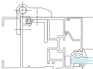
SECTION 3A w/ Butt Hinge
