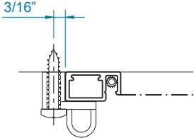
WING CLIP
