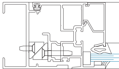
SECTION 3 w/ 4-Bar Hinge
