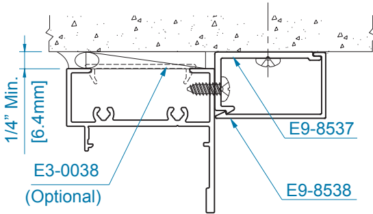
Head With 1" x 1-11/16" Trim & Clip (Jamb Similar)
