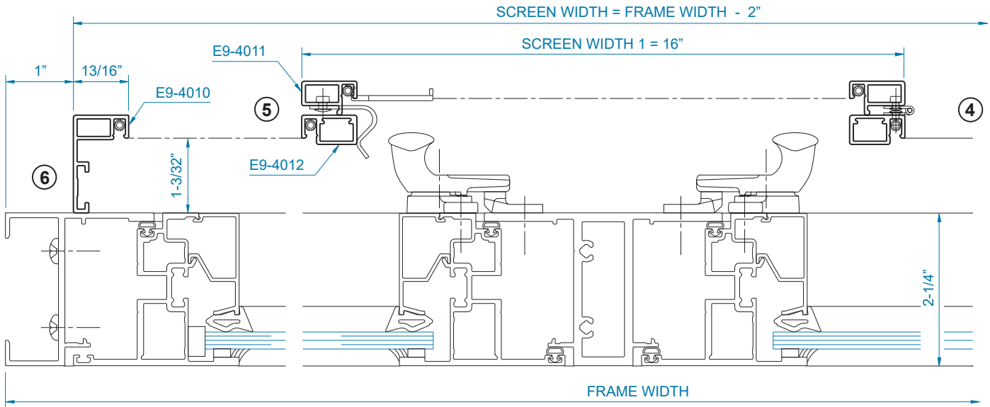
SCREEN ATTACHMENT OPTIONS
