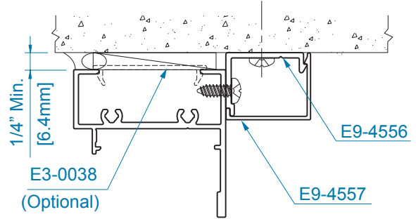
Head With 1" x 1-1/4" Trim & Clip (Jamb Similar)
