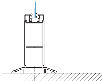
SECTION 8 BOTTOM RAIL
