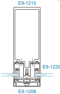
SECTION 5 HEAVY DUTY VERTICAL (1/4" Gl.)
