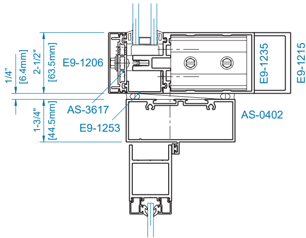
SECTION 7 TRANSOM BAR
