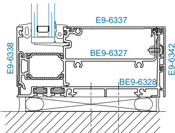
SECTION 8 O.G. SILL
