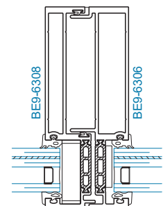
SECTION 60A OPTIONAL O.G. CAPTURED MULLION
