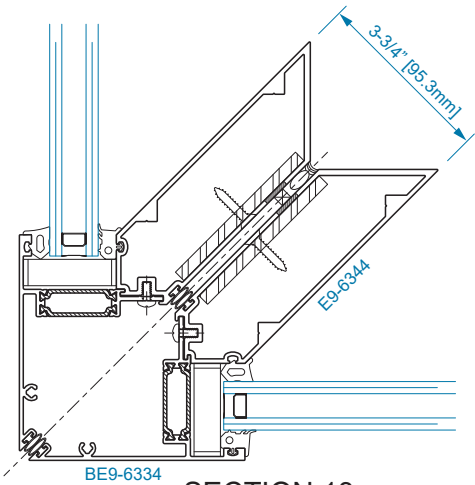
SECTION 13 90° O.S. CORNER CAPTURED MULLION
