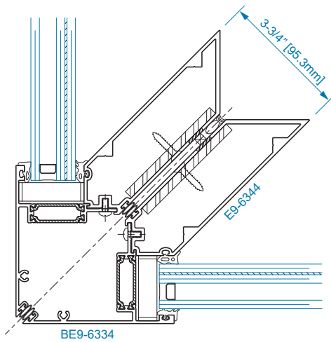
SECTION 63 90° O.S. CORNER CAPTURED MULLION
