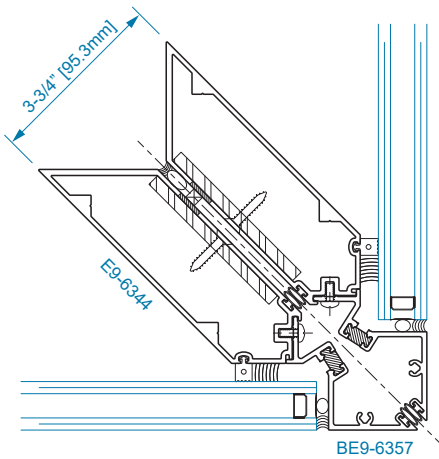
SECTION 13A 90° O.S. CORNER SSG MULLION
