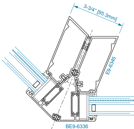
SECTION 64 135° O.S. CORNER CAPTURED MULLION
