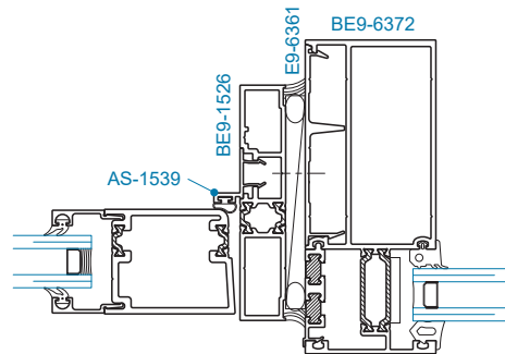
SECTION 37T DOOR JAMB w/ SIDELITE
