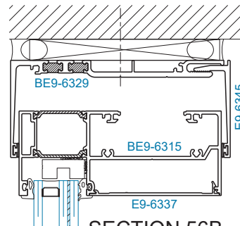
SECTION 56B O.G. HEAD W/ RECEPTOR
