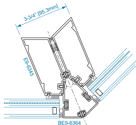
SECTION 64A 135° O.S. CORNER SSG MULLION
