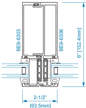
SECTION 10 O.G. CAPTURED MULLION
