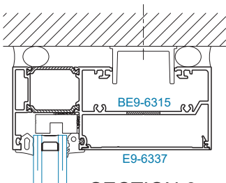
SECTION 6 O.G. HEAD
