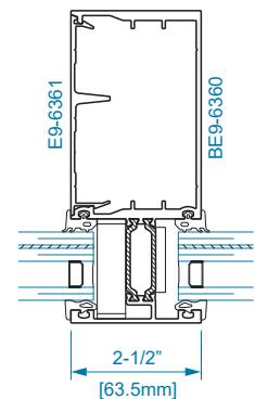
SECTION 60B FIELD GLAZED O.G. CAPTURED TUBULAR MULLION
