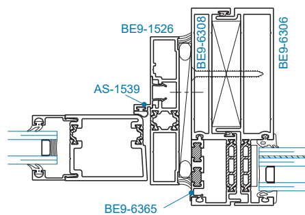
SECTION 80T DOOR JAMB w/ SIDELITE
