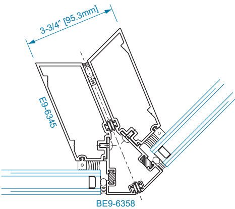
SECTION 14A 135° O.S. CORNER SSG MULLION
