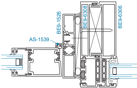
SECTION 24T DOOR JAMB w/ SIDELITE
