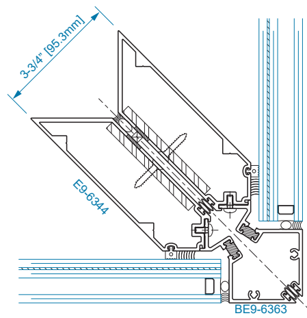
SECTION 63A 90° O.S. CORNER SSG MULLION
