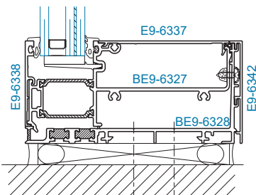
SECTION 58 O.G. SILL
