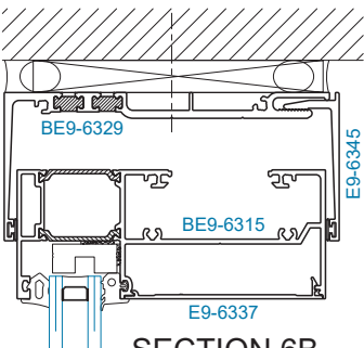
SECTION 6B O.G. HEAD W/ RECEPTOR
