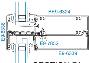
SECTION 7A OPTIONAL O.G. HORIZONTAL
