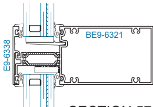
SECTION 57 O.G. HORIZONTAL
