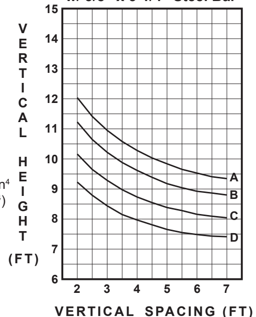
E9-6354 / E9-6355 w/ 3/8" x 3-1/4" Steel Bar
