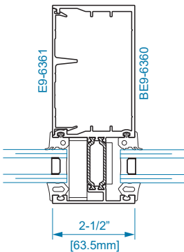
SECTION 10B FIELD GLAZED O.G. CAPTURED TUBULAR MULLION
