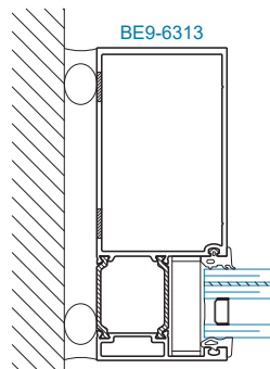
SECTION 59A TUBULAR O.G. JAMB
