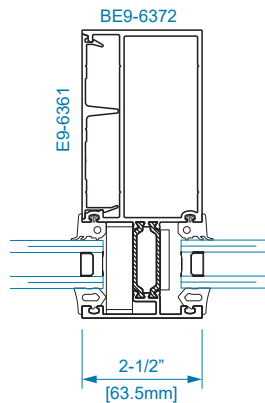
SECTION 35T DOOR JAMB w/ SIDELITE
