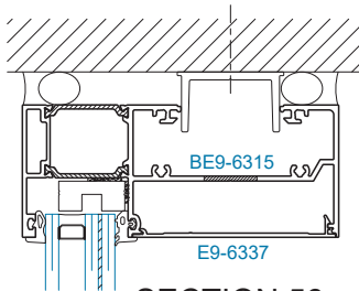
SECTION 56 O.G. HEAD
