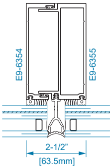
SECTION 62 SSG MULLION
