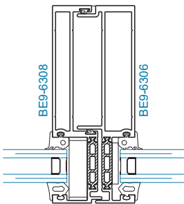
SECTION 10A OPTIONAL O.G. CAPTURED MULLION
