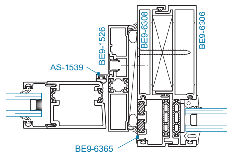
SECTION 30T DOOR JAMB w/ SIDELITE
