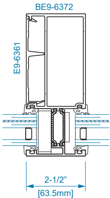
SECTION 85T DOOR JAMB w/ SIDELITE
