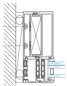
SECTION 77T DOOR JAMB @ TRANSOM
