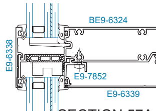
SECTION 57A OPTIONAL O.G. HORIZONTAL
