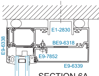
SECTION 6A OPTIONAL O.G. HEAD
