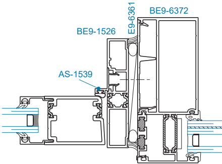
SECTION 87T DOOR JAMB w/ SIDELITE
