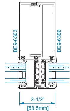
SECTION 60 O.G. CAPTURED MULLION
