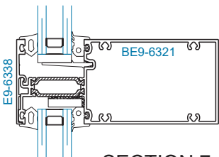
SECTION 7 O.G. HORIZONTAL
