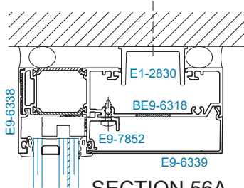
SECTION 56A OPTIONAL O.G. HEAD
