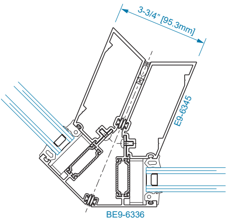
SECTION 14 135° O.S. CORNER CAPTURED MULLION
