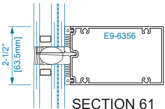
SECTION 61 SSG HORIZONTAL
