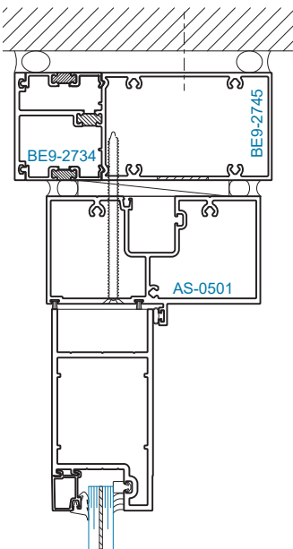
SECTION 16 DOOR HEAD w/o TRANSOM
