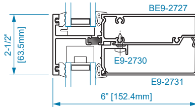
SECTION 2 HORIZONTAL
