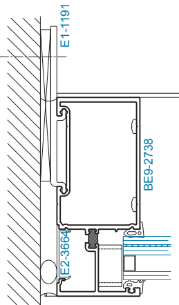
SECTION 4C HEAVY DUTY JAMB
