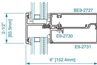
SECTION 2 HORIZONTAL
