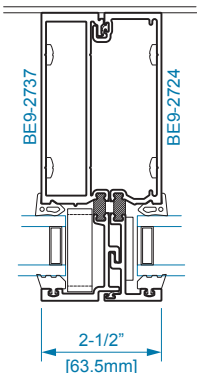
SECTION 5A HEAVY DUTY MULLION
