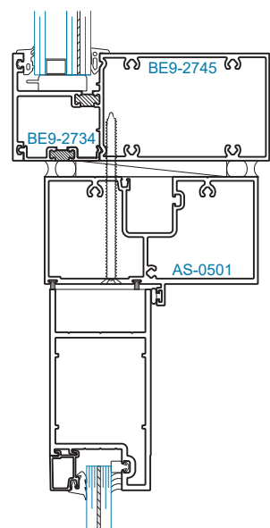
SECTION 17 DOOR HEAD w/ TRANSOM
