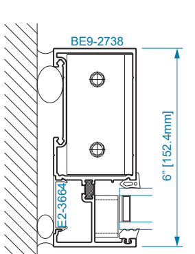
SECTION 12 JAMB @ TRANSOM w/o SIDELITE
