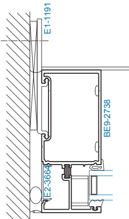
SECTION 4C HEAVY DUTY JAMB
