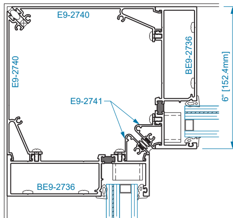
SECTION 7 90° INSIDE CORNER
