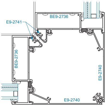
SECTION 9 90° OUTSIDE CORNER
