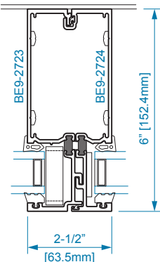
SECTION 5 MULLION
