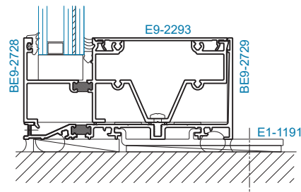
SECTION 3A SILL
