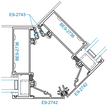
SECTION 10 135° OUTSIDE CORNER
