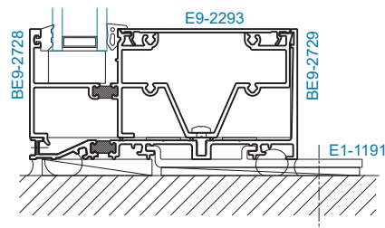
SECTION 3A SILL
