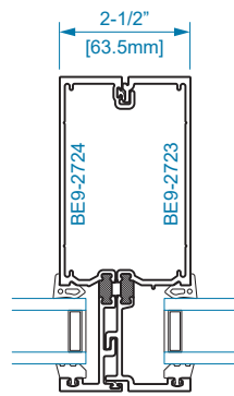
SECTION 13 JAMB @ TRANSOM w/ SIDELITE
