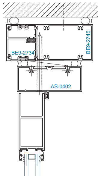
SECTION 16 DOOR HEAD w/o TRANSOM
