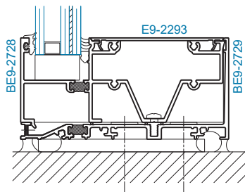
SECTION 3 SILL
