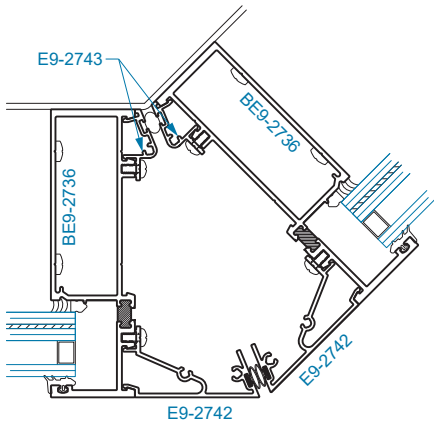
SECTION 10 135° OUTSIDE CORNER
