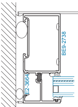
SECTION 4B HEAVY DUTY JAMB
