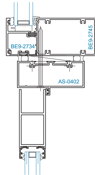
SECTION 17 DOOR HEAD w/ TRANSOM
