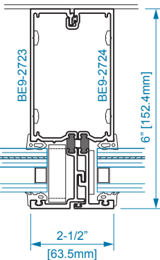
SECTION 5 MULLION
