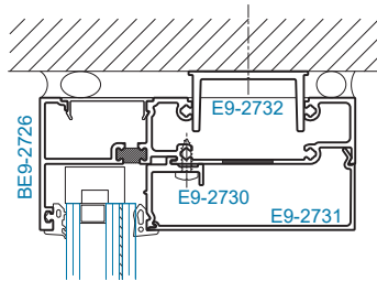
SECTION 1 HEAD
