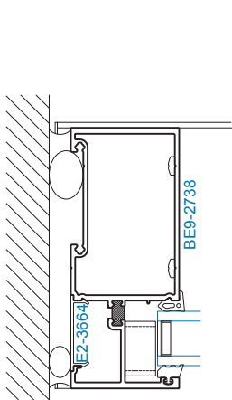
SECTION 4B HEAVY DUTY JAMB
