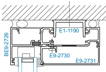
SECTION 1 HEAD
