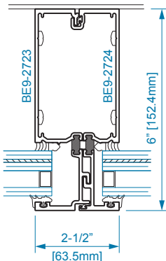
SECTION 5 MULLION
