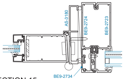
SECTION 15 DOOR JAMB w/ SIDELITE
