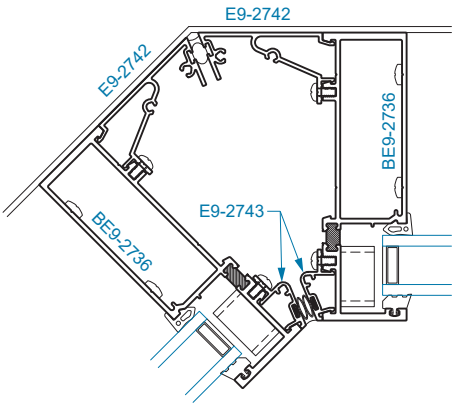
SECTION 8 135° INSIDE CORNER
