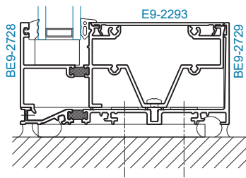
SECTION 3 SILL
