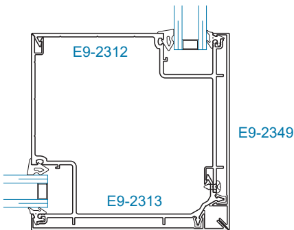
SECTION 11 90° OUTSIDE CORNER
