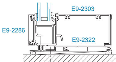
SECTION 4A SILL w/ ECONOMY SILL FLASHING
