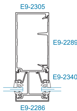
SECTION 7 VERTICAL WITH 1/4" GLAZING ADAPTOR
