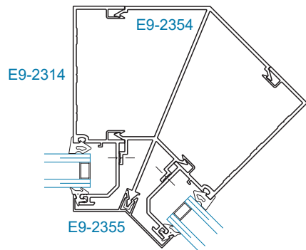
SECTION 14 135° INSIDE CORNER
