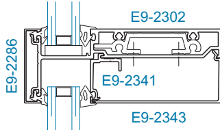
SECTION 3 HORIZONTAL
