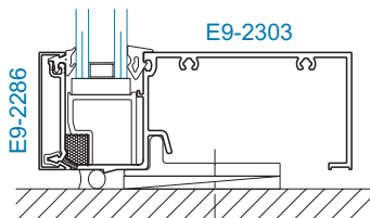
SECTION 4A SILL WITH SILL ANCHOR
