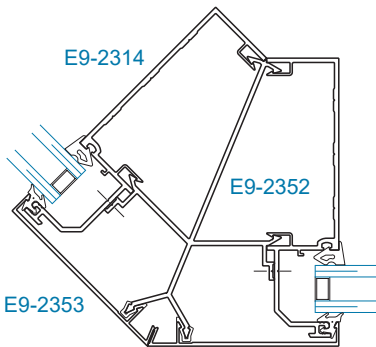
SECTION 13 135° OUTSIDE CORNER
