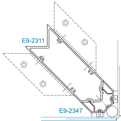
SECTION 11B SSG 90° OUTSIDE CORNER WITH 1/4" GLAZING ADAPTOR
