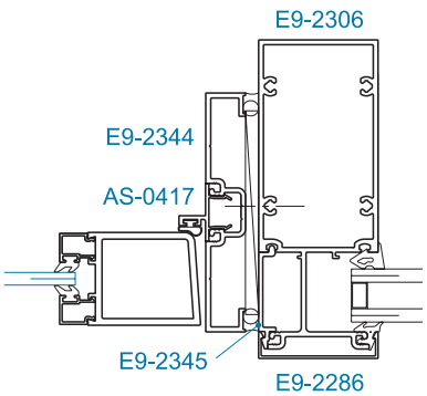
SECTION 17 DOOR JAMB WITH SIDELITE
