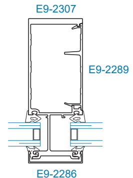
SECTION 6A HEAVY DUTY VERTICAL
