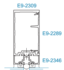
SECTION 9 SSG VERTICAL WITH 1/4" GLAZING ADAPTOR
