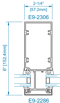
SECTION 6 TUBULAR VERTICAL
