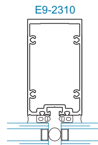
SECTION 8 SSG TUBULAR VERTICAL
