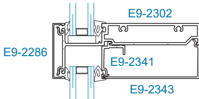
SECTION 3 HORIZONTAL
