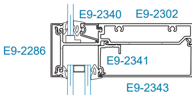
SECTION 2 HORIZONTAL WITH 1/4" GLAZING ADAPTOR
