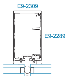
SECTION 8 SSG VERTICAL 1" GLAZING
