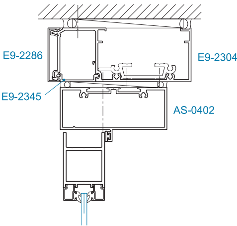
SECTION 15 DOOR HEAD WITHOUT TRANSOM
