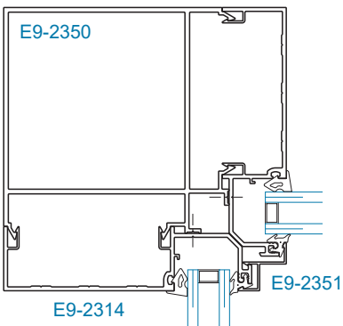
SECTION 12 90° INSIDE CORNER
