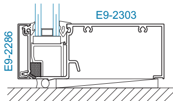
SECTION 4 SILL
