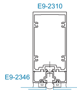
SECTION 9 SSG TUBULAR VERTICAL WITH 1/4" GLAZING ADAPTOR
