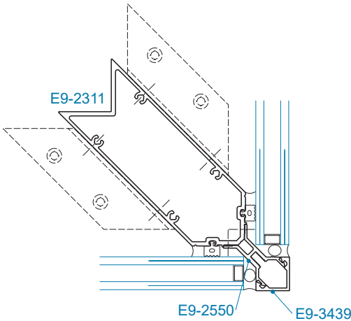
SECTION 11A SSG 90° OUTSIDE CORNER WITH 1/4" GLAZING ADAPTOR
