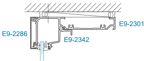
SECTION 1 HEAD WITH 1/4" GLAZING ADAPTOR
