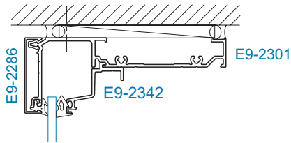
SECTION 1 HEAD WITH 1/4" GLAZING ADAPTOR
