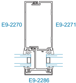
SECTION 10 EXPANSION MULLION
