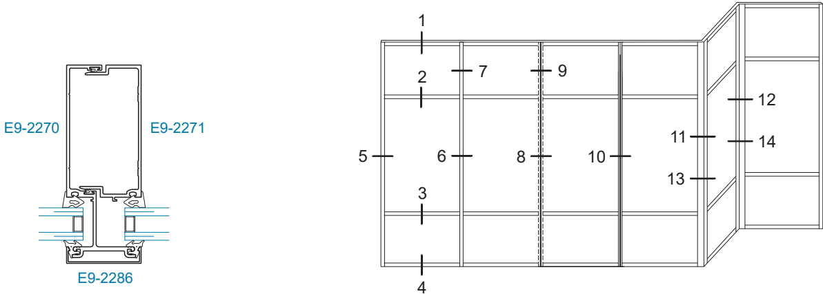
SECTION 10 EXPANSION MULLION
