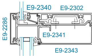
SECTION 2 HORIZONTAL WITH 1/4" GLAZING ADAPTOR
