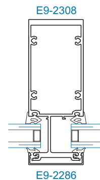
SECTION 6A HEAVY DUTY TUBULAR VERTICAL
