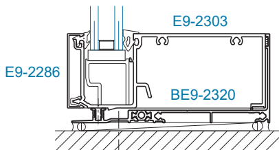
SECTION 4 SILL w/ THERMAL SILL FLASHING
