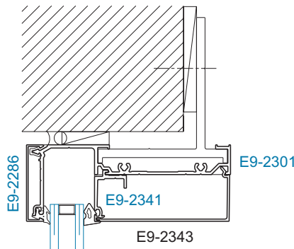
SECTION 1A HEAD WITH HEAD ANCHOR
