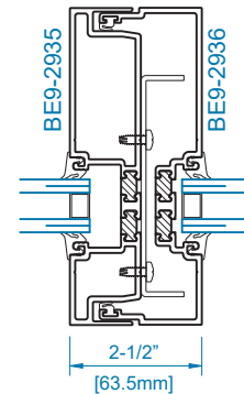
SECTION 6 EXPANSION MULLION
