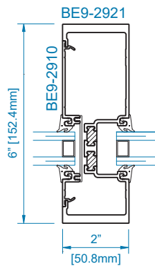
SECTION 5A HEAVY DUTY MULLION
