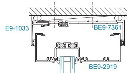
SECTION 1A HEAD RECEPTOR
