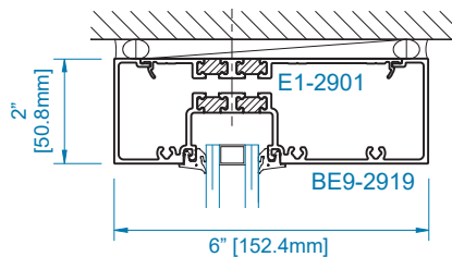
SECTION 1 HEAD
