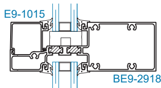
SECTION 2 HORIZONTAL
