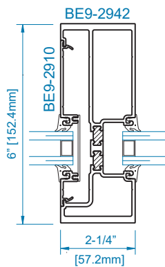
SECTION 5B HEAVY DUTY MULLION
