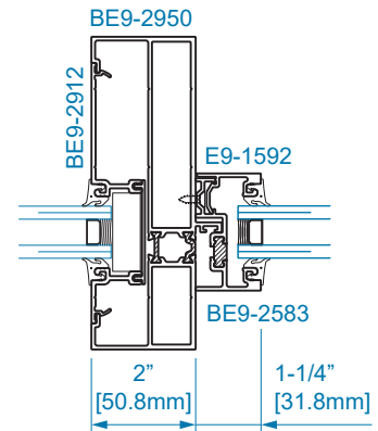
SECTION 9T DOOR JAMB @ TRANSOM
