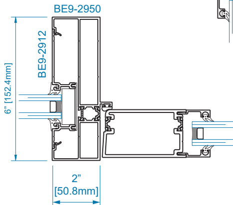
SECTION 10T SINGLE ACTING DOOR JAMB
