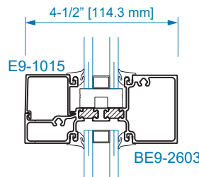
SECTION 2A OPTIONAL 4-1/2" DEPTH HORIZONTAL
