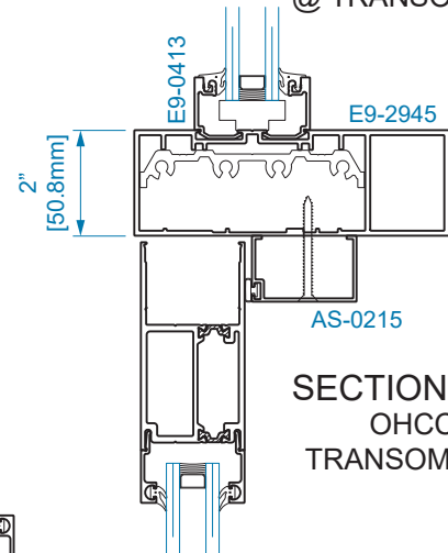
SECTION 9T DOOR JAMB @ TRANSOM
