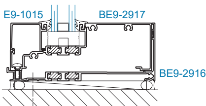
*SECTION 3 SILL
