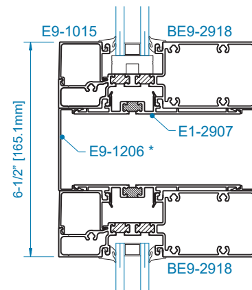
SECTION 2B OPTIONAL COMPOUND HORIZONTAL
