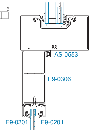
SECTION 8 TRANSOM BAR
