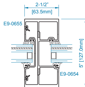
SECTION 5 MULLION ±70 PSF
