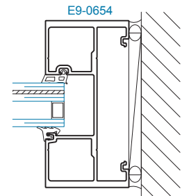
SECTION 4A opp. JAMB ±70 PSF
