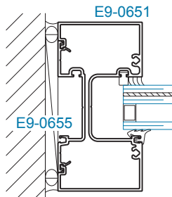
SECTION 4 JAMB ±70 PSF
