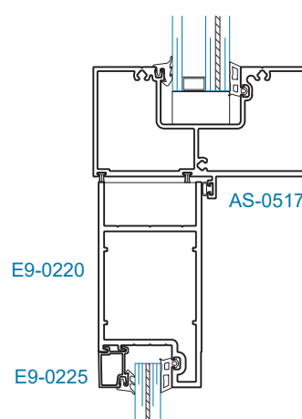
SECTION 8 TRANSOM BAR
