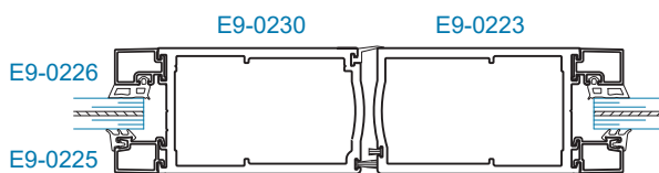
SECTION 14 MEETING STILE
