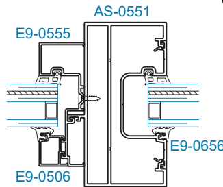
SECTION 11 JAMB @ TRANSOM w/ SIDELITE
