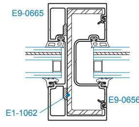
SECTION 5A MULLION +70/-90 PSF
