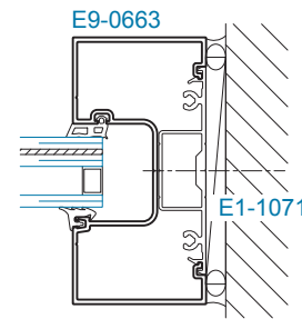
SECTION 4C opp. JAMB +70/-90 PSF
