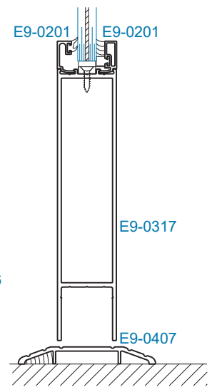
SECTION 9 AIR TIGHT THRESHOLD
