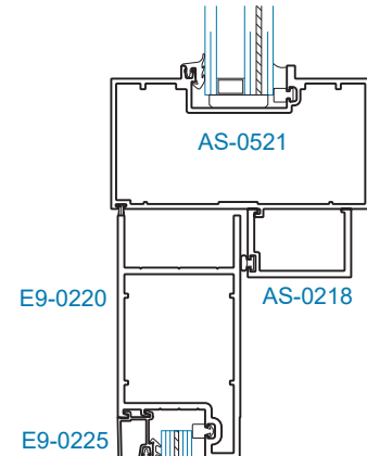
SECTION 8A TRANSOM BAR FOR OHCC
