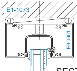
SECTION 1 HEAD @ TRANSOM
