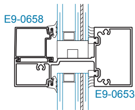
SECTION 2 HORIZONTAL +70/-90 PSF
