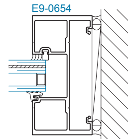
SECTION 4A opp. JAMB ±70 PSF
