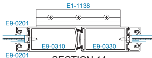
SECTION 14 MEETING STILE
