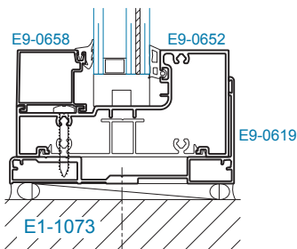
SECTION 3 SILL +70/-90 PSF
