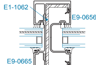
SECTION 5A MULLION w/ STEEL +70/-90 PSF
