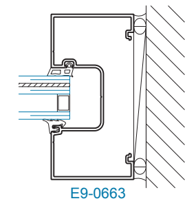
SECTION 4A opp. JAMB ±50 PSF
