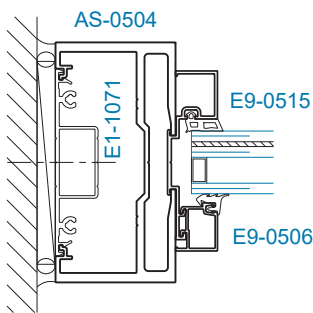
SECTION 10 JAMB @ TRANSOM w/o SIDELITE
