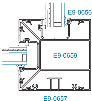
SECTION 7A 90° OUTSIDE CORNER
