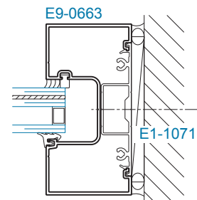
SECTION 4C opp. JAMB +70/-90 PSF
