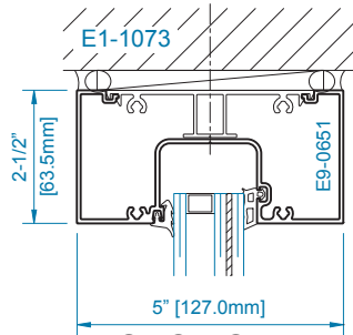
SECTION 1 HEAD +70/-90 PSF
