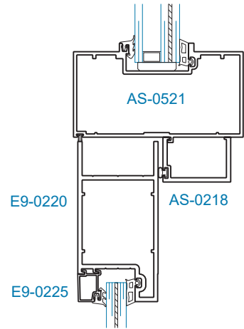
SECTION 8A TRANSOM BAR FOR OHCC
