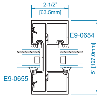
SECTION 5 MULLION ±70 PSF
