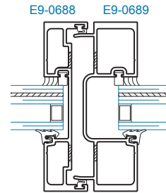
SECTION 6 EXPANSION MULLION ±65 PSF
