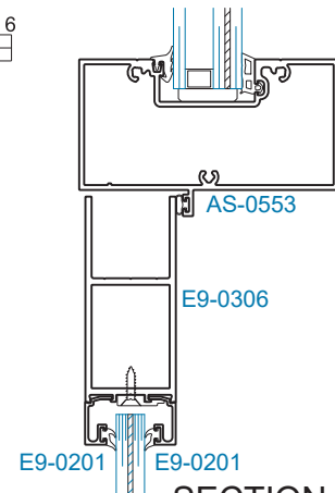
SECTION 8 TRANSOM BAR
