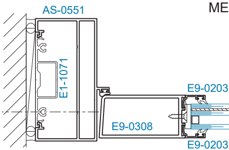
SECTION 12 DOOR JAMB w/o SIDELITE 35HL INSULATING GLASS OPTION SHOWN
