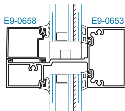
SECTION 2 HORIZONTAL +70/-90 PSF
