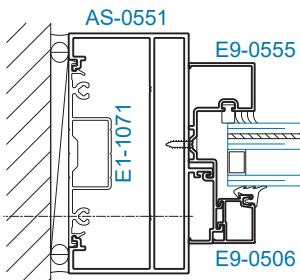
SECTION 10 JAMB @ TRANSOM w/o SIDELITE
