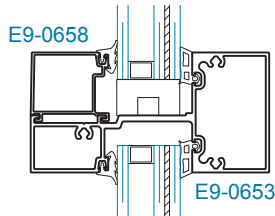
SECTION 2 HORIZONTAL ±50 PSF
