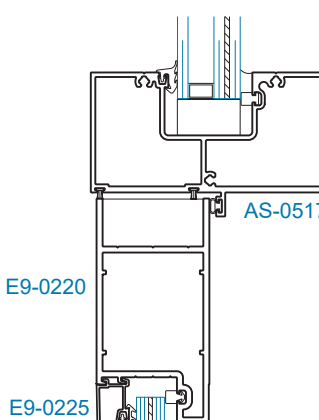
SECTION 8 TRANSOM BAR
