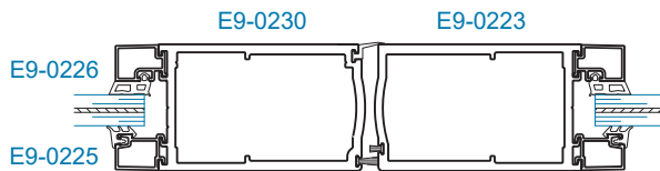
SECTION 14 MEETING STILE
