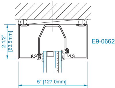
SECTION 1 HEAD ±50 PSF
