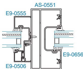
SECTION 11 JAMB @ TRANSOM w/ SIDELITE
