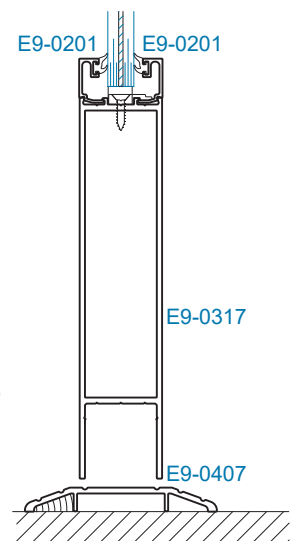
SECTION 9 AIR TIGHT THRESHOLD
