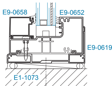
SECTION 3 SILL +70/-90 PSF
