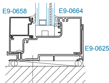
SECTION 3 SILL ±50 PSF
