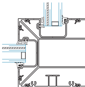
SECTION 7A 90° OUTSIDE CORNER
