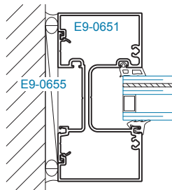
SECTION 4 JAMB ±70 PSF
