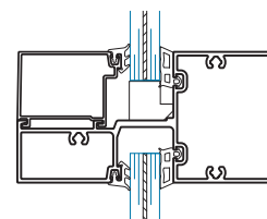
9/16" Dry Glazing
