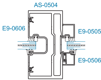
SECTION 6 JAMB @ TRANSOM w/ SIDELITE (±70 psf)
