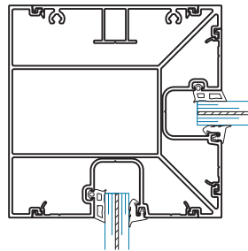
SECTION 20 90° INSIDE CORNER
