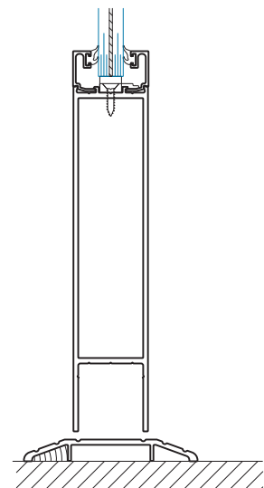
SECTION 19 THRESHOLD
