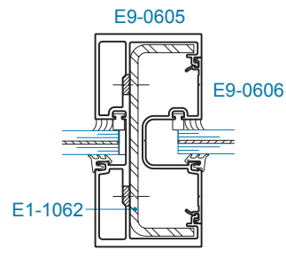
SECTION 5A VERTICAL w/ STEEL REINFORCING (+70/-90 psf)
