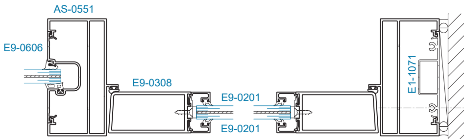
SECTION 15 JAMB w/ SIDELITE
