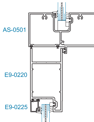
SECTION 11 TRANSOM BAR (+70/-90 psf)
