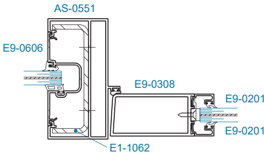
SECTION 15A JAMB w/ SIDELITE w/ STEEL REINFORCING
