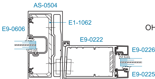
SECTION 8A JAMB w/ SIDELITE w/ STEEL REINFORCING
