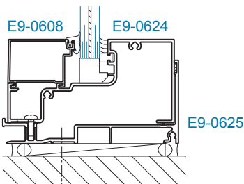
SECTION 3 SILL ±50 PSF
