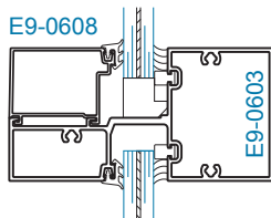
SECTION 2 HORIZONTAL (+70/-90 psf)
