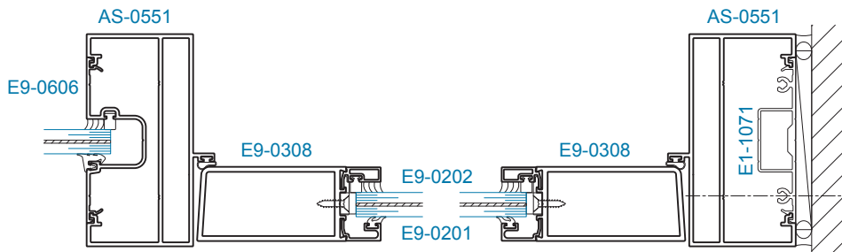
SECTION 8 JAMB w/ SIDELITE (±50 psf)
