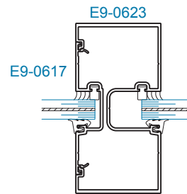
SECTION 5 MULLION ±50 PSF
