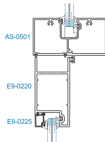
SECTION 11 TRANSOM BAR
