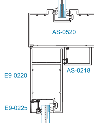
SECTION 11A OHCC TRANSOM BAR (+70/-90 psf)
