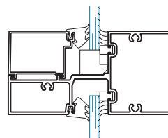
1/4" Glazing (Not in FPA)
