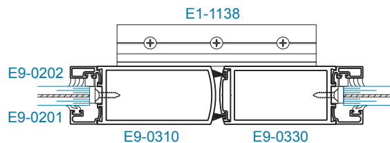
SECTION 9 MEETING STILE (±50 psf)
