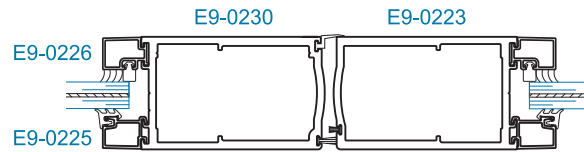
SECTION 9 MEETING STILE (+70/-90 psf)
