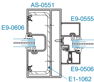
SECTION 13A JAMB @ TRANSOM w/ STEEL REINFORCING
