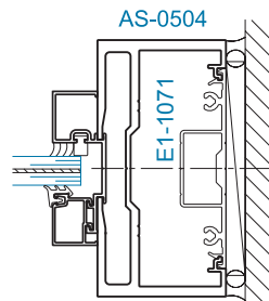
SECTION 7 JAMB @ TRANSOM w/o SIDELITE (+70/-90 psf)
