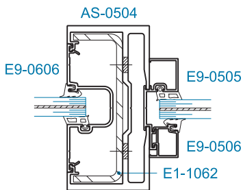
SECTION 6A JAMB @ TRANSOM w/ STEEL REINFORCING
