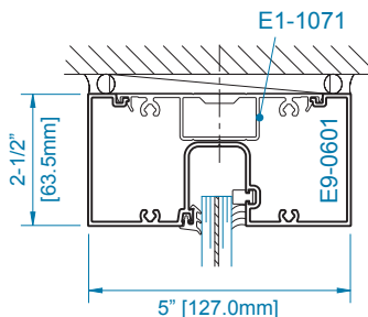
SECTION 1 HEAD (+70/-90 psf)
