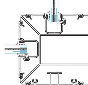
SECTION 20A 90° OUTSIDE CORNER
