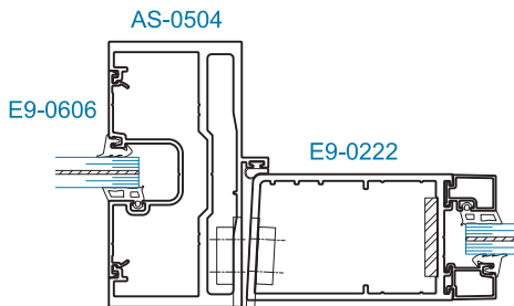
SECTION 8 JAMB w/ SIDELITE
