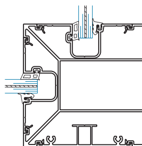
SECTION 20A 90° OUTSIDE CORNER
