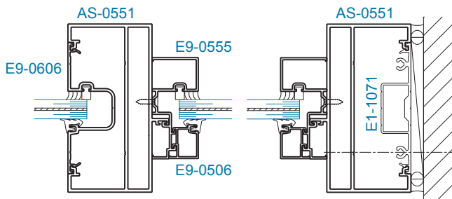
SECTION 6 JAMB @ TRANSOM w/ SIDELITE (±50 psf)
