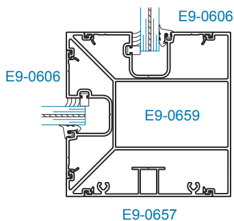
SECTION 20A 90° OUTSIDE CORNER
