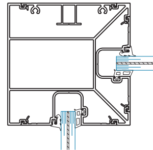
SECTION 20 90° INSIDE CORNER
