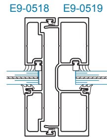
SECTION 5B EXPANSION MULLION (±65 psf)
