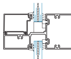
9/16" Glazing
