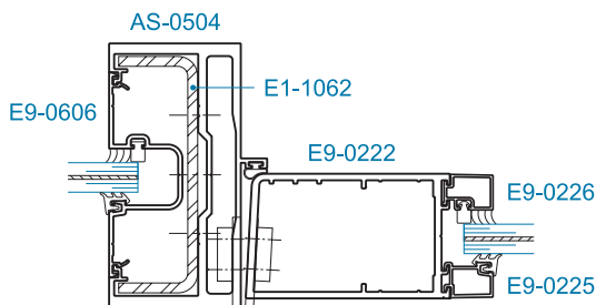
SECTION 8A JAMB w/ SIDELITE w/ STEEL REINFORCING (+70/-90 psf)
