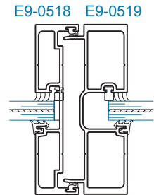
SECTION 5A EXPANSION MULLION ±65 PSF
