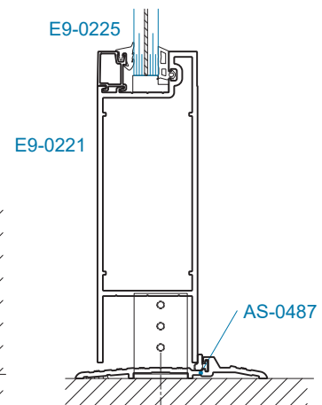
SECTION 12 AIR RESISTANT THRESHOLD
