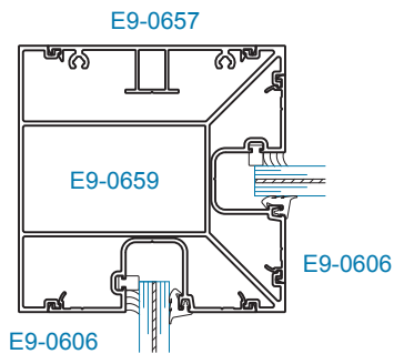
SECTION 20 90° INSIDE CORNER
