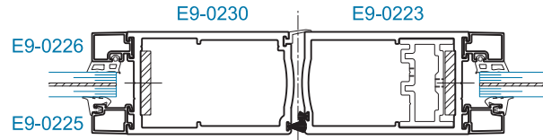
SECTION 9 MEETING STILE
