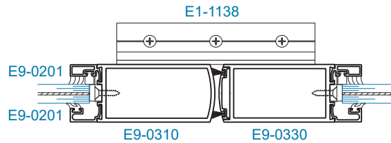
SECTION 16 MEETING STILE
