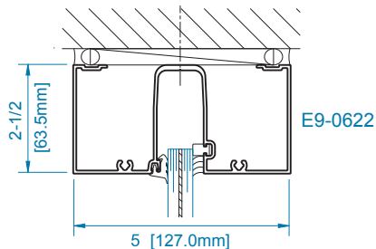
SECTION 1 HEAD ±50 PSF
