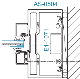
SECTION 7 JAMB @ TRANSOM w/o SIDELITE
