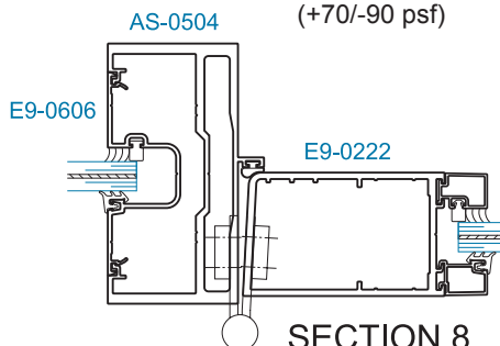
SECTION 8A JAMB w/ SIDELITE w/ STEEL REINFORCING (+70/-90 psf)
