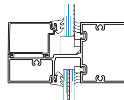
7/16" Glazing (Not in FPA)
