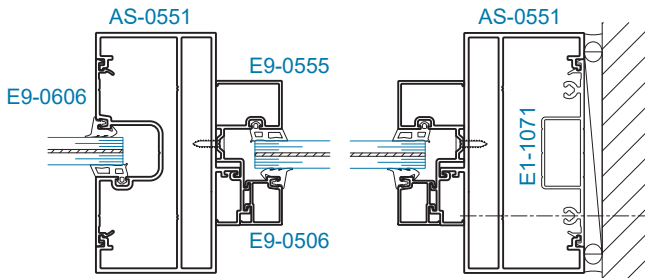
SECTION 13 JAMB @ TRANSOM w/ SIDELITE
