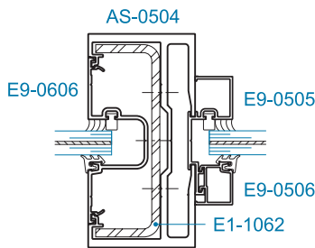
SECTION 6A JAMB @ TRANSOM w/ STEEL REINFORCING (+70/-90 psf)
