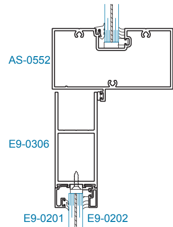
SECTION 11 TRANSOM BAR (±50 psf)
