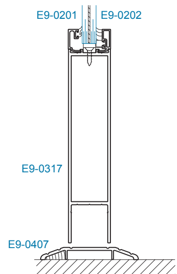
SECTION 12 THRESHOLD (±50 psf)
