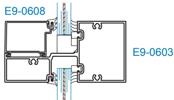
SECTION 2 HORIZONTAL
