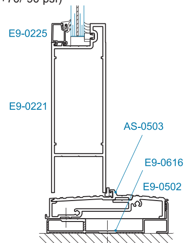
SECTION 12 WATER RESISTANT THRESHOLD
