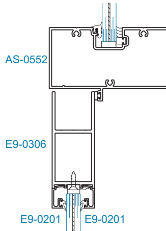
SECTION 18 TRANSOM BAR
