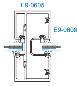
SECTION 5 VERTICAL (±70 psf)
