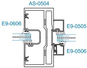
SECTION 6 JAMB @ TRANSOM w/ SIDELITE
