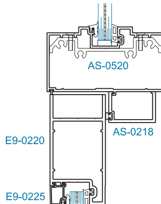
SECTION 11A OHCC TRANSOM BAR
