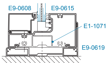
SECTION 3 SILL (+70/-90 psf)
