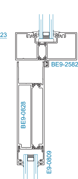
SECTION 17B OPTIONAL 6-1/2" TRANSOM BAR
