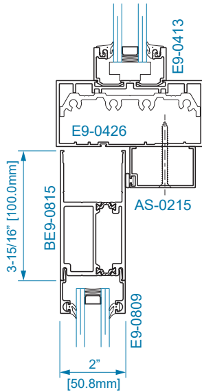
SECTION 17A STD. TRANSOM BAR w/ OHCC*
