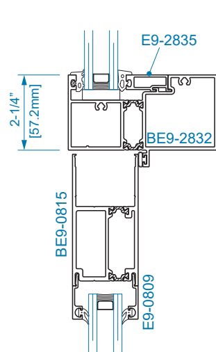
SECTION 34B STD. TRANSOM BAR
