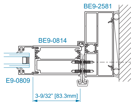
SECTION 23A CONTINUOUS HINGE JAMB
