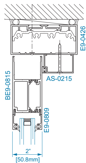
SECTION 21A STD. TOP RAIL w/ OHCC
