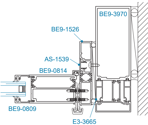
SECTION 33D HINGE JAMB
