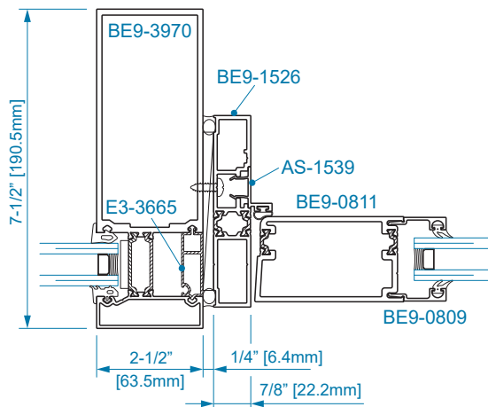
SECTION 31D LOCK JAMB w/ SIDELITE
