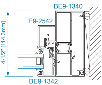
SECTION 32 DOOR JAMB AT TRANSOM
