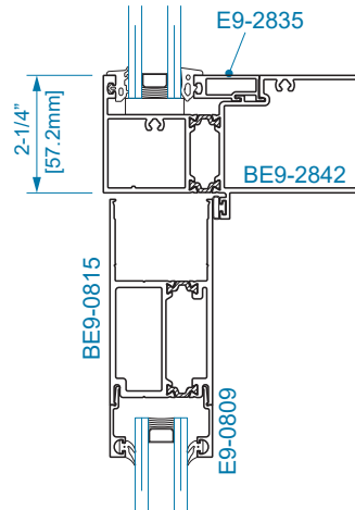
SECTION 34C STD. TRANSOM BAR
