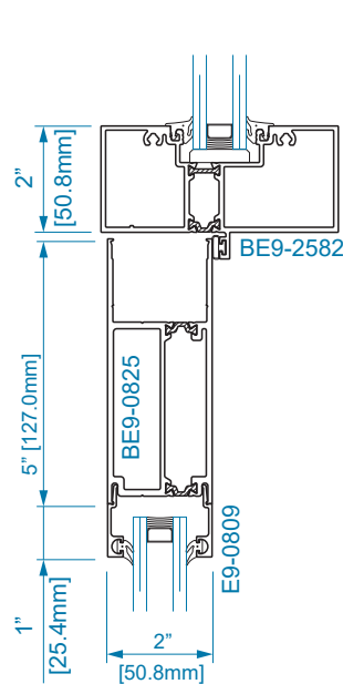
SECTION 30 STD. TRANSOM BAR
