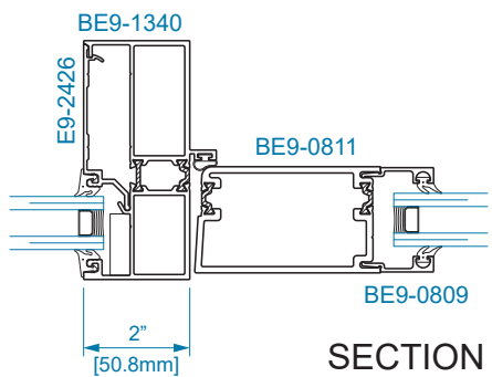
SECTION 30 DOOR JAMB AT TRANSOM w/ SIDELITE
