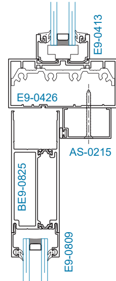
SECTION 30A STD. TRANSOM BAR w/ OHCC
