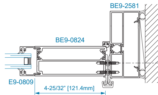
SECTION 28A CONTINUOUS HINGE JAMB
