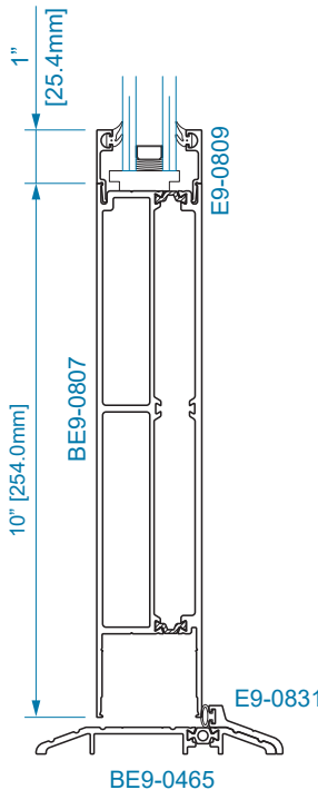
SECTION 4A w/ OPTIONAL DOOR STOP
