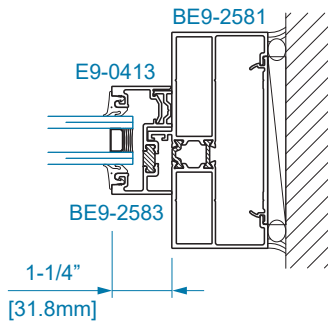
SECTION 20 DOOR JAMB AT TRANSOM
