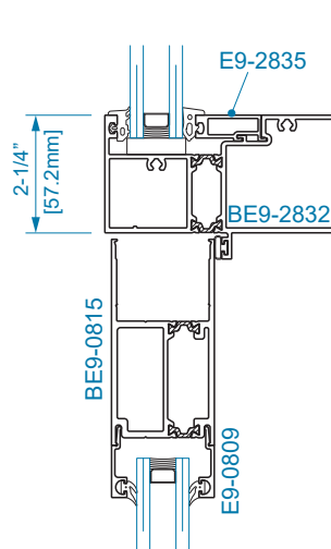
SECTION 34B STD. TRANSOM BAR
