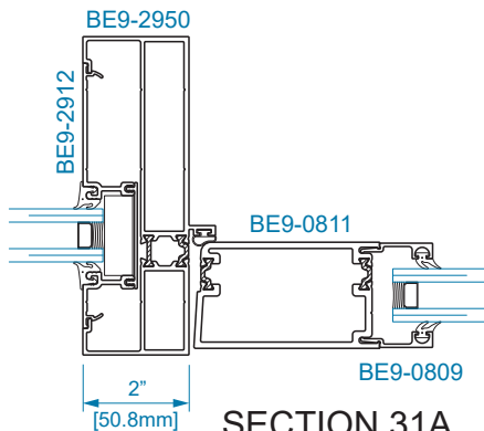
SECTION 31A LOCK JAMB w/ SIDELITE
