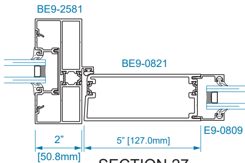
SECTION 27 HINGE JAMB w/ SIDELITE
