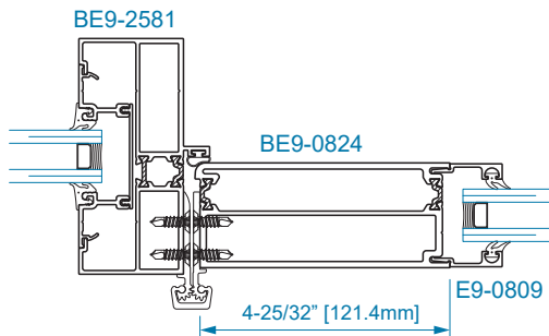
SECTION 27A CONTINUOUS HINGE JAMB w/ SIDELITE
