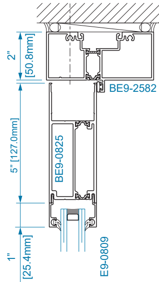
SECTION 26 STD. TOP RAIL
