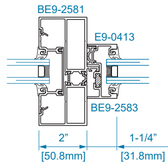
SECTION 19 DOOR JAMB AT TRANSOM w/ SIDELITE
