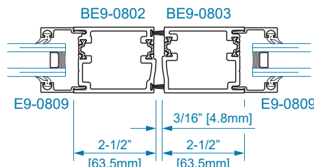
SECTION 16 MEETING STILES
