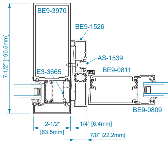
SECTION 31D LOCK JAMB w/ SIDELITE
