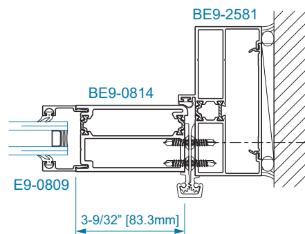
SECTION 23A CONTINUOUS HINGE JAMB
