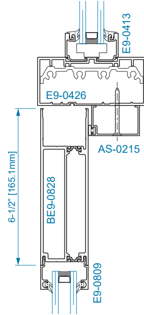
SECTION 17C OPTIONAL 6-1/2" TRANSOM BAR w/ OHCC
