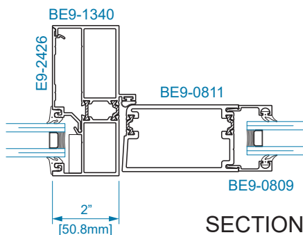
SECTION 30 DOOR JAMB AT TRANSOM w/ SIDELITE
