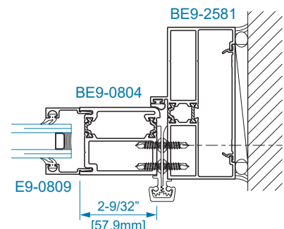
SECTION 15A CONTINUOUS HINGE JAMB
