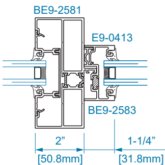
SECTION 19 DOOR JAMB AT TRANSOM w/ SIDELITE
