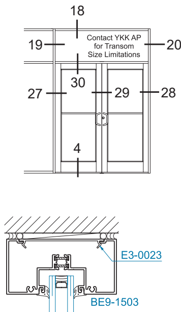
SECTION 18 HEAD AT TRANSOM
