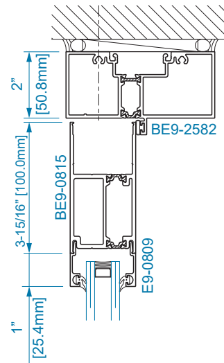
SECTION 21 STD. TOP RAIL
