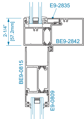
SECTION 34C STD. TRANSOM BAR
