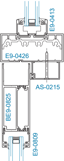
SECTION 30A STD. TRANSOM BAR w/ OHCC
