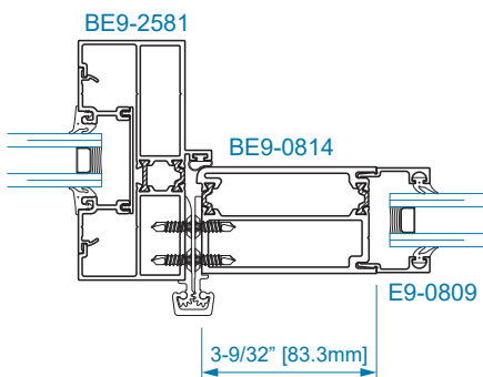
SECTION 22A CONTINUOUS HINGE JAMB w/ SIDELITE
