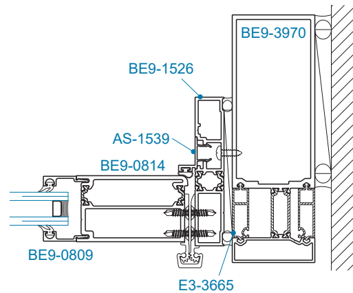
SECTION 33D HINGE JAMB
