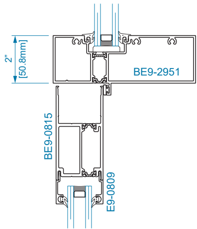
SECTION 34A STD. TRANSOM BAR
