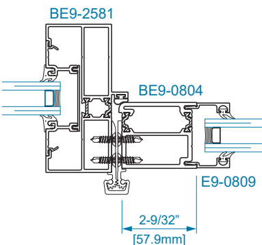
SECTION 14A CONTINUOUS HINGE JAMB w/ SIDELITE
