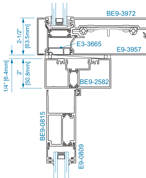
SECTION 34D STD. TRANSOM BAR
