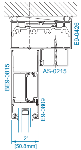
SECTION 21A STD. TOP RAIL w/ OHCC
