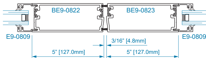
SECTION 29 MEETING STILES
