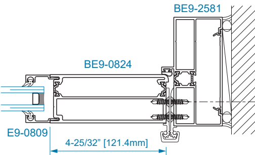
SECTION 28A CONTINUOUS HINGE JAMB
