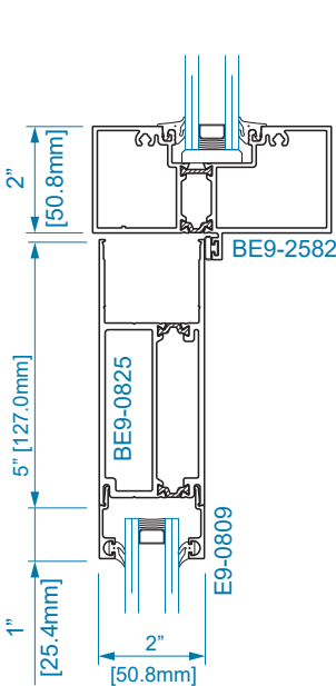
SECTION 30 STD. TRANSOM BAR
