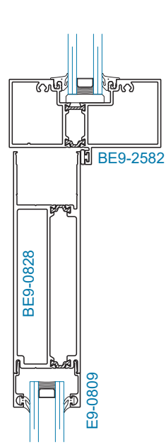
SECTION 17B OPTIONAL 6-1/2" TRANSOM BAR
