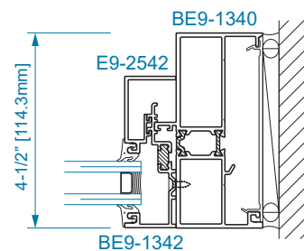
SECTION 32 DOOR JAMB AT TRANSOM
