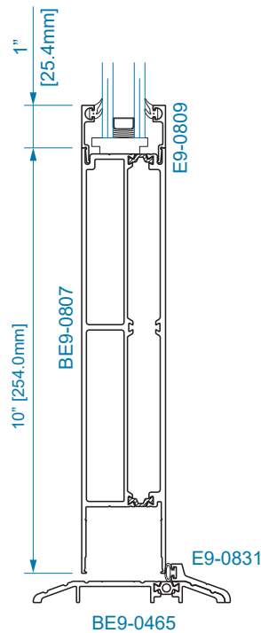
SECTION 4A w/ OPTIONAL DOOR STOP
