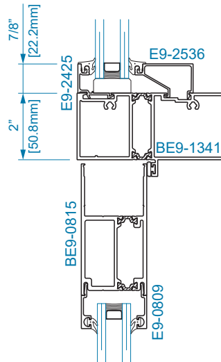
SECTION 34 STD. TRANSOM BAR
