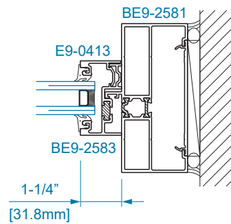
SECTION 20 DOOR JAMB AT TRANSOM
