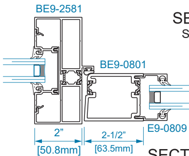
SECTION 14 HINGE JAMB w/ SIDELITE
