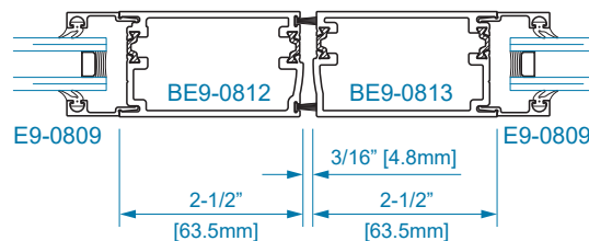
SECTION 24 MEETING STILES
