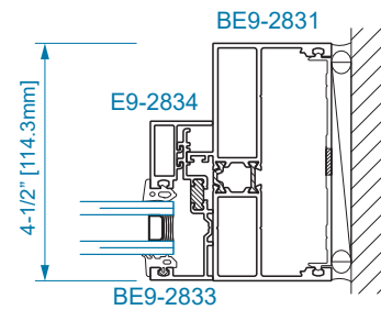
SECTION 32B DOOR JAMB AT TRANSOM
