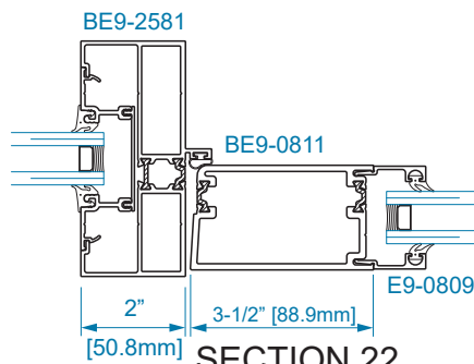
SECTION 22 HINGE JAMB w/ SIDELITE
