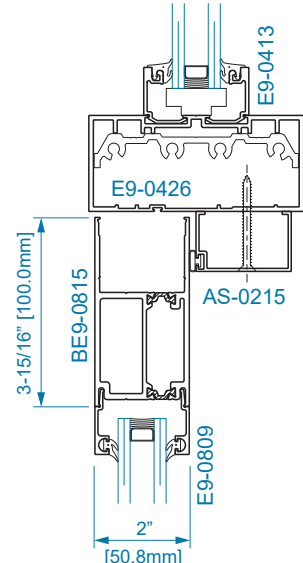
SECTION 17A STD. TRANSOM BAR w/ OHCC*
