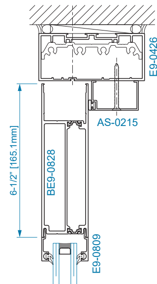
SECTION 13C OPTIONAL 6-1/2" TOP RAIL w/ OHCC
