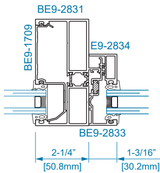
SECTION 34B STD. TRANSOM BAR
