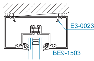
SECTION 18 HEAD AT TRANSOM
