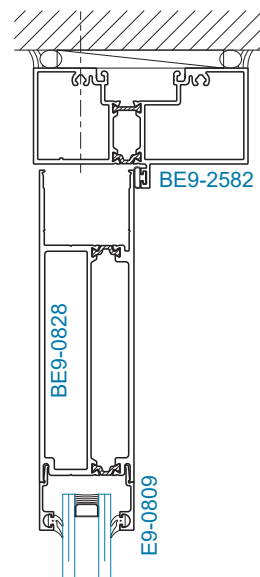
SECTION 13B OPTIONAL 6-1/2" TOP RAIL
