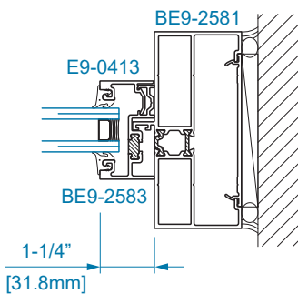
SECTION 20 DOOR JAMB AT TRANSOM
