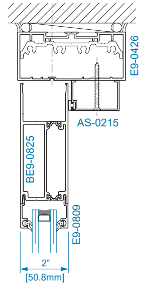
SECTION 26A STD. TOP RAIL w/ OHCC
