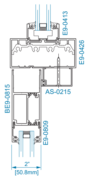
SECTION 25A STD. TRANSOM BAR w/ OHCC
