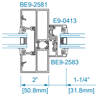
SECTION 19 DOOR JAMB AT TRANSOM w/ SIDELITE
