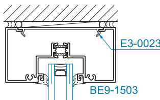
SECTION 18 HEAD AT TRANSOM
