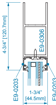
SECTION 1A 1" DRY GLAZING
