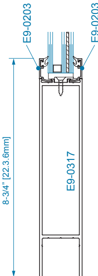
SECTION 2A 8" BOTTOM RAIL 1" DRY GLAZING
