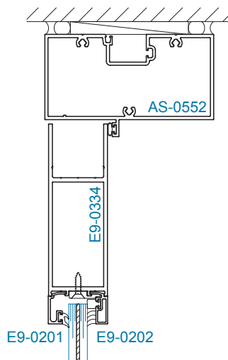
SECTION 3 OFFSET HUNG 9/16" DOOR GLAZING
