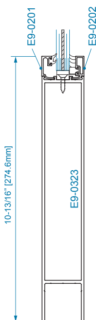
SECTION 3 10" BOTTOM RAIL 9/16" WET GLAZING
