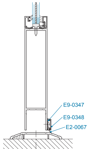
SECTION 2 W/ DOOR SWEEP
