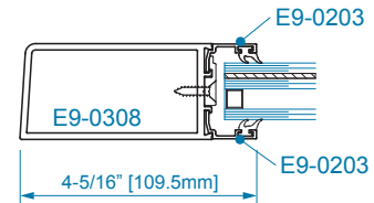
SECTION 4A OFFSET HUNG 1" DRY GLAZING
