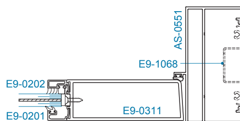
SECTION 5 OFFSET HUNG
