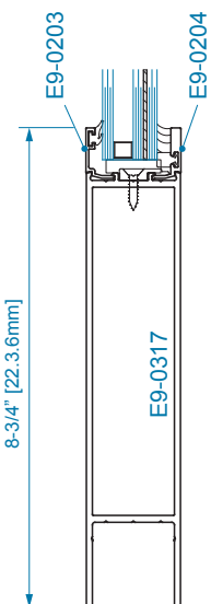
SECTION 2A 8" BOTTOM RAIL 1" WET GLAZING
