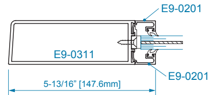
SECTION 4 OFFSET HUNG 9/16" DRY GLAZING
