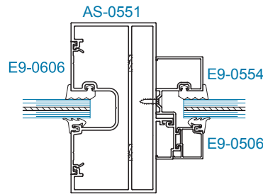
SECTION 1 9/16" GLAZING
