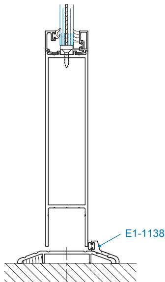
SECTION 1 W/ THRESHOLD STOP
