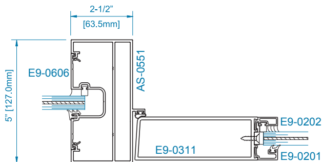
SECTION 2 OFFSET HUNG 9/16" GLAZING SIDELITE
