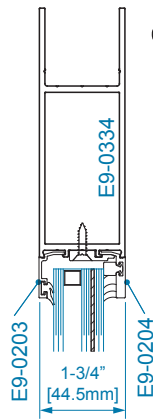
SECTION 1A 1" WET GLAZING
