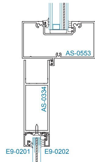
SECTION 4A OFFSET HUNG 9/16" DOOR GLAZING 1-5/16" TRANSM GLAZING
