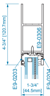
SECTION 1A 1" WET GLAZING
