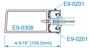
SECTION 4 OFFSET HUNG 9/16" DRY GLAZING
