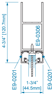
SECTION 1 9/16" DRY GLAZING
