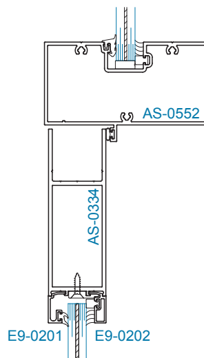
SECTION 4 OFFSET HUNG 9/16" DOOR GLAZING 9/16" TRANSM GLAZING
