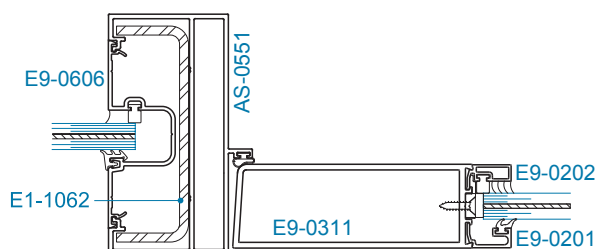
SECTION 4 OFFSET HUNG w/ OPTIONAL STEEL REINFORCEMENT
