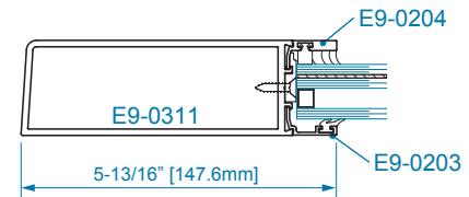
SECTION 4A OFFSET HUNG 1" WET GLAZING
