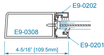
SECTION 4 OFFSET HUNG 9/16" WET GLAZING
