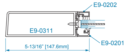
SECTION 4 OFFSET HUNG 9/16" WET GLAZING
