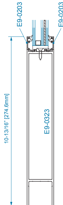
SECTION 3 10" BOTTOM RAIL 1" DRY GLAZING
