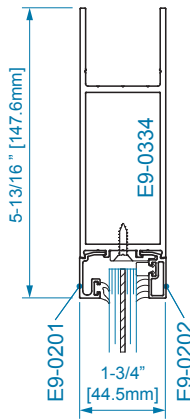
SECTION 1 9/16" WET GLAZING
