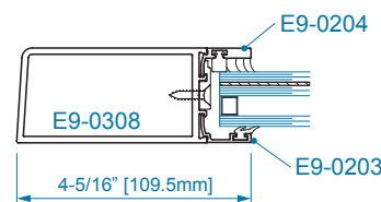
SECTION 4A OFFSET HUNG 1" WET GLAZING
