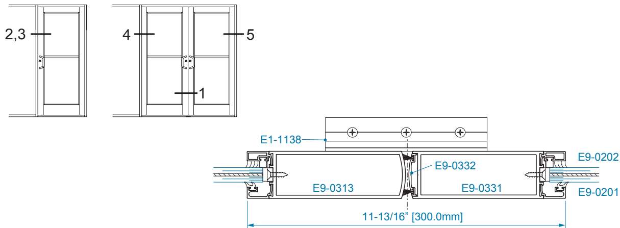
SECTION 1 MEETING STILES
