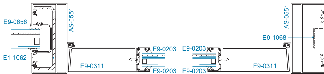
SECTION 3 OFFSET HUNG w/ OPTIONAL STEEL REINFORCEMENT
