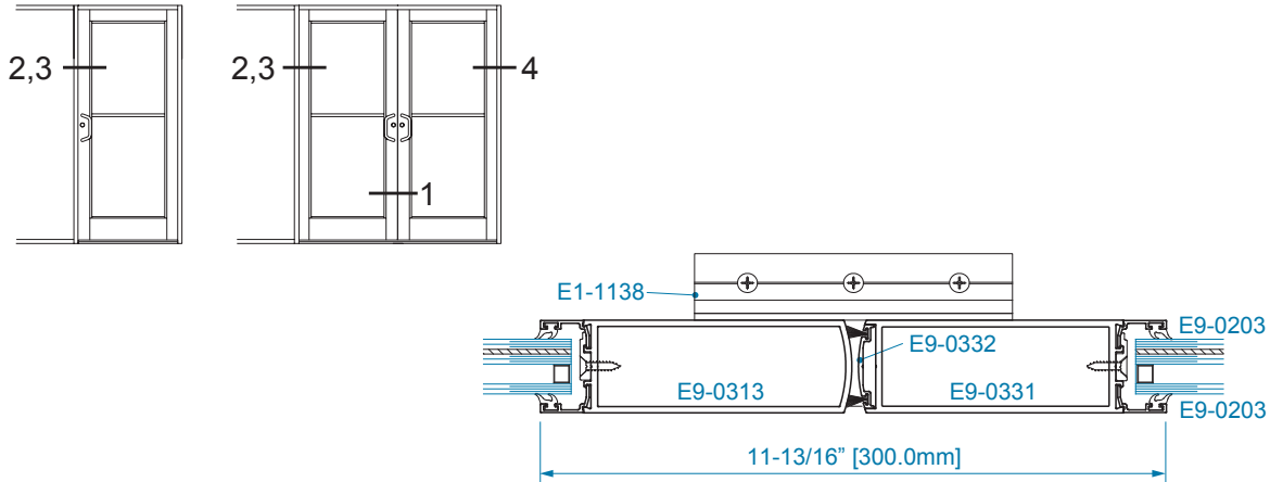
SECTION 1 MEETING STILES
