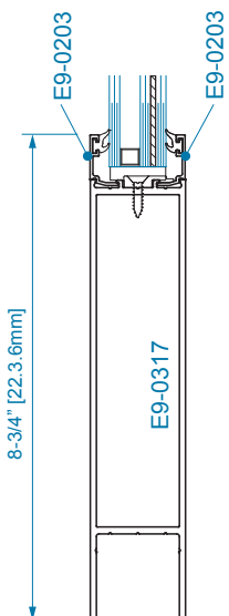
SECTION 2A 8" BOTTOM RAIL 1" DRY GLAZING
