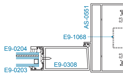
SECTION 4 OFFSET HUNG
