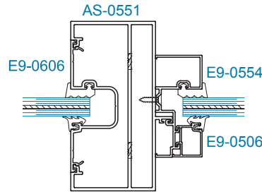
SECTION 1 9/16" GLAZING
