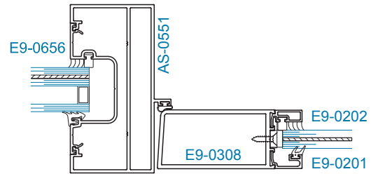
SECTION 3 OFFSET HUNG 1-5/16" GLAZING SIDELITE
