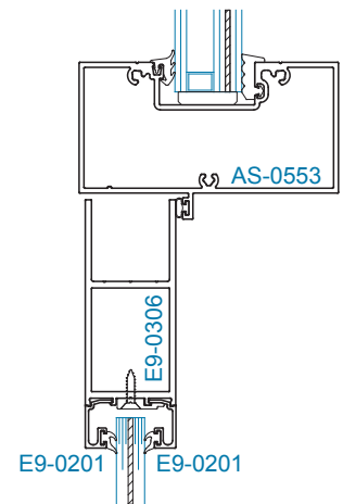
SECTION 4A OFFSET HUNG 9/16" DOOR GLAZING 1-5/16" TRANSOM GLAZING
