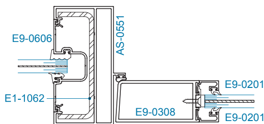
SECTION 4 OFFSET HUNG w/ OPTIONAL STEEL REINFORCEMENT
