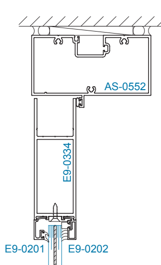
SECTION 3 OFFSET HUNG 9/16" DOOR GLAZING
