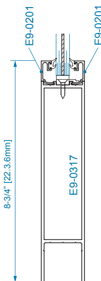
SECTION 2 8" BOTTOM RAIL 9/16" DRY GLAZING
