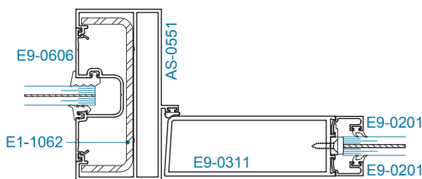
SECTION 4 OFFSET HUNG w/ OPTIONAL STEEL REINFORCEMENT
