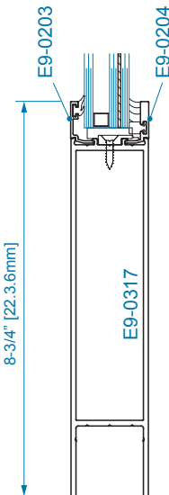
SECTION 2A 8" BOTTOM RAIL 1" WET GLAZING
