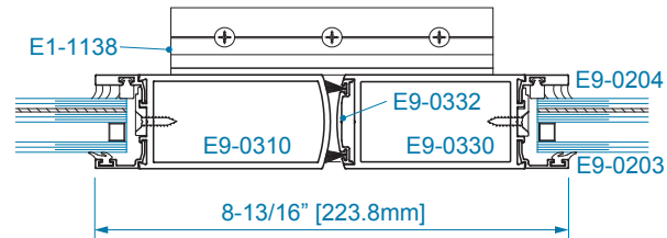
SECTION 1 MEETING STILES
