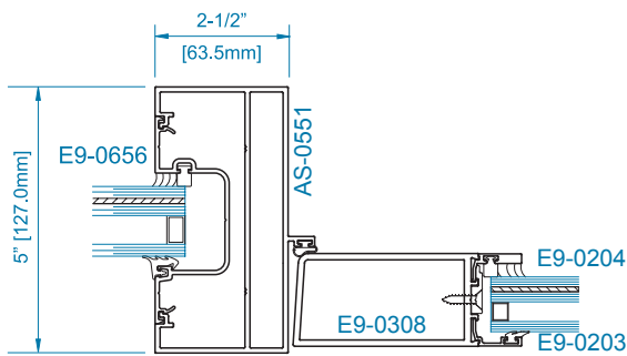
SECTION 2 OFFSET HUNG 1-5/16" GLAZING SIDELITE
