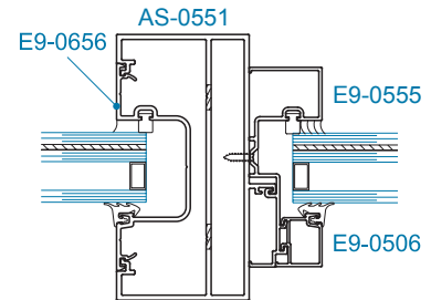
SECTION 1A 1-5/16" GLAZING
