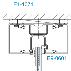
SECTION 2 9/16" GLAZING
