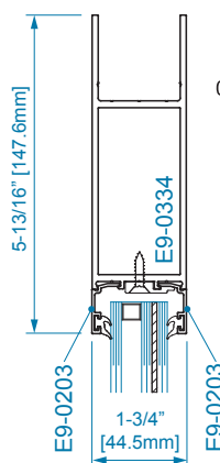
SECTION 1A 1" DRY GLAZING
