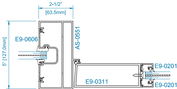
SECTION 2 OFFSET HUNG 9/16" GLAZING SIDELITE
