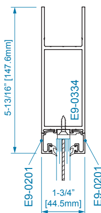
SECTION 1 9/16" DRY GLAZING
