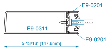
SECTION 4 OFFSET HUNG 9/16" DRY GLAZING
