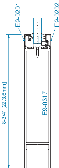
SECTION 2 8" BOTTOM RAIL 9/16" WET GLAZING
