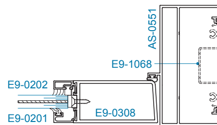
SECTION 5 OFFSET HUNG
