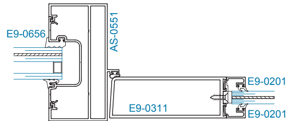
SECTION 3 OFFSET HUNG 1-5/16" GLAZING SIDELITE
