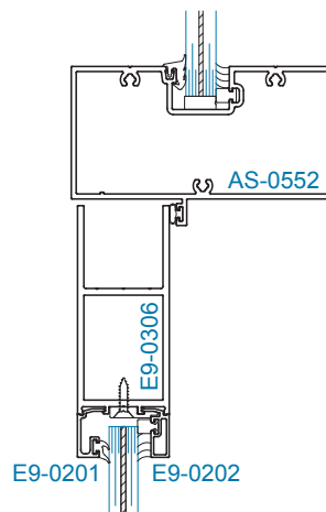
SECTION 4 OFFSET HUNG 9/16" DOOR GLAZING 9/16" TRANSOM GLAZING
