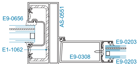
SECTION 3 OFFSET HUNG w/ OPTIONAL STEEL REINFORCEMENT
