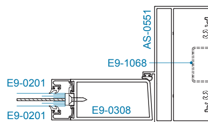
SECTION 5 OFFSET HUNG
