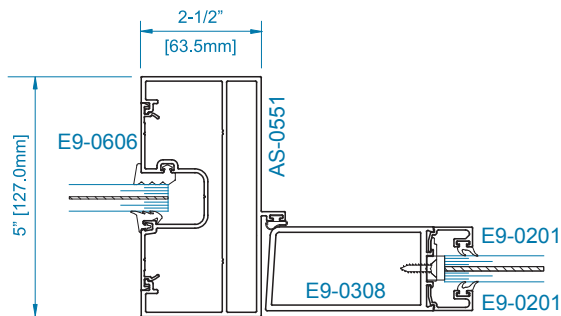
SECTION 2 OFFSET HUNG 9/16" GLAZING SIDELITE
