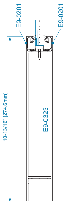
SECTION 3 10" BOTTOM RAIL 9/16" DRY GLAZING
