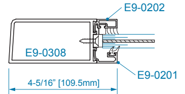
SECTION 4 OFFSET HUNG 9/16" WET GLAZING
