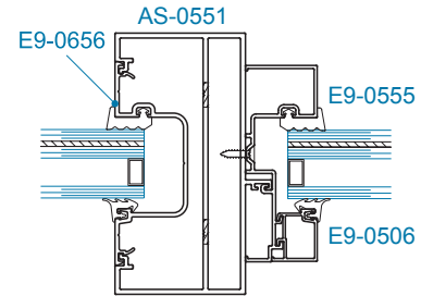
SECTION 1A 1-5/16" GLAZING
