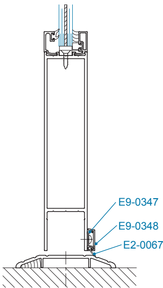
SECTION 2 W/ DOOR SWEEP
