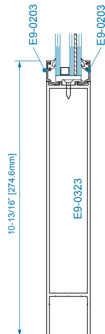
SECTION 3A 10" BOTTOM RAIL 1" DRY GLAZING
