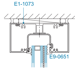
SECTION 2A 1-5/16" GLAZING
