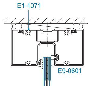
SECTION 2 9/16" GLAZING
