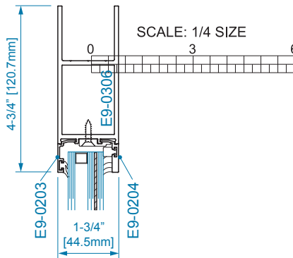
SECTION 1A 1" WET GLAZING
