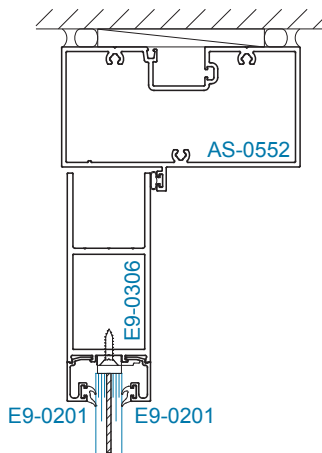
SECTION 3 OFFSET HUNG 9/16" DOOR GLAZING
