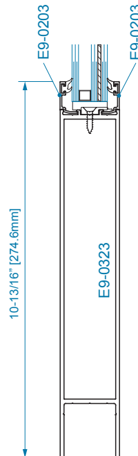
SECTION 3 10" BOTTOM RAIL 1" DRY GLAZING
