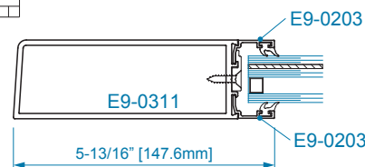
SECTION 4A OFFSET HUNG 1" DRY GLAZING
