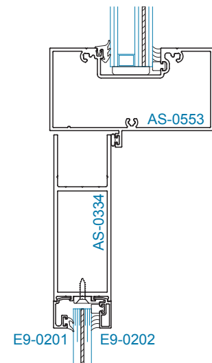
SECTION 4A OFFSET HUNG 9/16" DOOR GLAZING 1-5/16" TRANSOM GLAZING
