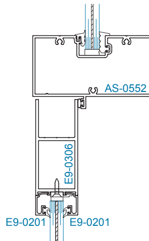
SECTION 4 OFFSET HUNG 9/16" DOOR GLAZING 9/16" TRANSOM GLAZING
