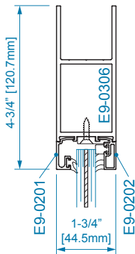
SECTION 1 9/16" WET GLAZING
