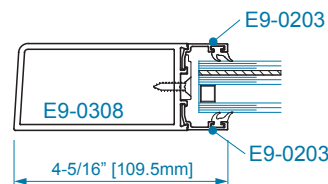
SECTION 4A OFFSET HUNG 1" DRY GLAZING
