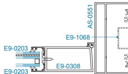
SECTION 4 OFFSET HUNG
