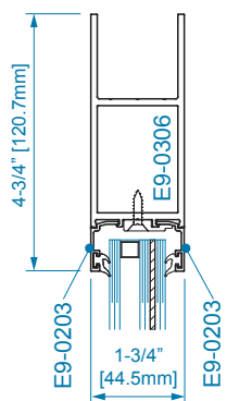
SECTION 1A 1" DRY GLAZING
