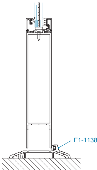
SECTION 1 W/ THRESHOLD STOP
