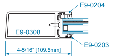
SECTION 4A OFFSET HUNG 1" WET GLAZING
