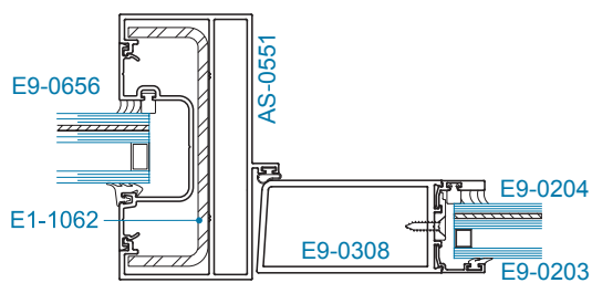
SECTION 3 OFFSET HUNG w/ OPTIONAL STEEL REINFORCEMENT
