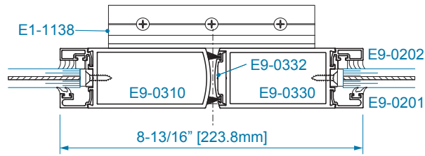
SECTION 1 MEETING STILES
