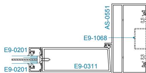
SECTION 5 OFFSET HUNG
