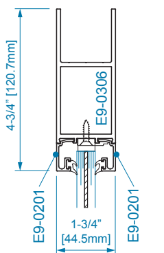
SECTION 1 9/16" DRY GLAZING
