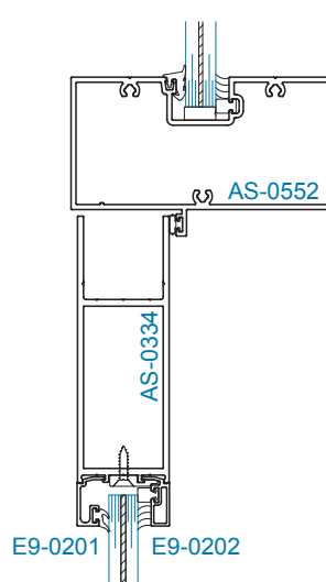
SECTION 4 OFFSET HUNG 9/16" DOOR GLAZING 9/16" TRANSOM GLAZING
