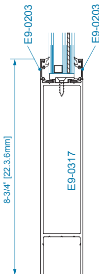
SECTION 2A 8" BOTTOM RAIL 1" DRY GLAZING
