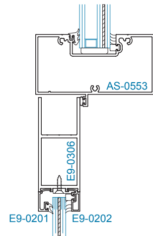
SECTION 4A OFFSET HUNG 9/16" DOOR GLAZING 1-5/16" TRANSOM GLAZING
