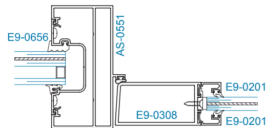
SECTION 3 OFFSET HUNG 1-5/16" GLAZING SIDELITE
