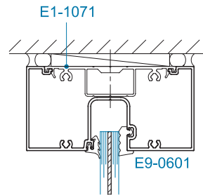
SECTION 2 9/16" GLAZING
