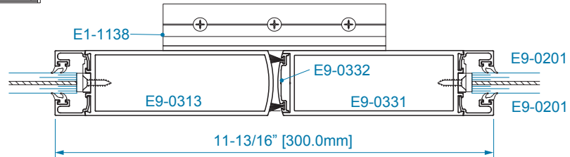
SECTION 1 MEETING STILES
