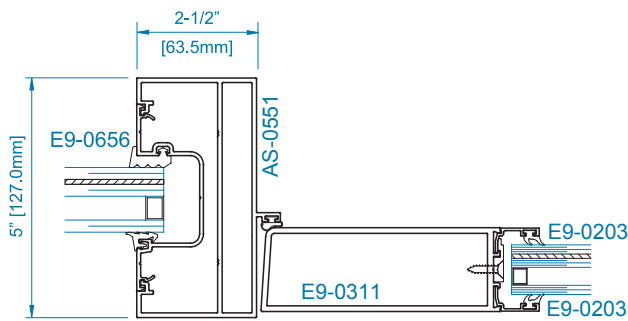
SECTION 2 OFFSET HUNG 1-5/16" GLAZING SIDELITE
