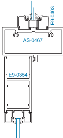
SECTION 15A OFFSET HUNG w/ SCREW SPLINES 1/4" GLAZING
