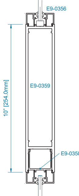
SECTION 4C 10" MID RAIL OPTION
