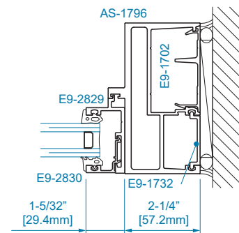
SECTION 17 1" GLAZING
