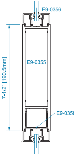
SECTION 4B 7-1/2" MID RAIL OPTION
