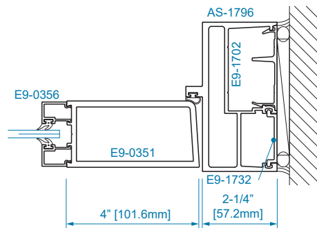
SECTION 13 1/4" GLAZING
