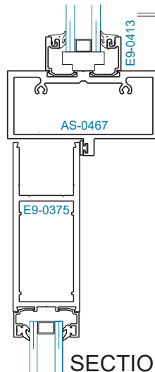
SECTION 26A 1" GLAZING
