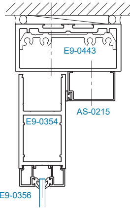
SECTION 11A OFFSET HUNG (OHCC)
