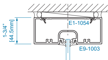
SECTION 24 1/4" GLAZING
