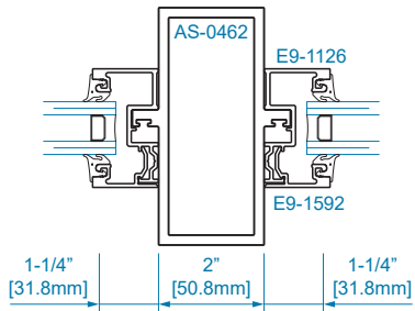
SECTION 18A 1" GLAZING
