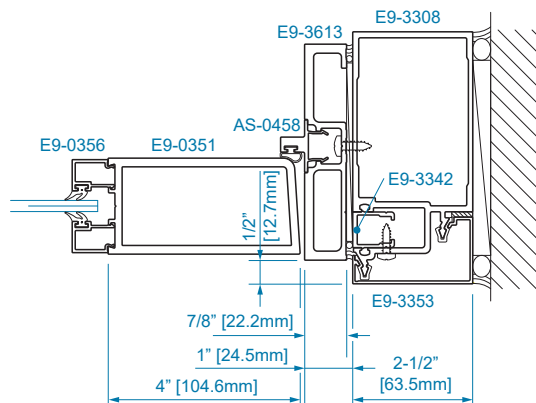
SECTION 13 1/4" GLAZING
