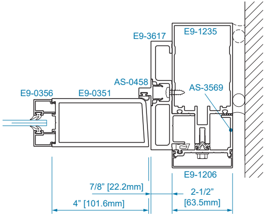
SECTION 13 1/4" GLAZING
