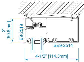
SECTION 24 1" GLAZING
