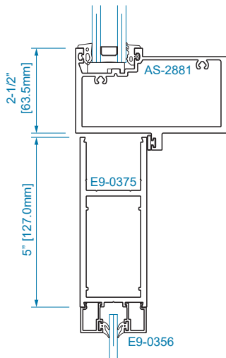
SECTION 25 OFFSET HUNG
