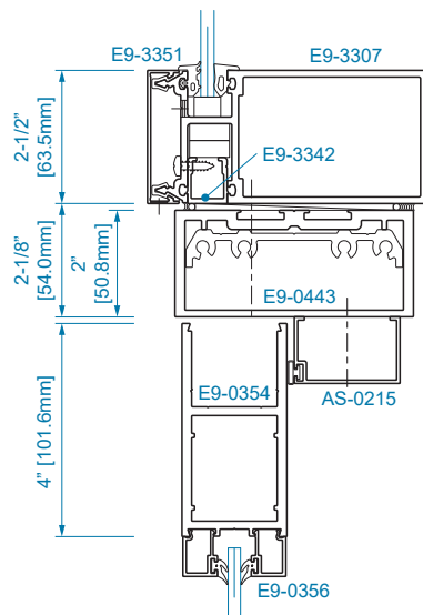
SECTION 11A OFFSET HUNG (OHCC)
