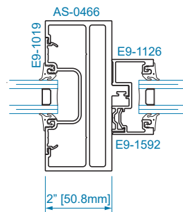
SECTION 26A 1" GLAZING
