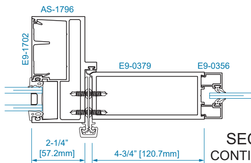
SECTION 22 1/4" GLAZING
