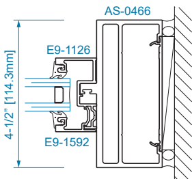
SECTION 17A 1" GLAZING
