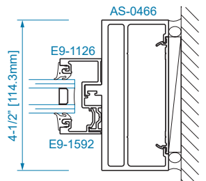
SECTION 17A 1" GLAZING
