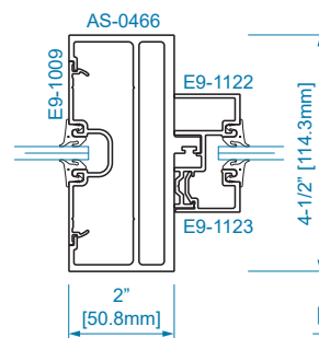
SECTION 16 1/4" GLAZING
