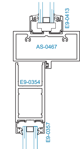
SECTION 15D OFFSET HUNG w/ SCREW SPLINES 1/4" GLAZING
