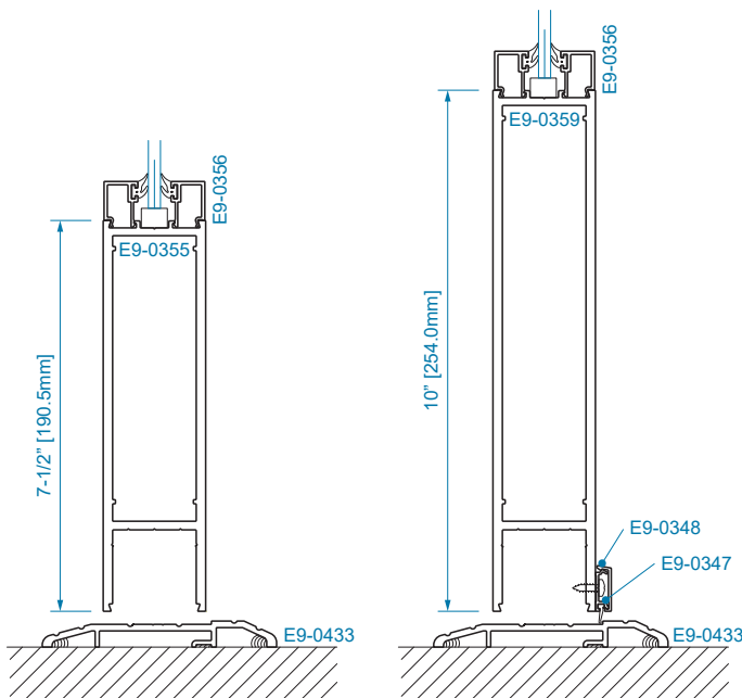
SECTION 2 7-1/2" BOTTOM RAIL
