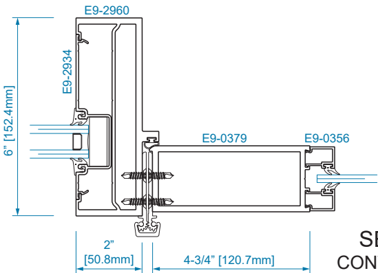
SECTION 22 1/4" GLAZING
