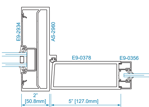
SECTION 22 1/4" GLAZING
