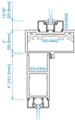
SECTION 15 OFFSET HUNG 1/4" GLAZING
