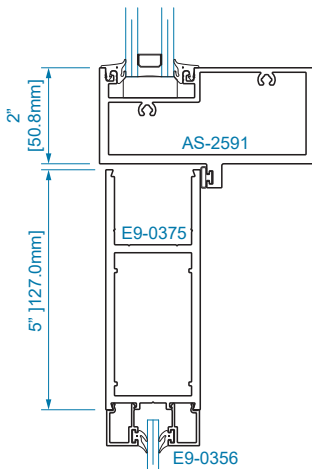
SECTION 25 OFFSET HUNG
