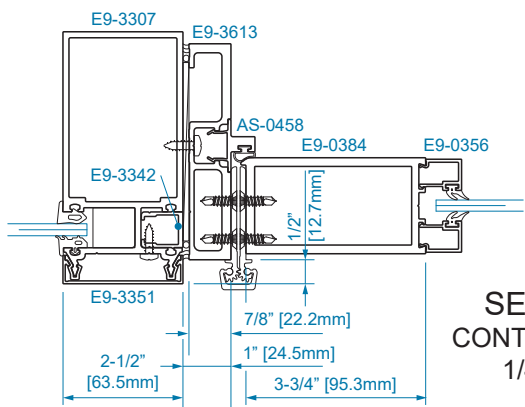
SECTION 12 1/4" GLAZING
