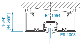
SECTION 14 1/4" GLAZING
