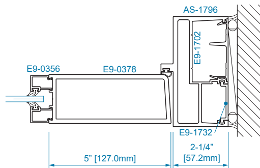
SECTION 23 1/4" GLAZING
