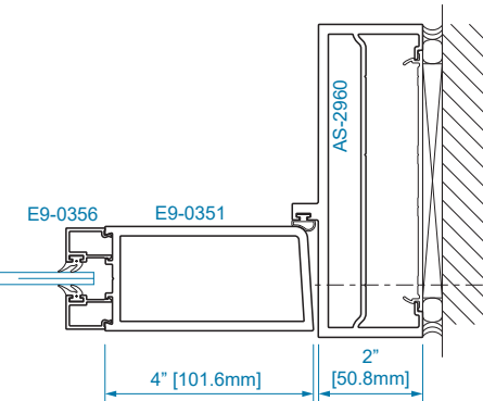
SECTION 13 1/4" GLAZING
