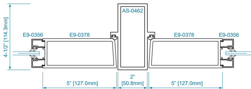
SECTION 29 INTERMEDIATE MULLION
