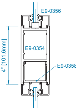
SECTION 4 4" MID RAIL OPTION
