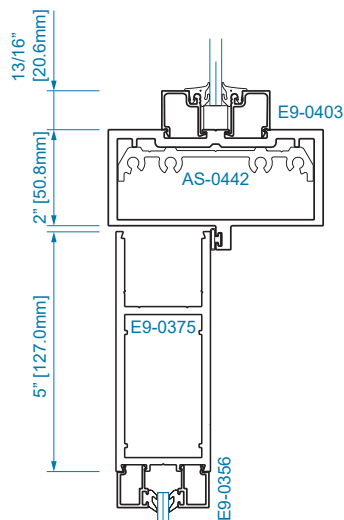
SECTION 25 OFFSET HUNG 1/4" GLAZING
