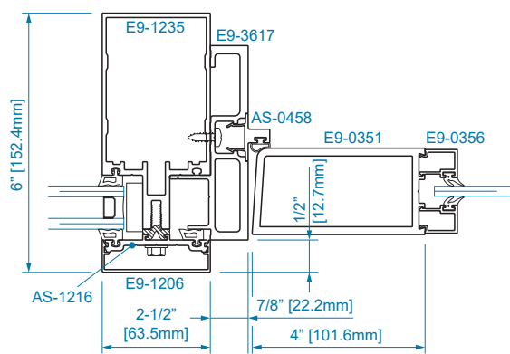
SECTION 12 1/4" GLAZING
