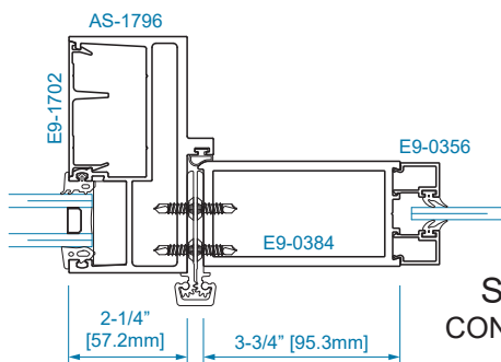
SECTION 12 1/4" GLAZING
