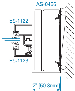
SECTION 27 1/4" GLAZING
