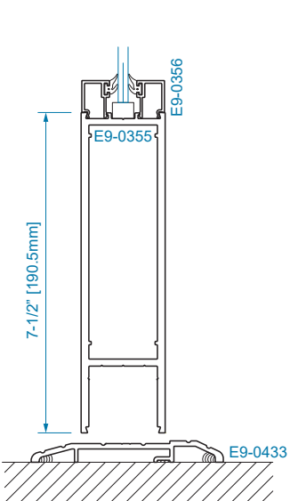
SECTION 2 7-1/2" BOTTOM RAIL
