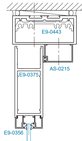
SECTION 21A OFFSET HUNG (OHCC)
