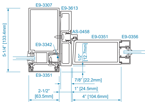
SECTION 12 1/4" GLAZING
