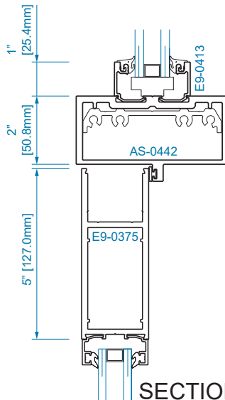
SECTION 24A 1/4" GLAZING
