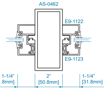
SECTION 18 1/4" GLAZING
