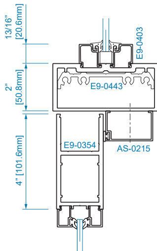
SECTION 15B OFFSET HUNG (OHCC) 1/4" GLAZING
