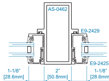
SECTION 28 1" GLAZING
