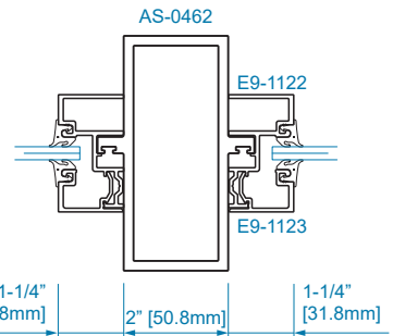
SECTION 28 1/4" GLAZING
