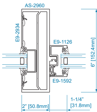
SECTION 26 1" GLAZING
