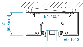
SECTION 24A 1/4" GLAZING
