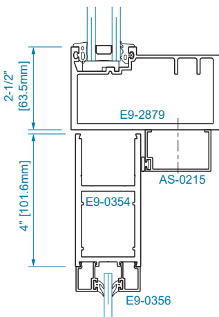
SECTION 15A OFFSET HUNG (OHCC)
