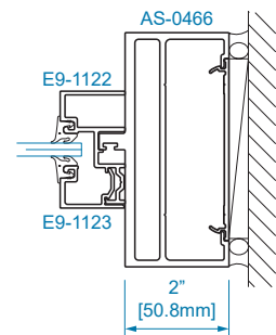
SECTION 17 1/4" GLAZING
