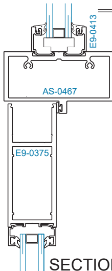
SECTION 25D OFFSET HUNG w/ SCREW SPLINES 1/4" GLAZING
