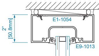
SECTION 14A 1" GLAZING
