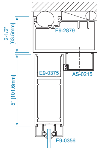
SECTION 21A OFFSET HUNG (OHCC)
