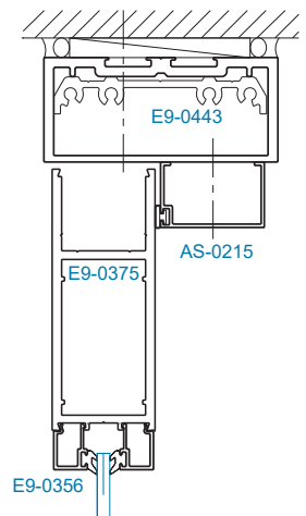
SECTION 21A OFFSET HUNG (OHCC)
