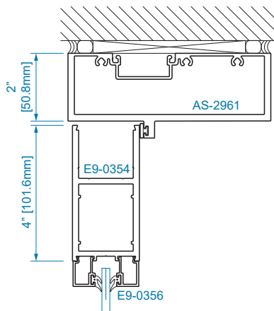
SECTION 11 OFFSET HUNG
