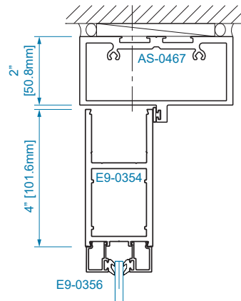
SECTION 11 OFFSET HUNG
