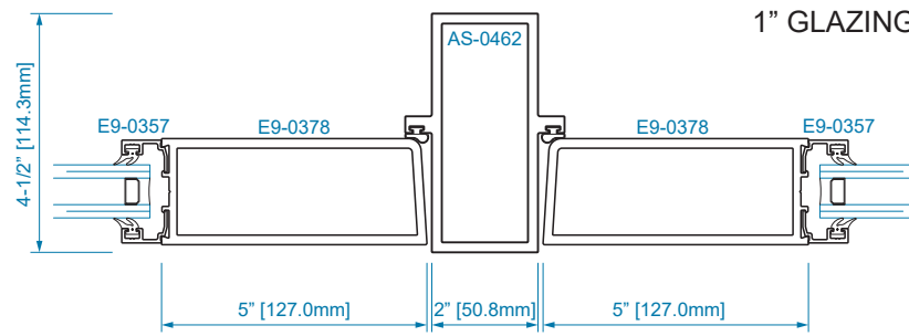
SECTION 29A 1" GLAZING
