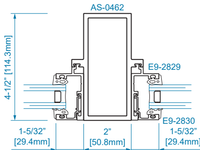
SECTION 18 1" GLAZING
