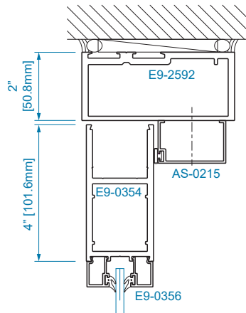
SECTION 11A OFFSET HUNG (OHCC)
