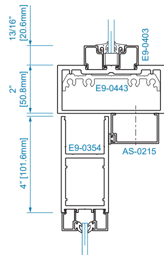
SECTION 15B OFFSET HUNG (OHCC) 1/4" GLAZING
