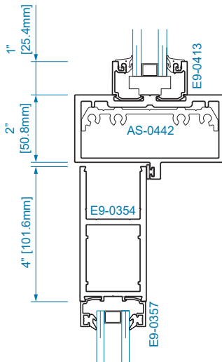
SECTION 15C OFFSET HUNG 1" GLAZING
