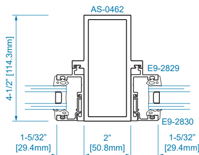
SECTION 28 1" GLAZING
