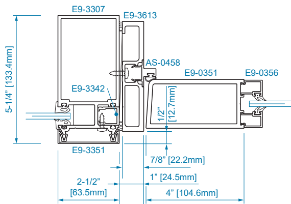
SECTION 12 1/4" GLAZING
