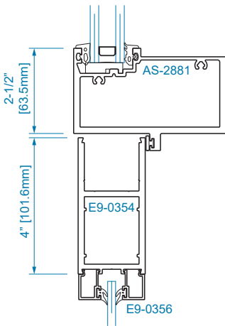
SECTION 15 OFFSET HUNG
