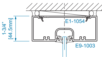
SECTION 24 1/4" GLAZING
