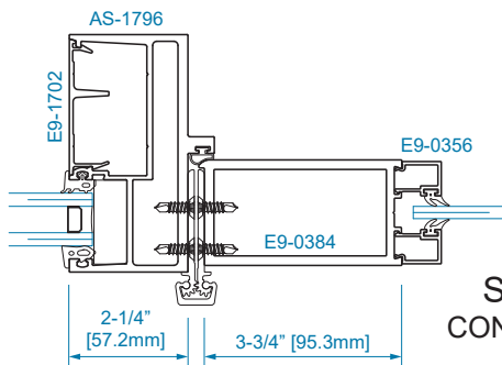
SECTION 12 1/4" GLAZING
