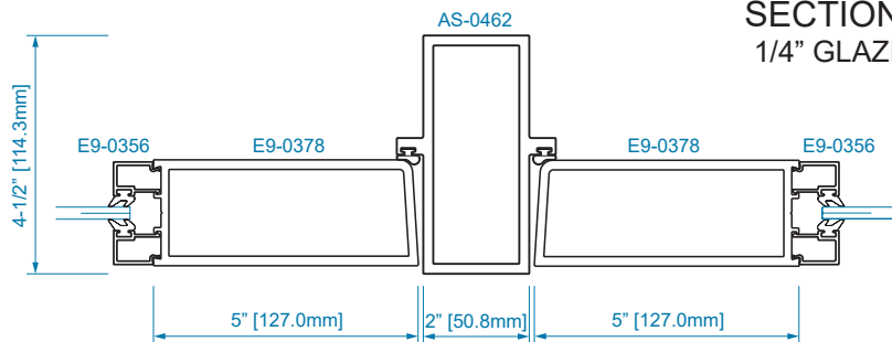
SECTION 29 INTERMEDIATE JAMB
