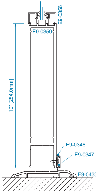
SECTION 2A 10" BOTTOM RAIL
