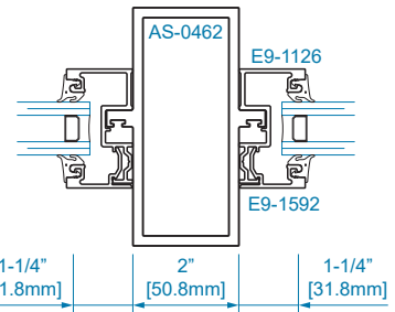
SECTION 18A 1" GLAZING
