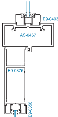
SECTION 25A OFFSET HUNG w/ SCREW SPLINES 1/4" GLAZING
