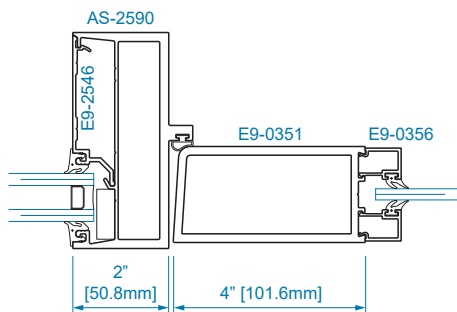
SECTION 12 1/4" GLAZING
