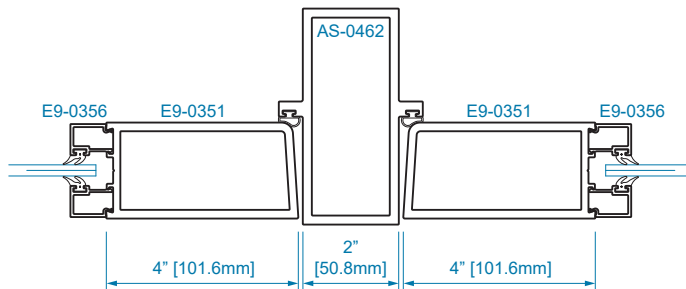
SECTION 19 INTERMEDIATE MULLION
