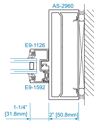
SECTION 27 1" GLAZING
