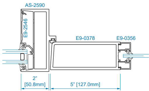
SECTION 22 1/4" GLAZING
