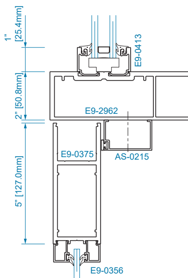
SECTION 25A OFFSET HUNG (OHCC)
