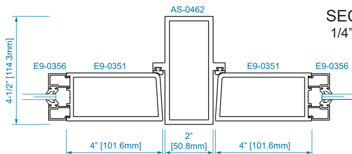
SECTION 19 INTERMEDIATE JAMB
