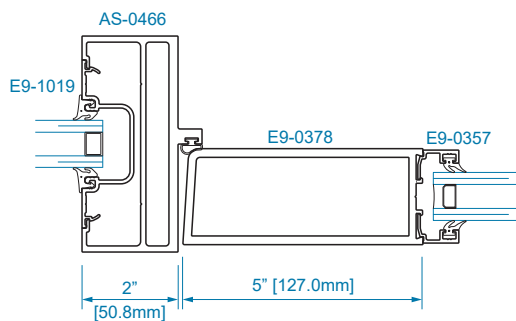
SECTION 22A OFFSET HUNG 1" GLAZING SIDELITE
