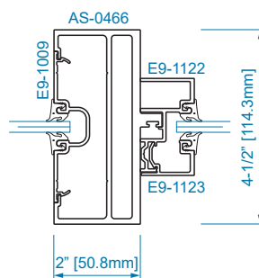
SECTION 26 1/4" GLAZING
