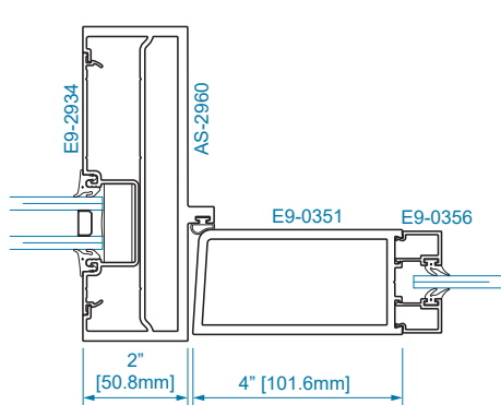
SECTION 12 1/4" GLAZING
