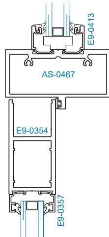
SECTION 15D OFFSET HUNG w/ SCREW SPLINES 1/4" GLAZING
