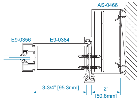
SECTION 13 CONTINUOUS HINGE AT JAMB
