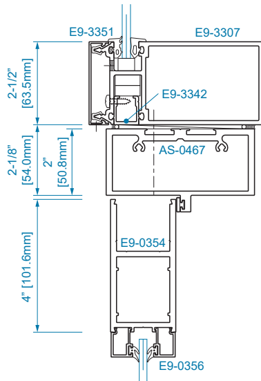
SECTION 11 OFFSET HUNG
