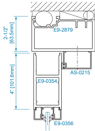
SECTION 11A OFFSET HUNG (OHCC)
