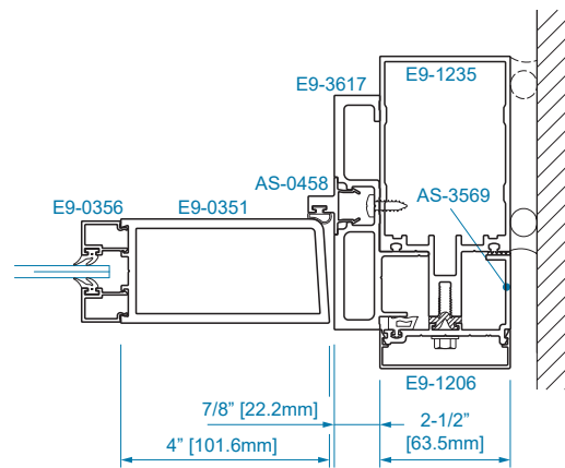
SECTION 13 1/4" GLAZING
