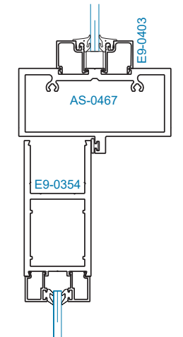
SECTION 15A OFFSET HUNG w/ SCREW SPLINES 1/4" GLAZING
