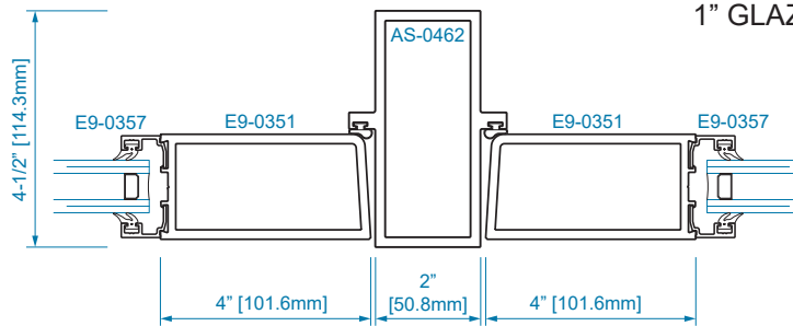
SECTION 19A 1" GLAZING
