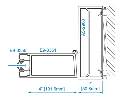
SECTION 13 1/4" GLAZING
