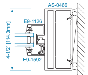
SECTION 17A 1" GLAZING
