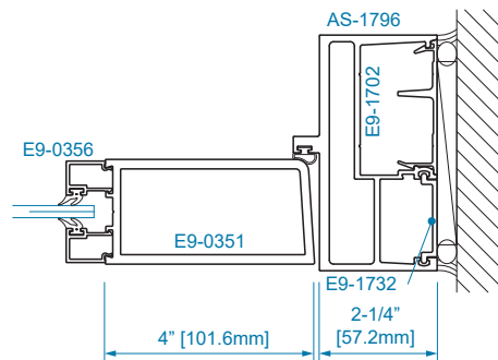
SECTION 13 1/4" GLAZING
