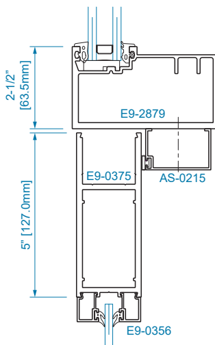
SECTION 25A OFFSET HUNG (OHCC)
