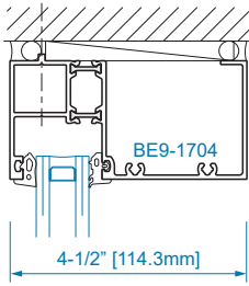
SECTION 14 1" GLAZING
