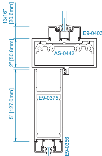
SECTION 25 OFFSET HUNG 1/4" GLAZING
