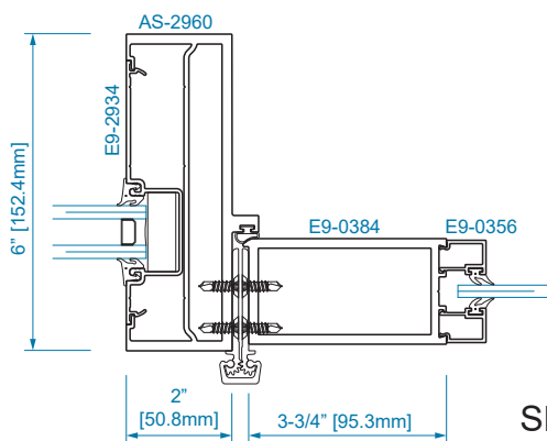
SECTION 12 1/4" GLAZING
