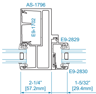
SECTION 26 1" GLAZING
