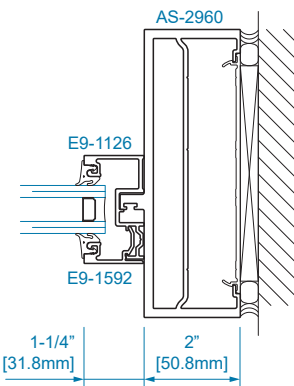
SECTION 17 1" GLAZING
