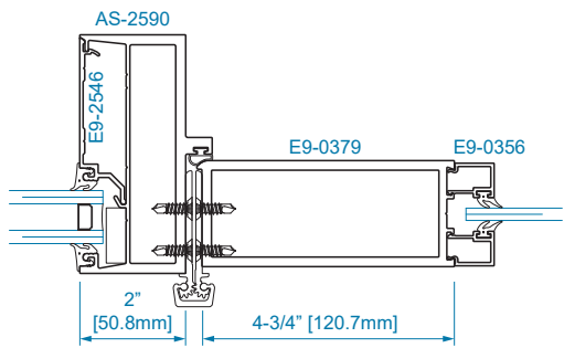
SECTION 22A CONTINUOUS HINGE 1/4" GLAZING
