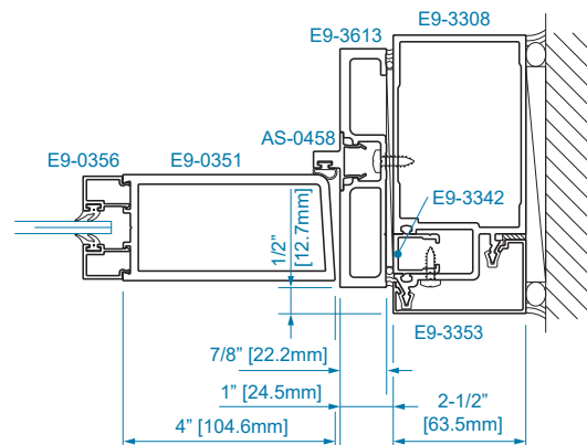
SECTION 13 1/4" GLAZING
