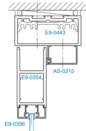
SECTION 11A OFFSET HUNG (OHCC)
