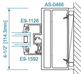
SECTION 17A 1" GLAZING
