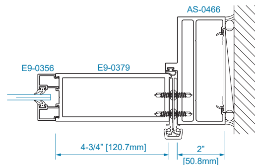
SECTION 23 CONTINUOUS HINGE AT JAMB
