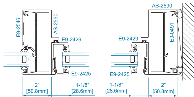
SECTION 27 1" GLAZING
