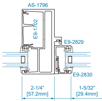
SECTION 16 1" GLAZING
