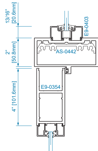
SECTION 15 OFFSET HUNG 1/4" GLAZING
