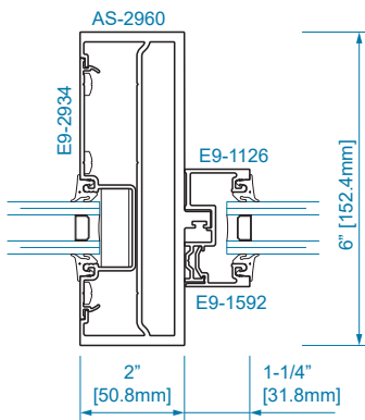
SECTION 16 1" GLAZING
