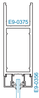
SECTION 6 5" TOP RAIL
