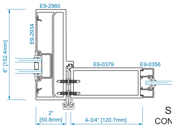
SECTION 22 1/4" GLAZING
