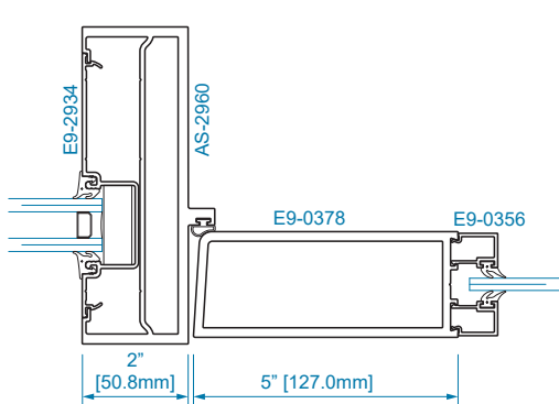
SECTION 22 1/4" GLAZING
