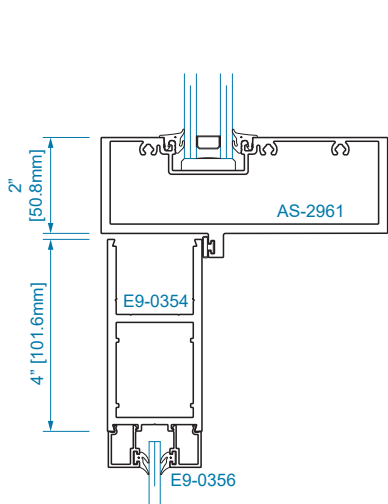
SECTION 15 OFFSET HUNG
