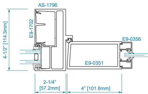
SECTION 12 1/4" GLAZING
