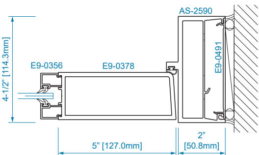
SECTION 23 1/4" GLAZING
