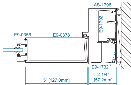
SECTION 23 1/4" GLAZING
