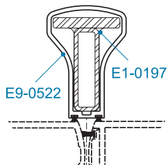
OPTIONAL REMOVABLE MULLION
