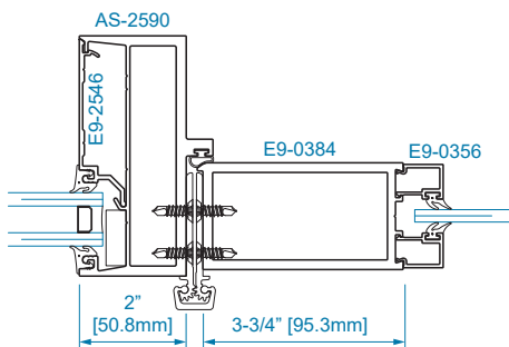
SECTION 12A CONTINUOUS HINGE 1/4" GLAZING
