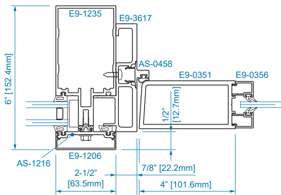
SECTION 12 1/4" GLAZING
