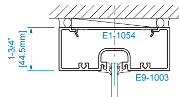
SECTION 14 1/4" GLAZING
