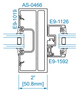
SECTION 16A 1" GLAZING
