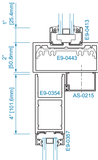
SECTION 15E OFFSET HUNG (OHCC) 1" GLAZING
