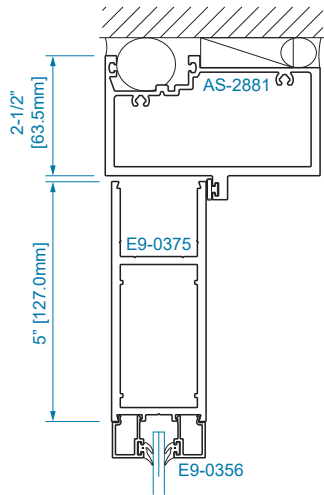
SECTION 21 OFFSET HUNG
