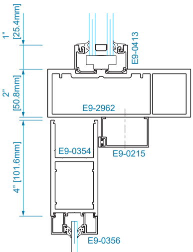
SECTION 15A OFFSET HUNG (OHCC)
