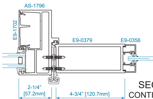
SECTION 22 1/4" GLAZING
