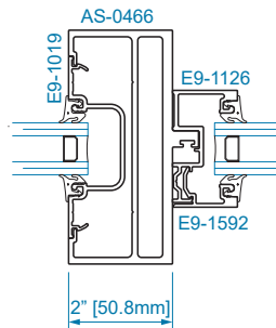
SECTION 26A 1" GLAZING
