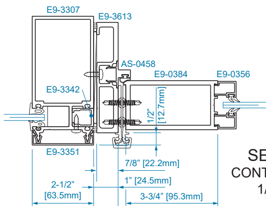
SECTION 12 1/4" GLAZING
