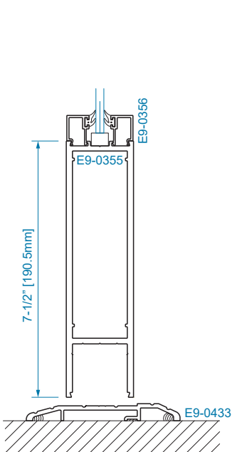
SECTION 2 7-1/2" BOTTOM RAIL
