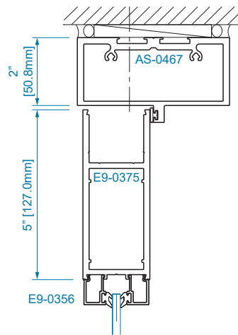
SECTION 21 OFFSET HUNG
