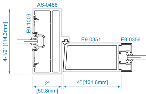
SECTION 12 OFFSET HUNG 1/4" GLAZING SIDELITE
