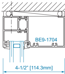
SECTION 24 1" GLAZING
