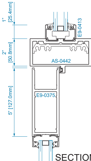
SECTION 25C OFFSET HUNG 1/4" GLAZING
