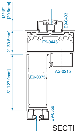
SECTION 25 OFFSET HUNG 1/4" GLAZING
