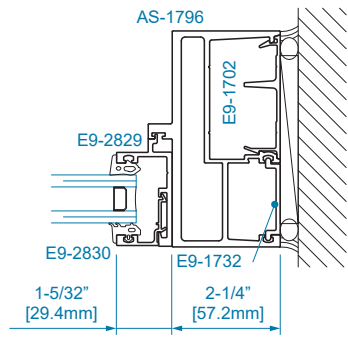
SECTION 17 1" GLAZING
