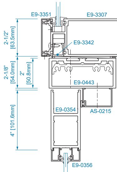
SECTION 11A OFFSET HUNG (OHCC)
