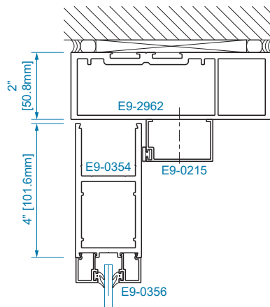
SECTION 11A OFFSET HUNG (OHCC)
