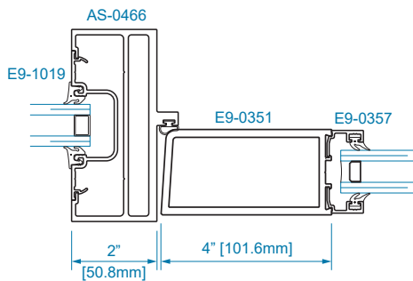
SECTION 12A OFFSET HUNG 1" GLAZING SIDELITE
