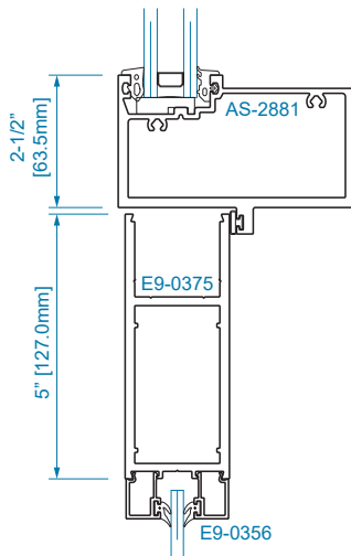
SECTION 25 OFFSET HUNG
