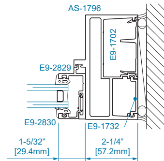
SECTION 27 1" GLAZING
