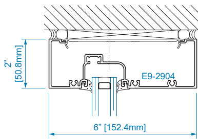
SECTION 14 1" GLAZING
