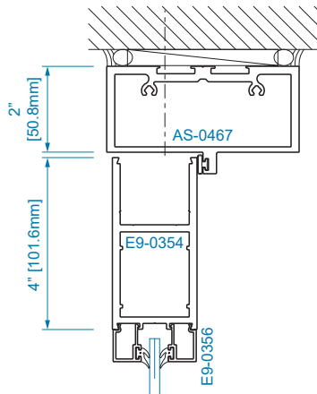
SECTION 11 OFFSET HUNG
