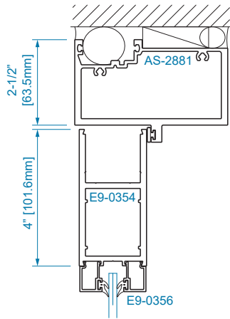
SECTION 11 OFFSET HUNG
