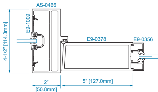
SECTION 22 OFFSET HUNG 1/4" GLAZING SIDELITE
