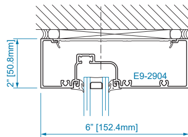
SECTION 24 1" GLAZING
