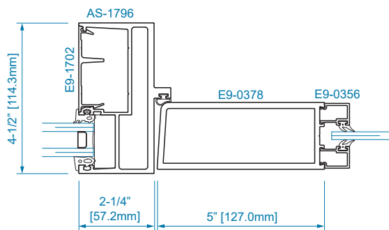
SECTION 22 1/4" GLAZING
