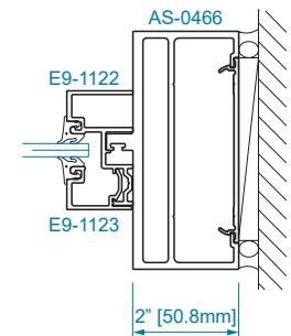
SECTION 27 1/4" GLAZING
