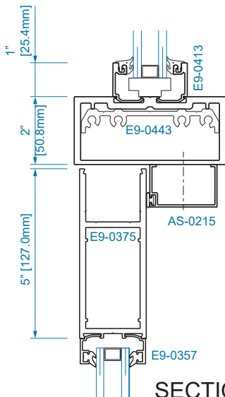
SECTION 25E OFFSET HUNG (OHCC) 1/4" GLAZING
