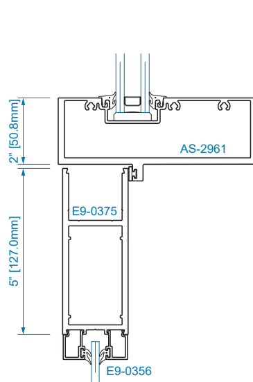
SECTION 25 OFFSET HUNG
