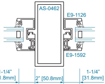
SECTION 28A 1" GLAZING
