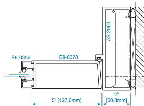
SECTION 23 1/4" GLAZING
