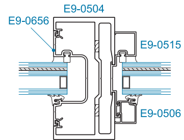
SECTION 1 1-5/16" GLAZING
