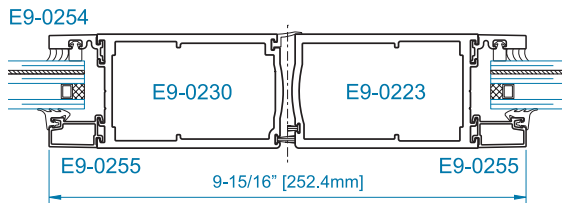
SECTION 1 WATER RESISTANT MEETING STILE
