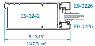
SECTION 5A CONTINUOUS HINGE
