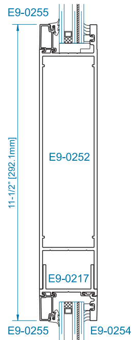
SECTION 4 11-1/2" MID RAIL OPTION*
