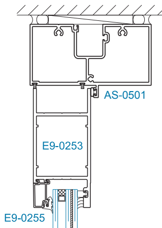
SECTION 3 OFFSET HUNG*
