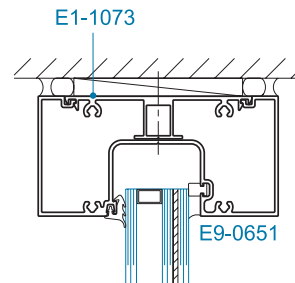
SECTION 2 1-5/16" GLAZING
