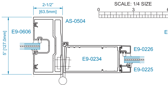
SECTION 2 OFFSET HUNG* 9/16" GLAZING SIDELITE
