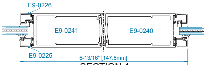
SECTION 1 WATER RESISTANT MEETING STILE
