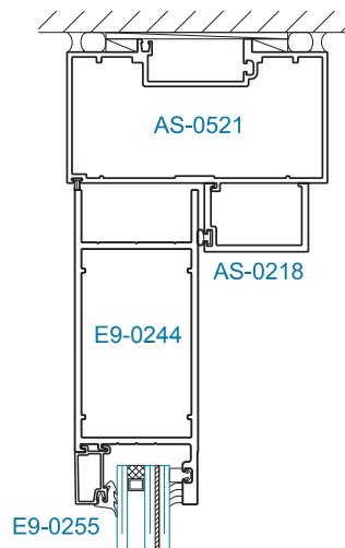
SECTION 4 OFFSET HUNG* (OHCC) 1" DOOR GLAZING
