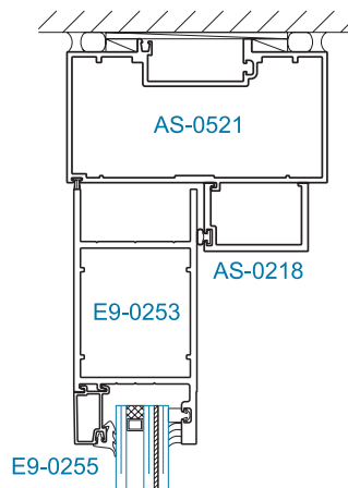
SECTION 4 OFFSET HUNG* (OHCC) 1" DOOR GLAZING
