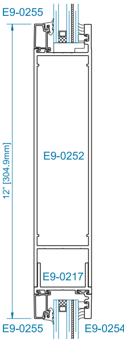
SECTION 4 12" MID RAIL OPTION*
