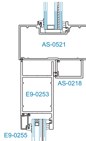
SECTION 5 OFFSET HUNG* (OHCC) 1" DOOR GLAZING 1-5/16" TRANSOM GLAZING
