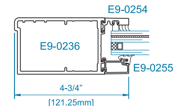
SECTION 3A CONTINUOUS HINGE
