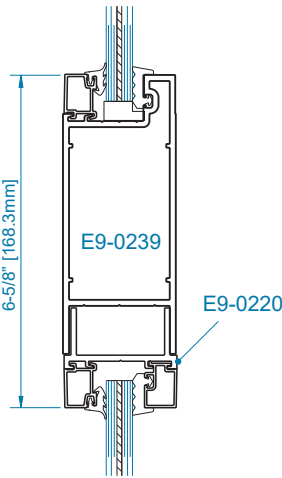
SECTION 3 6-5/8" MID RAIL W/ DRY GLAZE OPTION*
