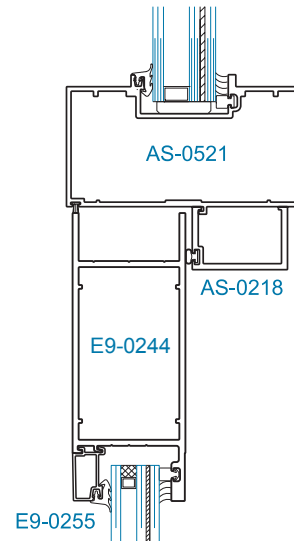
SECTION 5 OFFSET HUNG* (OHCC) 1" DOOR GLAZING 1-5/16" TRANSOM GLAZING
