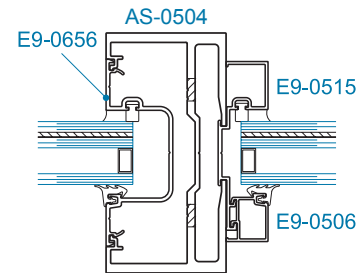
SECTION 2 1-5/16" GLAZING
