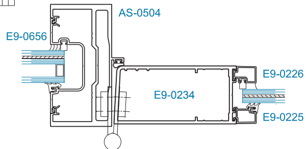
SECTION 3 OFFSET HUNG* 1-5/16" GLAZING SIDELITE
