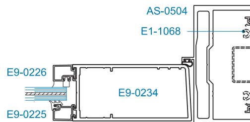
SECTION 5 OFFSET HUNG*
