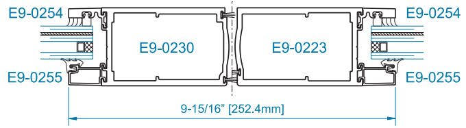
SECTION 1A AIR ONLY MEETING STILE
