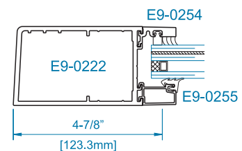
SECTION 3 OFFSET HUNG
