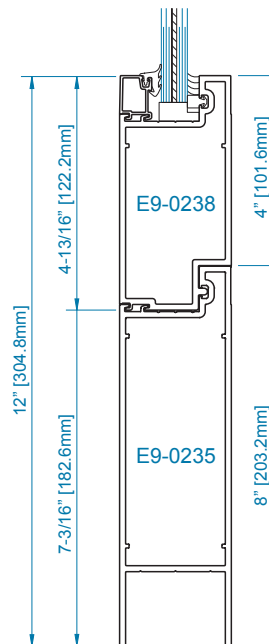
SECTION 4 OPTIONAL 12" STACKED BOTTOM RAIL
