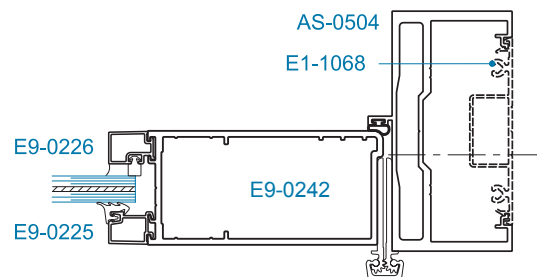
SECTION 7 CONTINUOUS HINGE
