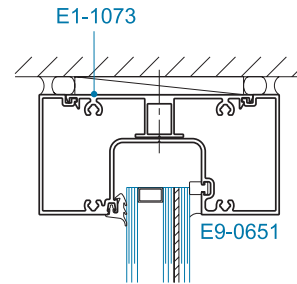
SECTION 1 1-5/16" GLAZING
