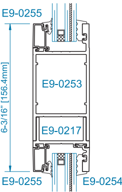
SECTION 1A 6" MID RAIL WITH DRY GLAZE OPTION*
