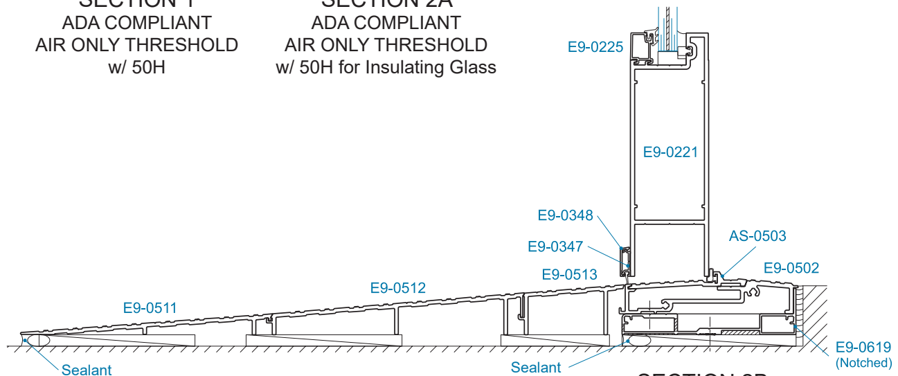
SECTION 2B WATER RESISTANT THRESHOLD w/ ADA EXTERIOR RAMP
