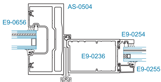
SECTION 5 CONTINUOUS HINGE
