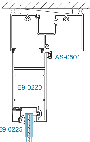
SECTION 3 OFFSET HUNG*
