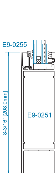
SECTION 2 8" BOTTOM RAIL *
