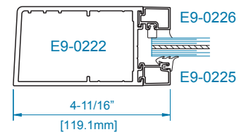
SECTION 5 OFFSET HUNG
