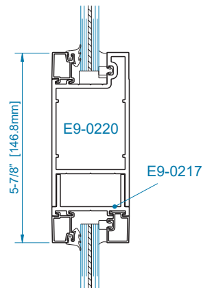
SECTION 3 5-3/4" MID RAIL W/ WET GLAZE OPTION*
