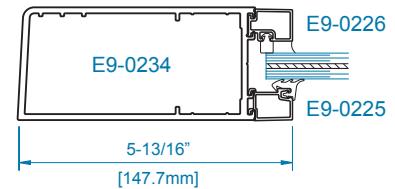
SECTION 5 OFFSET HUNG
