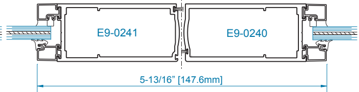
SECTION 1A AIR ONLY MEETING STILE
