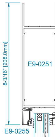
SECTION 1A 8" TOP RAIL *
