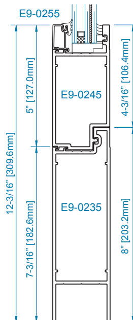
SECTION 2B OPTIONAL 12" STACKED BOTTOM RAIL
