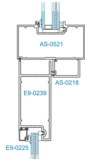
SECTION 4A OFFSET HUNG* (OHCC) 9/16" DOOR GLAZING 1-5/16" TRANSOM GLAZING
