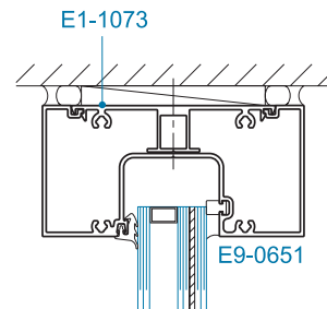
SECTION 2A 1-5/16" GLAZING
