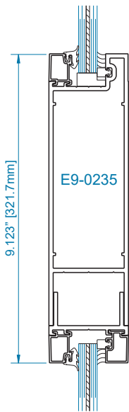
SECTION 2 9-1/8" MID RAIL *
