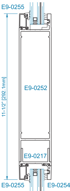
SECTION 4 11-1/2" MID RAIL OPTION*
