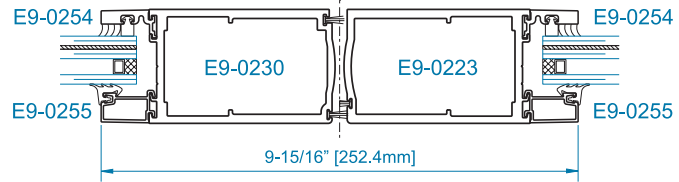
SECTION 1A AIR ONLY MEETING STILE
