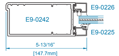
SECTION 5A CONTINUOUS HINGE
