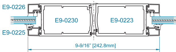
SECTION 1 WATER RESISTANT MEETING STILE
