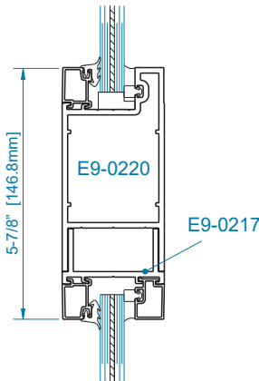
SECTION 3 5-3/4" MID RAIL W/ WET GLAZE OPTION*
