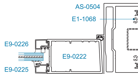
SECTION 5 OFFSET HUNG*
