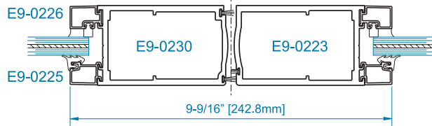
SECTION 1A AIR ONLY MEETING STILE
