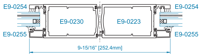
SECTION 1A AIR ONLY MEETING STILE
