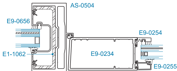
SECTION 3 OFFSET HUNG* w/ Optional Steel Reinforcement
