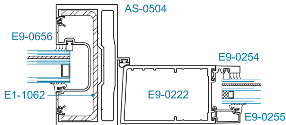
SECTION 3 OFFSET HUNG* w/ Optional Steel Reinforcement
