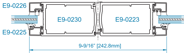
SECTION 1 WATER RESISTANT MEETING STILE
