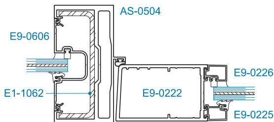
SECTION 4 OFFSET HUNG* w/ Optional Steel Reinforcement
