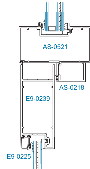
SECTION 4A OFFSET HUNG* (OHCC) 9/16" DOOR GLAZING 1-5/16" TRANSOM GLAZING
