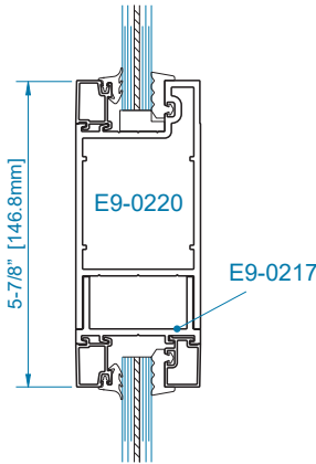
SECTION 3A 5-3/4" MID RAIL W/ DRY GLAZE OPTION*
