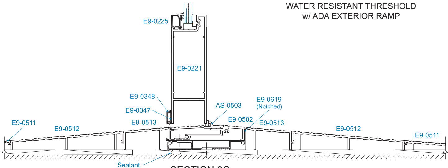
SECTION 2C WATER RESISTANT THRESHOLD w/ ADA EXTERIOR/INTERIOR RAMP
