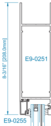
SECTION 1A 8" TOP RAIL *
