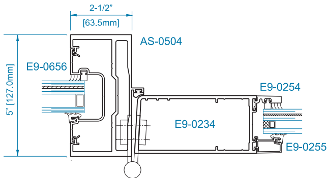
SECTION 1 WATER RESISTANT MEETING STILE
