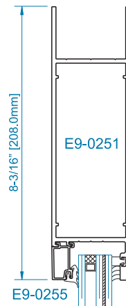
SECTION 1B 8" TOP RAIL*
