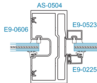
SECTION 1A 9/16" GLAZING (OHCC ONLY)
