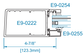
SECTION 3 OFFSET HUNG
