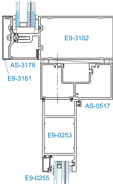
SECTION 1 YHC 300 OG W/ YHS 50 TU OFFSET HUNG* 1-5/16" GLAZING 1" GLAZING DOOR
