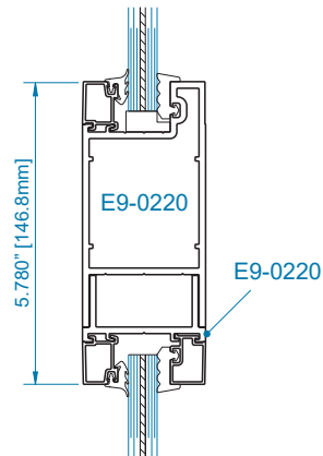
SECTION 3A 5-3/4" MID RAIL W/ DRY GLAZE OPTION*
