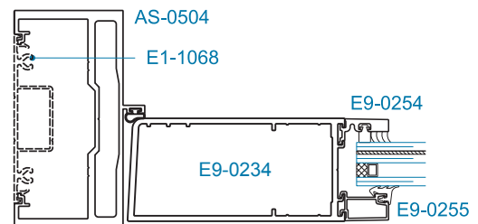
SECTION 4 OFFSET HUNG*
