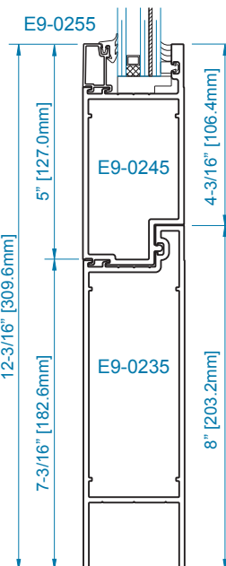
SECTION 2B OPTIONAL 12" STACKED BOTTOM RAIL
