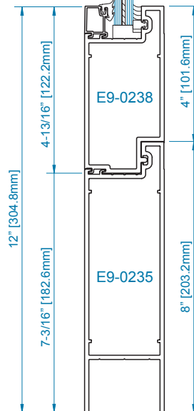
SECTION 5 OFFSET HUNG
