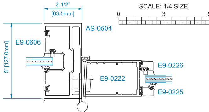
SECTION 2 OFFSET HUNG* 9/16" GLAZING SIDELITE
