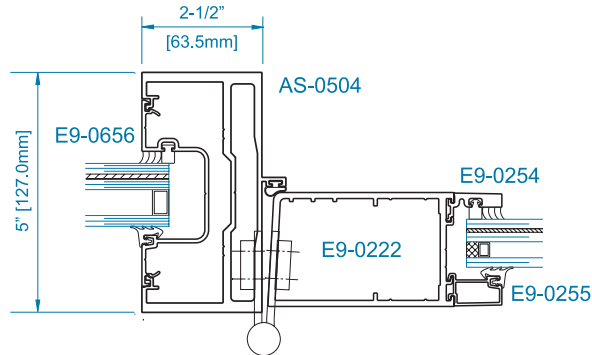
SECTION 1 WATER RESISTANT MEETING STILE
