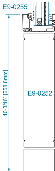
SECTION 2A 10" BOTTOM RAIL *
