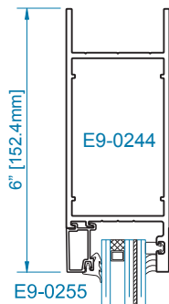
SECTION 1A 5" TOP RAIL*
