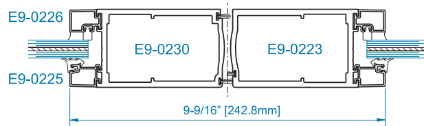
SECTION 1A AIR ONLY MEETING STILE
