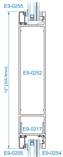
SECTION 4 12" MID RAIL OPTION*
