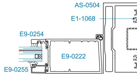
SECTION 4 OFFSET HUNG*
