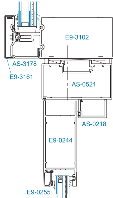
SECTION 2 YHC 300 OG W/ YHS 50 TU OFFSET HUNG (OHCC) 1" DOOR GLAZING 1-5/16" TRANSOM GLAZING
