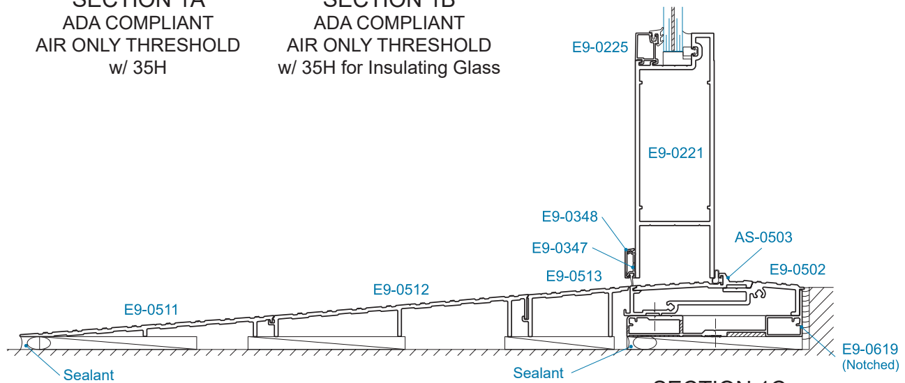
SECTION 1C WATER RESISTANT THRESHOLD w/ ADA EXTERIOR RAMP
