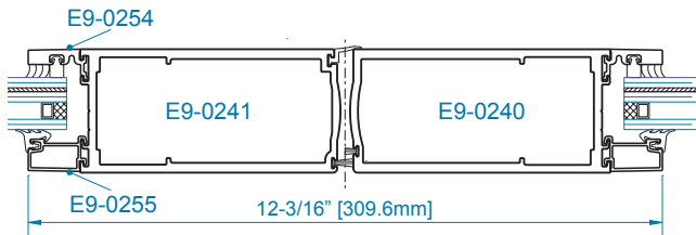
SECTION 1 WATER RESISTANT MEETING STILE
