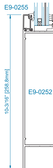
SECTION 2B 10" BOTTOM RAIL*
