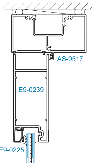
SECTION 3A OFFSET HUNG*
