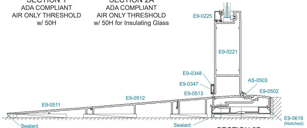
SECTION 2B WATER RESISTANT THRESHOLD w/ ADA EXTERIOR RAMP
