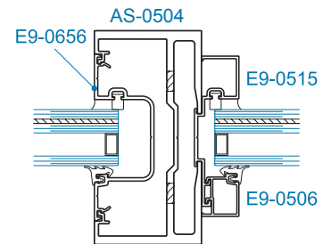
SECTION 1B 1-5/16" GLAZING
