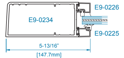
SECTION 5 OFFSET HUNG
