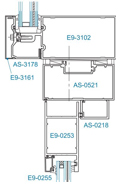
SECTION 2 YHC 300 OG W/ YHS 50 TU OFFSET HUNG* (OHCC) 1-5/16" GLAZING 1" GLAZING DOOR
