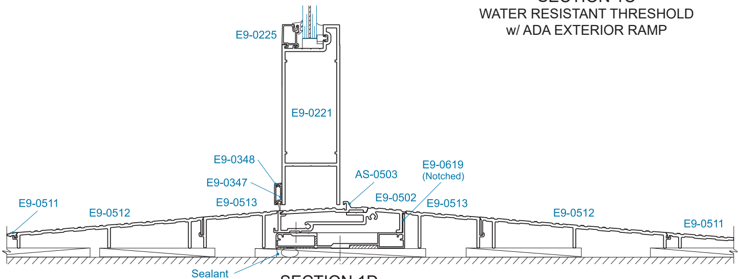
SECTION 1D WATER RESISTANT THRESHOLD w/ ADA EXTERIOR/INTERIOR RAMP
