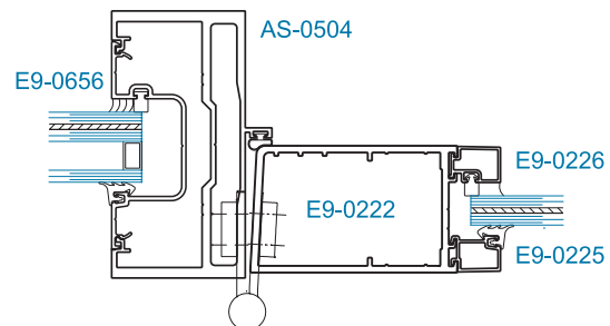
SECTION 3 OFFSET HUNG* 1-5/16" GLAZING SIDELITE
