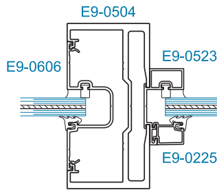
SECTION 1A 9/16" GLAZING (OHCC ONLY)
