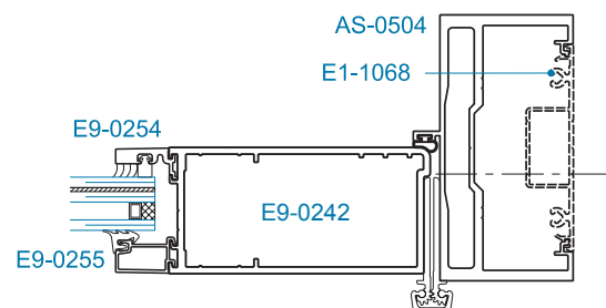
SECTION 6 CONTINUOUS HINGE
