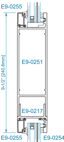
SECTION 2 9-1/2" MID RAIL OPTION*
