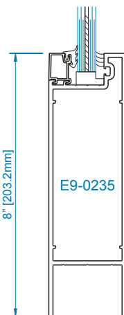
SECTION 3 8" BOTTOM RAIL
