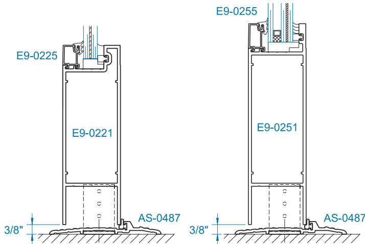
SECTION 1 ADA COMPLIANT AIR ONLY THRESHOLD w/ 50H
