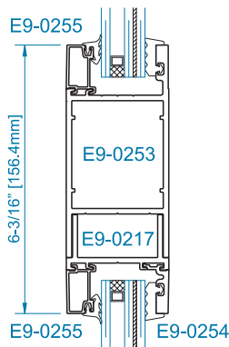
SECTION 1A 6" MID RAIL WITH DRY GLAZE OPTION*
