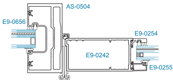
SECTION 5 CONTINUOUS HINGE
