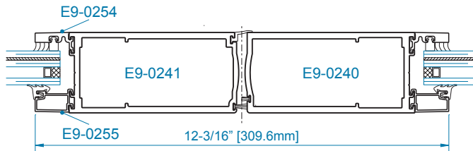
SECTION 1 WATER RESISTANT MEETING STILE
