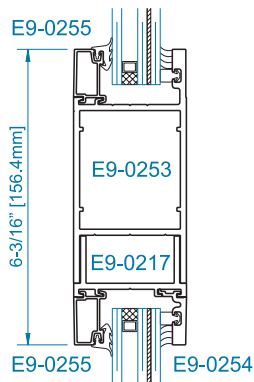
SECTION 1 6" MID RAIL OPTION*
