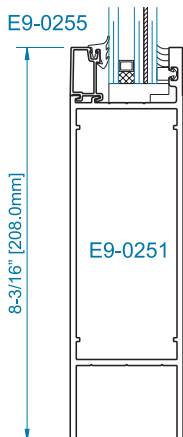
SECTION 2 8" BOTTOM RAIL*
