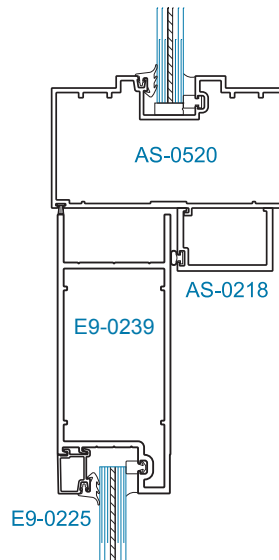
SECTION 4 OFFSET HUNG* (OHCC) 9/16" DOOR GLAZING 9/16" TRANSOM GLAZING
