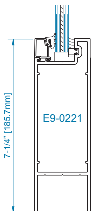
SECTION 2 7-1/4" BOTTOM RAIL
