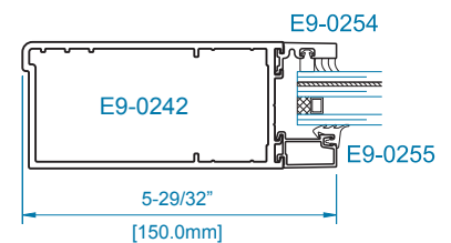
SECTION 3A CONTINUOUS HINGE
