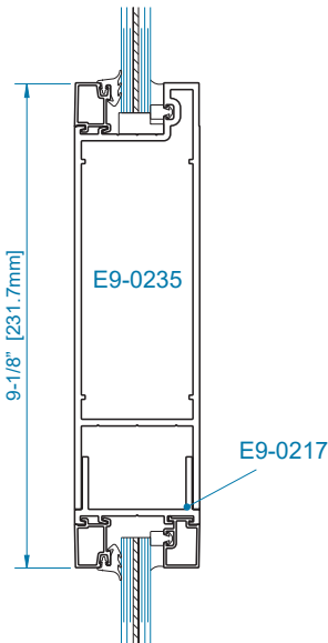
SECTION 2 9-1/8" MID RAIL *
