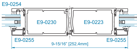
SECTION 1 WATER RESISTANT MEETING STILE
