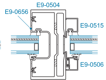
SECTION 1B 1-5/16" GLAZING
