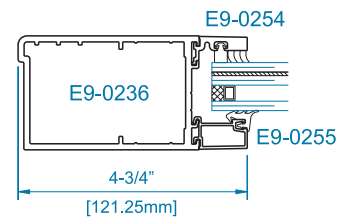
SECTION 3A CONTINUOUS HINGE
