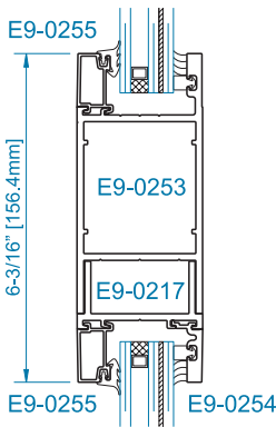
SECTION 1 6" MID RAIL OPTION*
