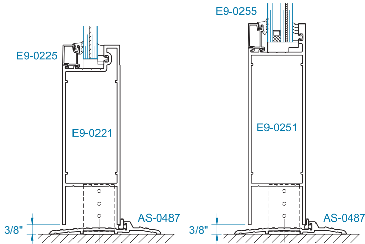
SECTION 1A ADA COMPLIANT AIR ONLY THRESHOLD w/ 35H
