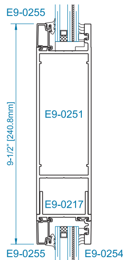
SECTION 2 9-1/2" MID RAIL OPTION*
