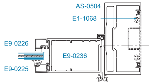
SECTION 7 CONTINUOUS HINGE
