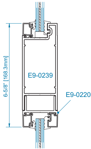
SECTION 3 6-5/8" MID RAIL W/ DRY GLAZE OPTION*
