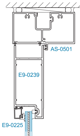
SECTION 3 OFFSET HUNG*
