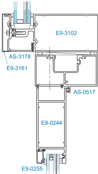
SECTION 1 YHC 300 OG W/ YHS 50 TU OFFSET HUNG 1" DOOR GLAZING 1-5/16" TRANSOM GLAZING
