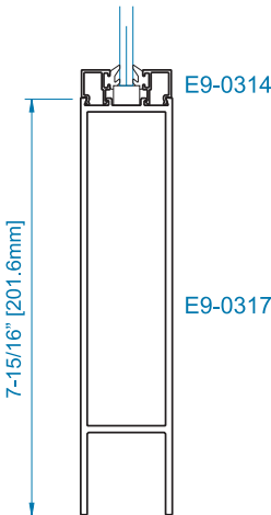
SECTION 2 8" BOTTOM RAIL *
