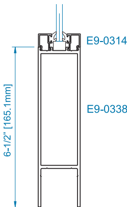
SECTION 2 6-1/2" BOTTOM RAIL *
