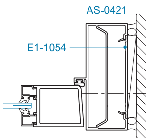
SECTION 4 OFFSET HUNG
