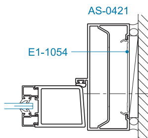
SECTION 4 OFFSET HUNG
