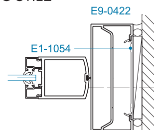
SECTION 4 CENTER HUNG
