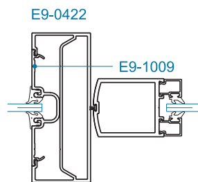
SECTION 3 CENTER HUNG
