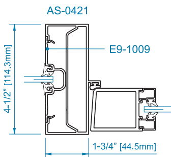
SECTION 3 OFFSET HUNG
