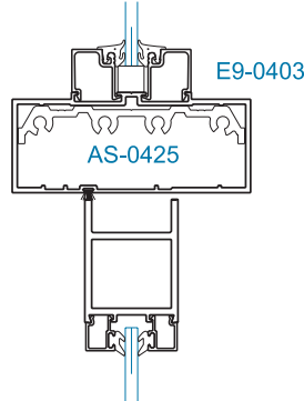
SECTION 6 CENTER HUNG
