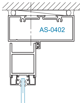
SECTION 1 OFFSET HUNG
