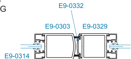
SECTION 8 MEETING STILE
