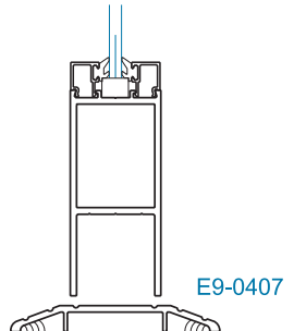
SECTION 2 OFFSET HUNG
