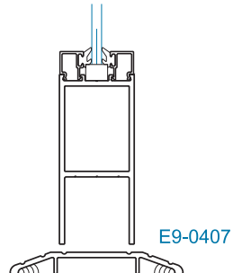
SECTION 2 OFFSET HUNG (OHCC)
