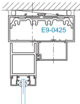
SECTION 1 OFFSET HUNG (OHCC)
