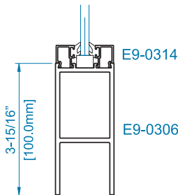
SECTION 2 4" BOTTOM RAIL *
