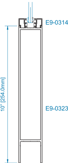
SECTION 2 10" BOTTOM RAIL *
