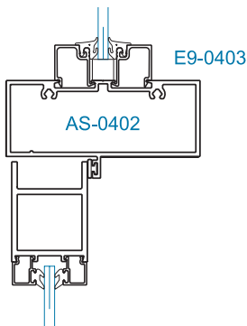
SECTION 6 OFFSET HUNG
