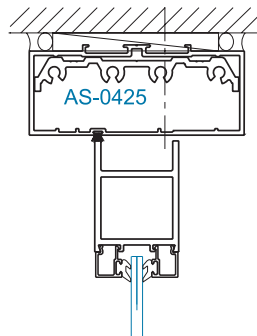
SECTION 1 CENTER HUNG
