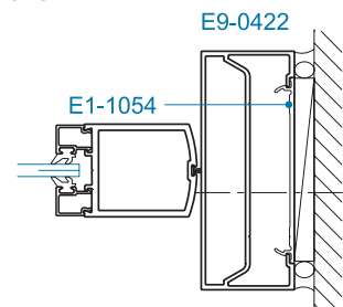
SECTION 4 CENTER HUNG
