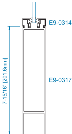
SECTION 2 8" BOTTOM RAIL*
