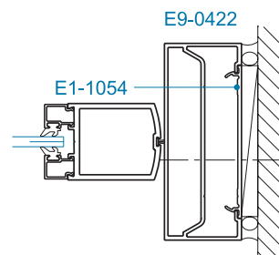
SECTION 4 CENTER HUNG
