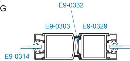
SECTION 8 MEETING STILE
