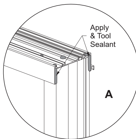
Lock Jamb Shown Fixed Jamb Similar
