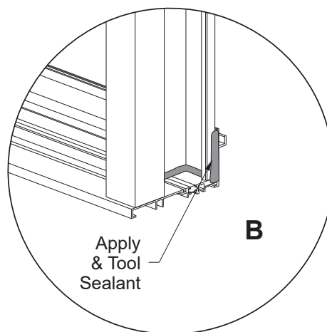
Lock Jamb Shown Fixed Jamb Similar
