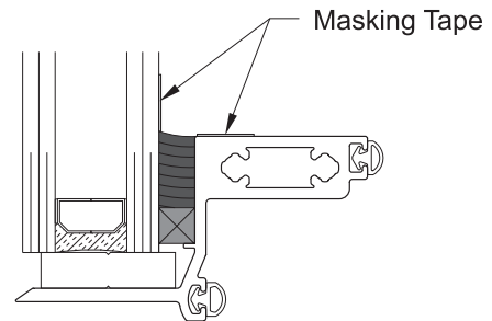
DETAIL 8
