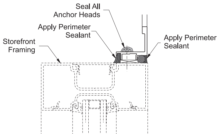
DETAIL 10
