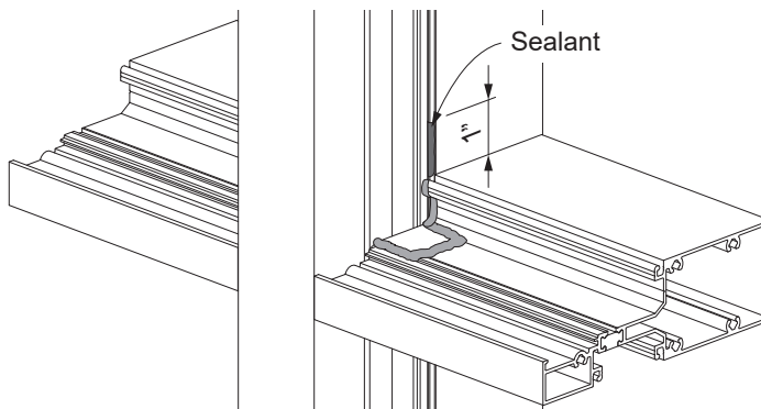
Detail 45
