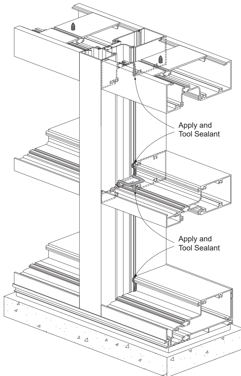
Detail 44
