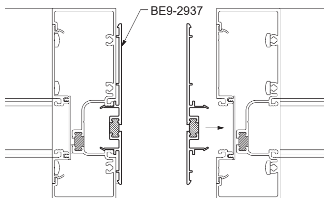
Detail 34
