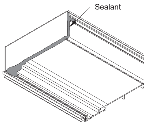
Detail 16
