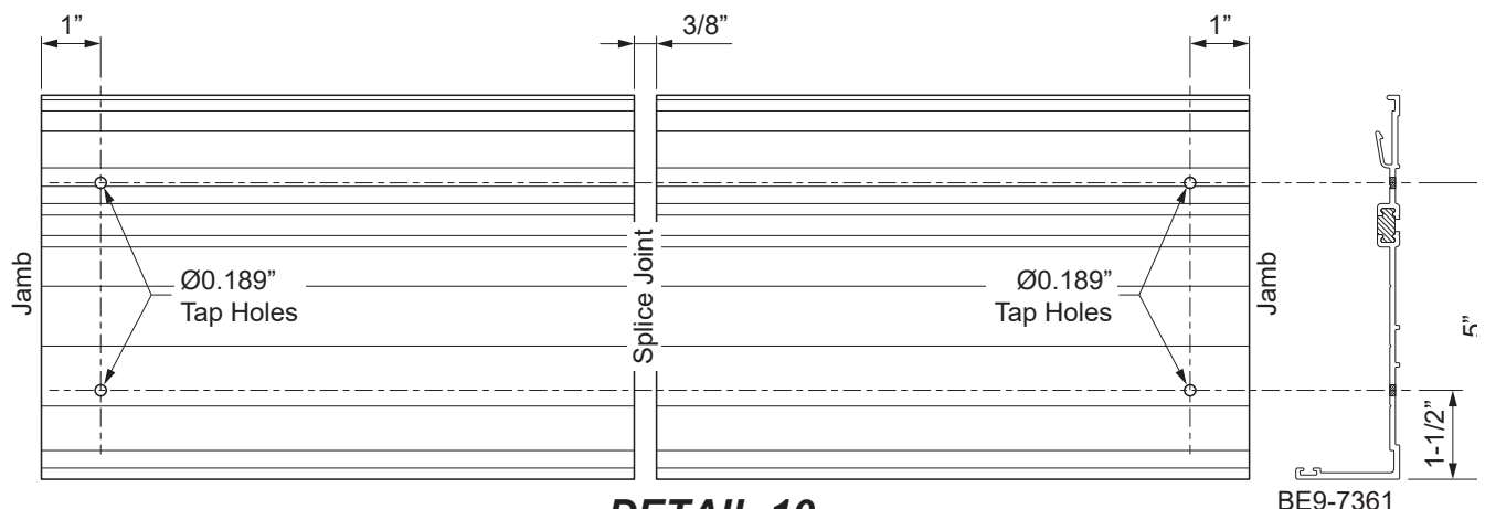
DETAIL 10
