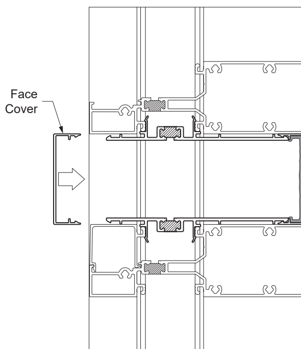
Detail 52
