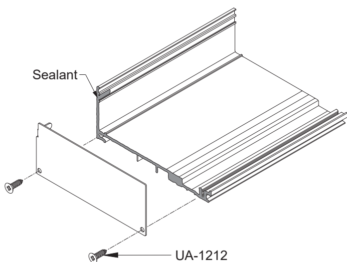
Detail 15
