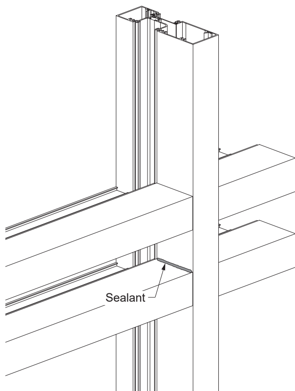
Detail 46
