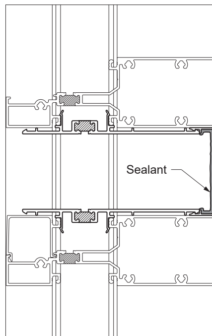
Detail 51
