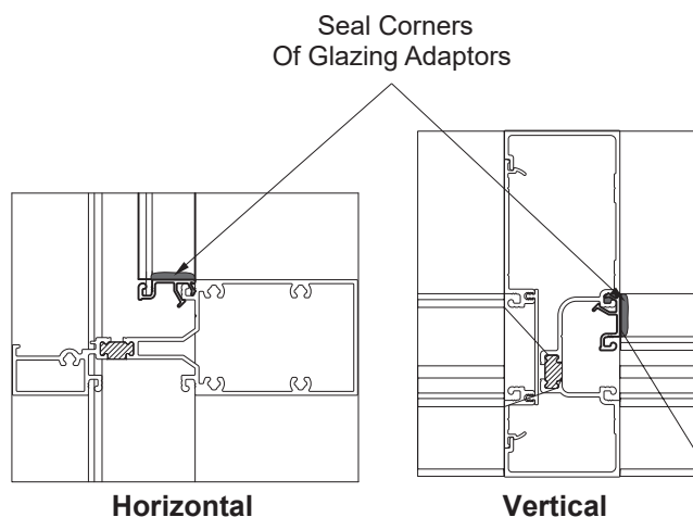
Detail 45A
