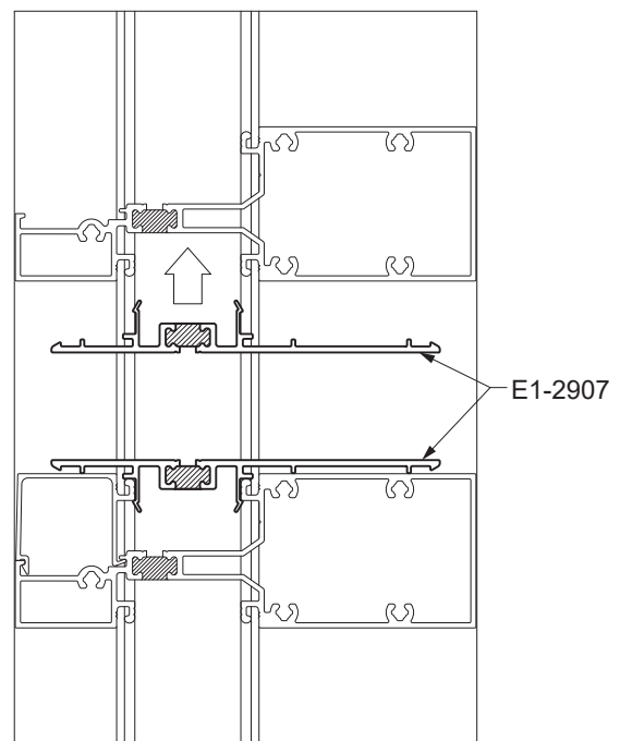
Detail 49
