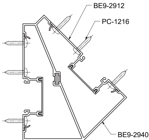
135° Outside Corner
