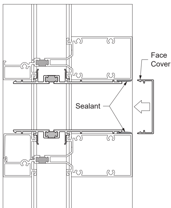
Detail 50
