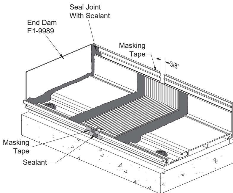
Detail 19
