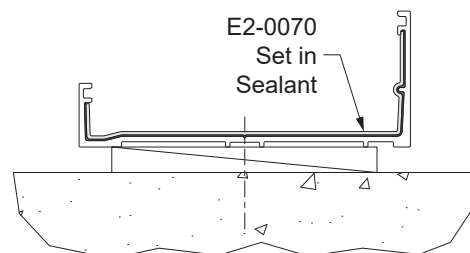
Detail 13A Sill Shown Head Similar
