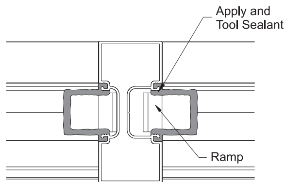
Detail 25 1" Glazing Shown 1/4" Glazing Similar
