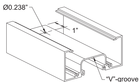
YES 45 FI Head Shown Others Similar
