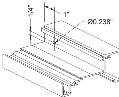
YES 45 FI Horizontal/Sill
